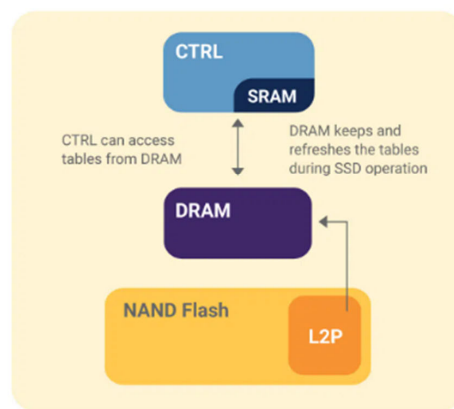
Figure 2. Cache operating mechanism of SSD with DRAM
