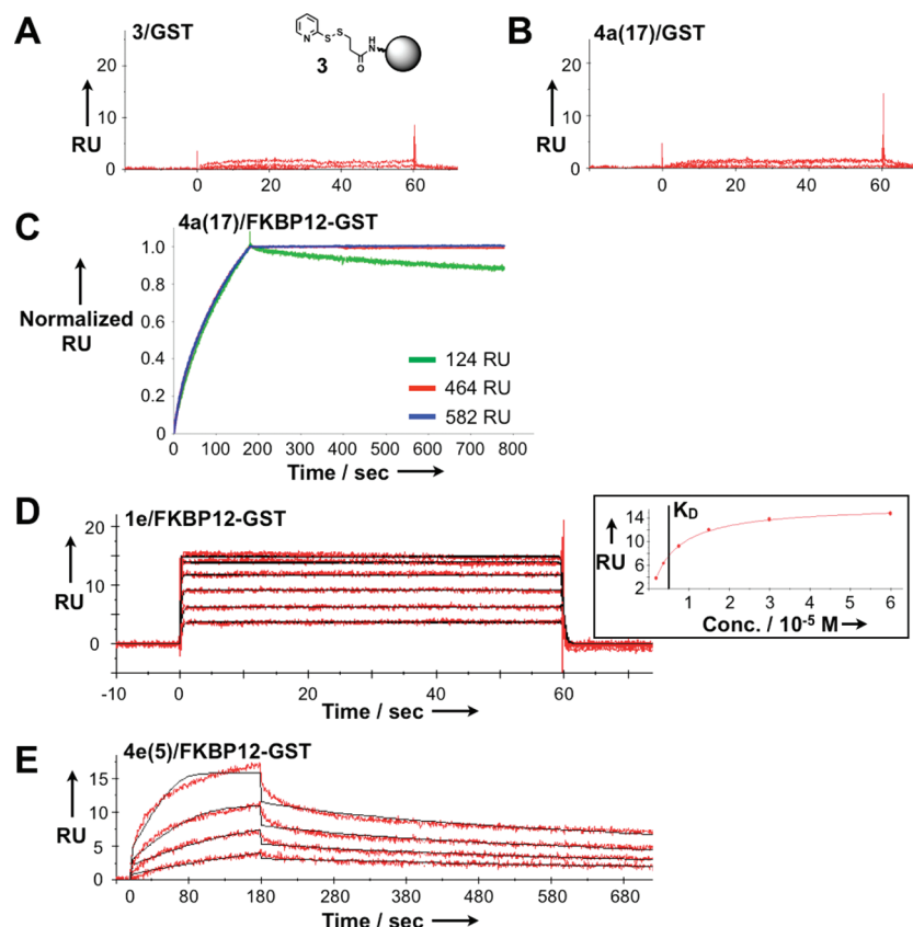
Figure 1. Specific protein–nanoparticle binding documented in SPR sensorgrams. A. Nanoparticle intermediate 3 does not bind to a control surface of GST. B. Targeted nanoparticle 4a(17) does not bind to a GST surface. C. Sensorgrams for targeted nanoparticle 4a(17) at different immobilization densities of FKBP12-GST. Significant binding occurs; appreciable dissociation only occurs at the lowest protein density tested. D. Representative sensorgram for a free small molecule ( 1e ) flowed over an FKBP12-GST surface. Inset: Depiction of calculating K_D from steady-state affinity studies. E. Representative sensorgram for multivalent nanoparticle 4e(5) . In parts D and E, red curves depict experimental data at different analyte concentrations; fitted curves modeled to describe a 1:1 binding event are overlaid in black.
