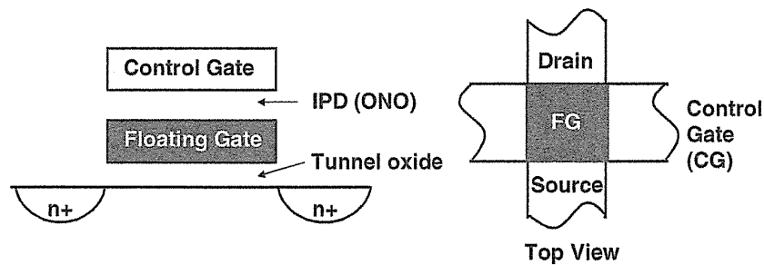
FIGURE 2.1 Single-cell architecture of floating-gate flash memory. Nch MOS transistor with poly-silicon floating gate (FG). The FG is electrically isolated by tunnel oxide and interpoly dielectric (IPD). Charge is stored in FG.
