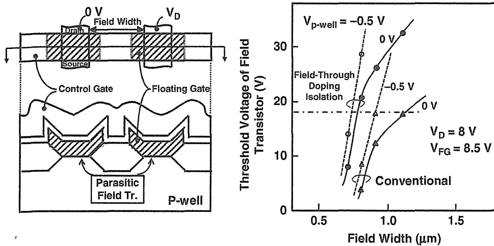
FIGURE 3.9 The threshold voltage of the parasitic field transistor as a function of the field width. By using a field-through implantation process (FTI process), the threshold voltage of a 0.8-μm field transistor becomes higher than 28 V when -0.5 V is applied to the p -well. Copyright 1994, The Japan Society of Applied Physics.
