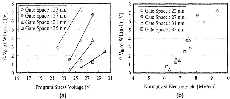
FIGURE 5.56 (a) The V_{th} reduction of WL(n-1) for samples with different gate space after 0.2 s of program stress; the pass voltage is 4.5 V. (b) The V_{th} reduction of WL(n-1) for samples with different gate space. The x-axis is the electric field between the control gate of WL(n) and the WL(n-1) .
