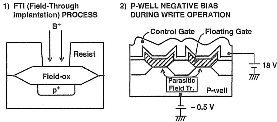
FIGURE 3.7 The 0.8- \mu\text{m} -wide high-voltage field isolation technology. Copyright 1994, The Japan Society of Applied Physics.
