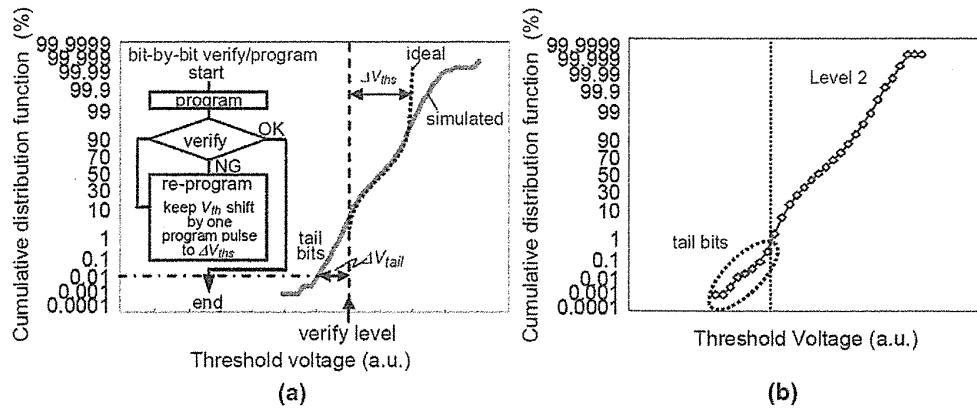
FIGURE 5.40 (a) Monte Carlo simulation results of programmed V_{th} distribution using bit-by-bit verify scheme. (b) Measured V_{th} distribution of Level 2 enlarged.
