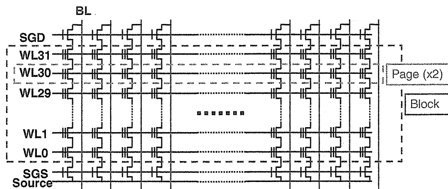
FIGURE 2.4 Array architecture of NAND flash memory cells. Page size is typically 2-K to 16-KByte (2- to 16-KByte cells + ECC code). Block size is typically page \times 2 \times 32 cells = 128-K to 256-KByte cell (physical). Read and program are performed in per page. Erase is performed in per block.
