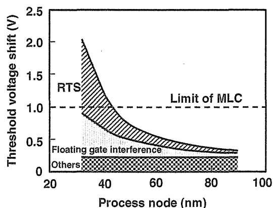
FIGURE 5.45 Estimation of threshold voltage shift as a function of process node.
