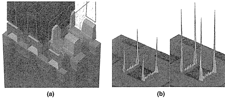
FIGURE 5.69 (a) Template NAND device structure for 3D TCAD (Technology Computer Aided Design) simulations. (b) Calculated tunneling current density at the edge of the selected cell active area along the WL direction, for the All 0 and the All 1 background patterns. A fixed negative V_{FG,s} is used.
