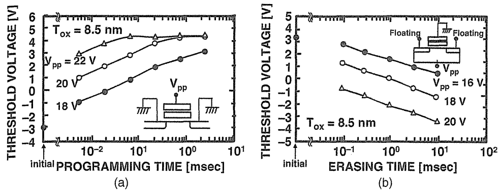
FIGURE 3.54 (a) The program and (b) erase characteristics of the SWATT cell. A short programming time of 200 \mu\text{s} and short erase time of 2 ms can be accomplished by Fowler-Nordheim tunneling over the channel area, applying a positive voltage of 21 V to the control gate during programming and 19 V to the p -well during erasing, respectively.
