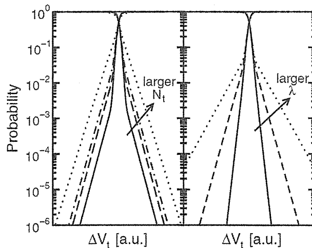
FIGURE 5.43 Cumulative probability distribution of \Delta V_t calculated according to the model for different values of (left) N_t and (right) \lambda .
