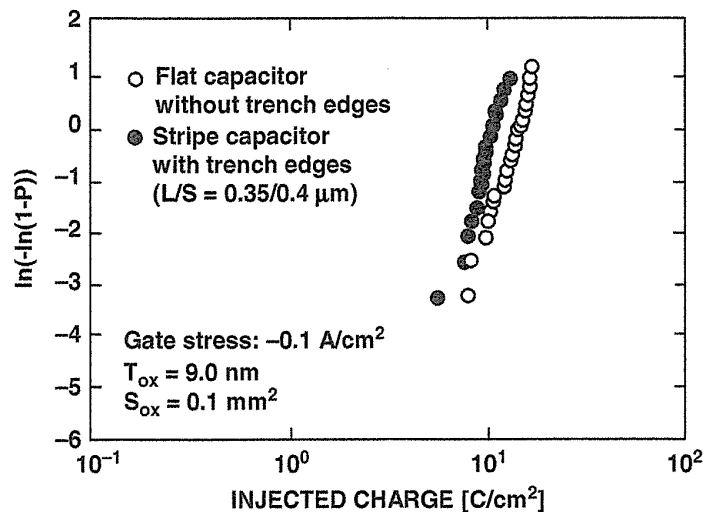
FIGURE 3.26 TDDB (Time Dependent Dielectric Breakdown) characteristics of the tunnel oxide in the STI stripe capacitor and a flat capacitor. The process damages into the tunnel oxides during the SA-STI fabrication steps are negligibly small.
