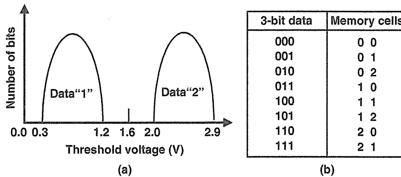
FIGURE 4.33 (a) Threshold distribution for a 3-level memory cell (1.5 bits/cell). (b) Three-bit data and three-level data in memory cells.
