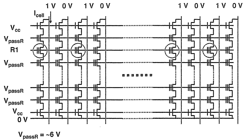
FIGURE 2.8 Read operation of NAND cell array. Page read: 2–16 KByte at the same time. Typical random read speed, t_R : 25 \mu\text{s} for SLC, 60 \mu\text{s} for MLC.
