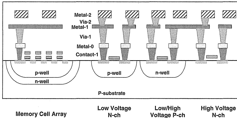
FIGURE 2.5 The cross-sectional view of NAND flash memory.
