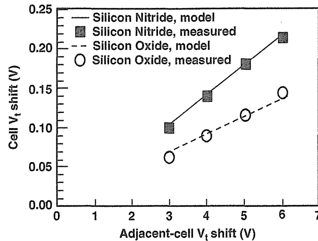
FIGURE 5.15 Floating-gate interference measurement results measured on a 0.12- \mu\text{m} design-rule cell array. The interference was measured on a WL8 cell as a function of WL9-cell V_t change for silicon nitride and silicon oxide spacer samples. Threshold voltage shift of the WL8 cell is monitored before and after WL9-cell programming from V_t = -3 V to 2.2 V. Each data consists of 15 points of a WL8 cell.
