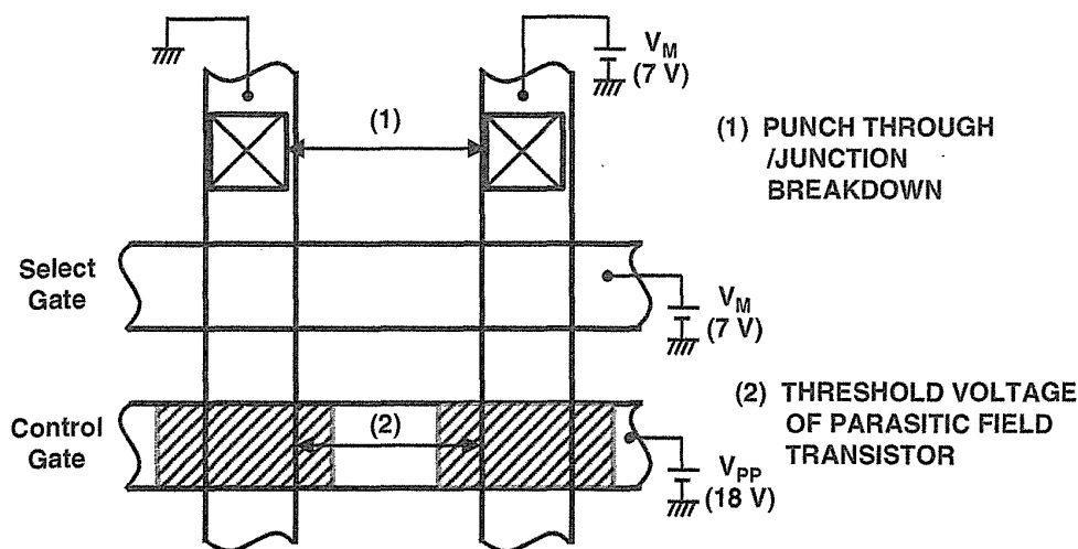
FIGURE 3.6 Isolation between two neighboring bit lines: (1) Punch-through or junction breakdown in the bit-line contact area. (2) The threshold voltage of the parasitic field transistor. Copyright 1994, The Japan Society of Applied Physics.
