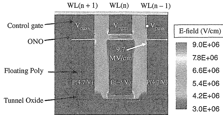
FIGURE 5.55 The simulation result of the electric field distribution under the program operation at t = 0 , where the V_{pgm} is 24 V and the V_{pass} is 8.5 V.
