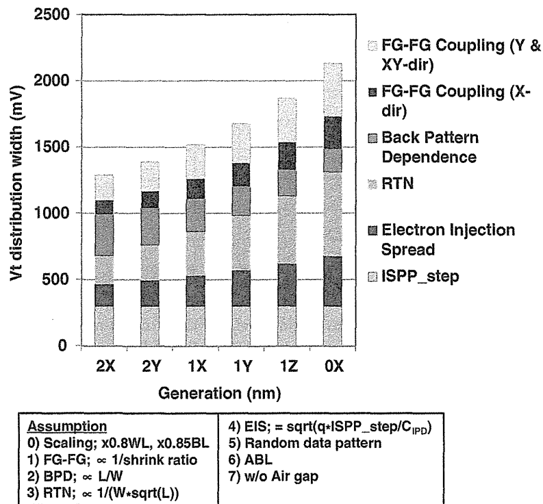
FIGURE 5.7 Calculated programmed V_t distribution width. The V_t distribution width is increased by cell dimension scaling. Major impact factors to increase V_t distributions width are the FG–FG coupling and RTN.
