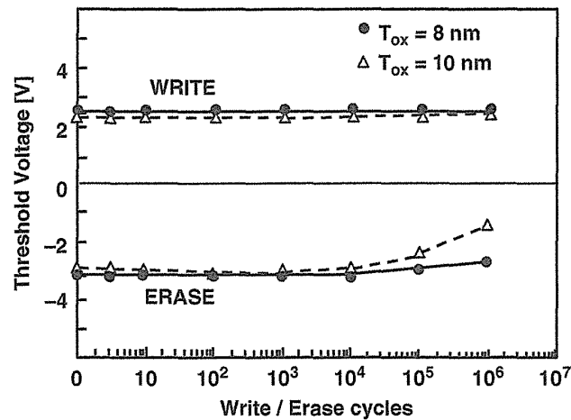
FIGURE 3.11 Program (write) and erase cycling endurance characteristics. The threshold voltage is defined as the control gate voltage which flows a drain current of 1 \mu\text{A} with a drain-source voltage of 1.5 V. For an 8-nm tunnel oxide, we have the following: Program (write): V_{cg} = 18\text{ V} , 0.1 ms. Erase: V_{p\text{-well}} = 20\text{ V} , 1 ms. For a 10-nm tunnel oxide, we have the following: Program (write): V_{cg} = 20.4\text{ V} , 0.1 ms. Erase: V_{p\text{-well}} = 22.7\text{ V} , 1 ms. Window narrowing is almost not observed up to 1 million program (write)/erase cycles. Copyright 1994, The Japan Society of Applied Physics.
