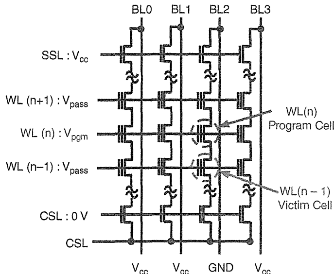
FIGURE 5.52 The schematic diagram for the test module with 4 bit lines and the basic program condition for the self-boasting scheme.
