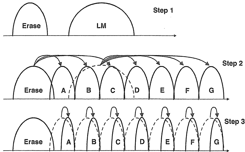
FIGURE 4.28 Three-step program algorithm for a 19-nm node cell.
