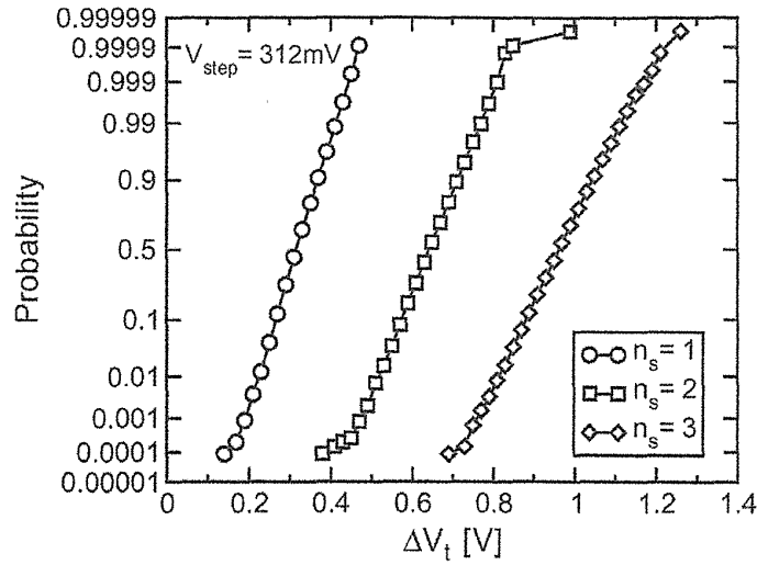
FIGURE 5.30 Experimental \Delta V_t distributions for V_{\text{step}} = 312 \text{ mV} and increasing n_s , showing the increase of \sigma_{\Delta V_t} that follows the larger average \Delta V_t value.
