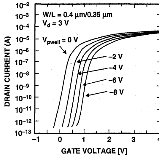
FIGURE 3.38 The subthreshold characteristics of the SA-STI cell with various substrate ( p -well) bias conditions. Anomalous subthreshold characteristics (hump) cannot be seen because the floating-gate dose not overlap the trench corner.
