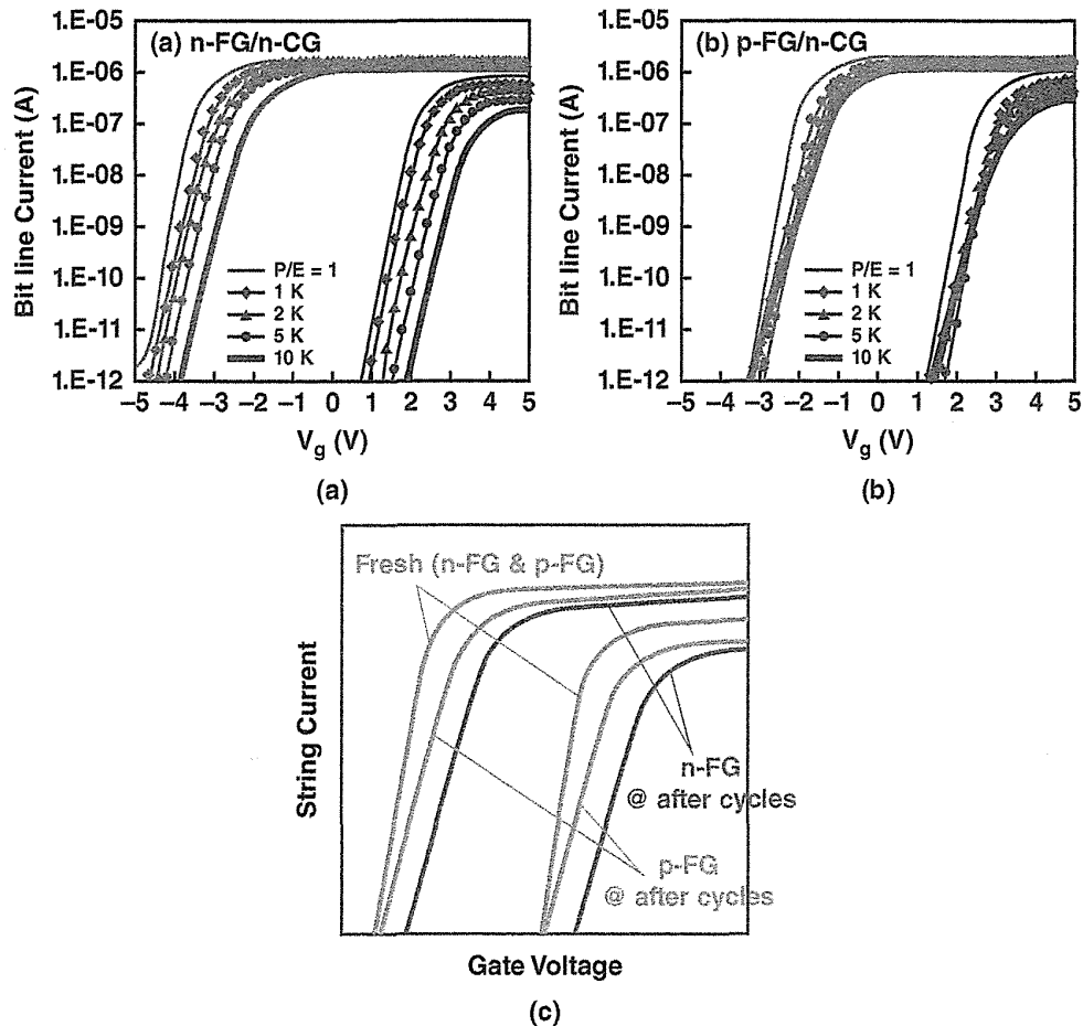
FIGURE 3.67 Experimental I_d - V_g characteristics of (a) n -FG and (b) p -FG cells ((a) n -FG/n-CG cell and (b) p -FG/n-CG cell) before and after P/E cycling. (c) Schematic I_d - V_g curve of cell transistor for n -type and p -type floating gate before/after P/E cycling.
