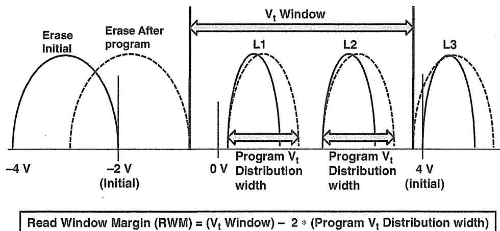
FIGURE 2.25 Read V_t window of an MLC NAND cell.
