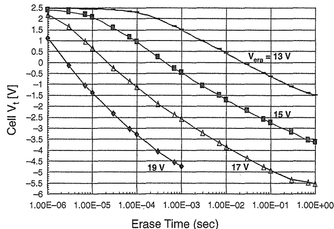
FIGURE 2.16 Erase characteristics. Higher erase voltage can be faster operation. Erase speed, t_{era} : 2–5 ms.
