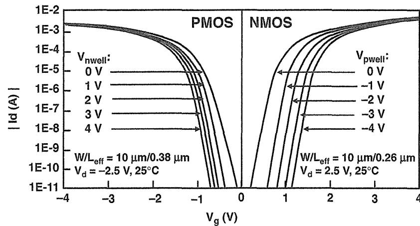
FIGURE 3.29 A subthreshold characteristics of the low-voltage peripheral transistor (NMOS and PMOS) as a function of well voltage.
