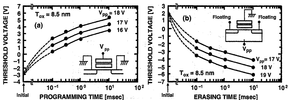
FIGURE 3.39 (a) Program and Erase characteristics of the SA-STI cell. The fast programming (100 \mu\text{s} ) and erasing (2 ms) can be accomplished by Fowler-Nordheim tunneling over the channel area, applying a positive voltage of 17 V to the control gate during programming and 17 V to the p -well during erasing, respectively.
