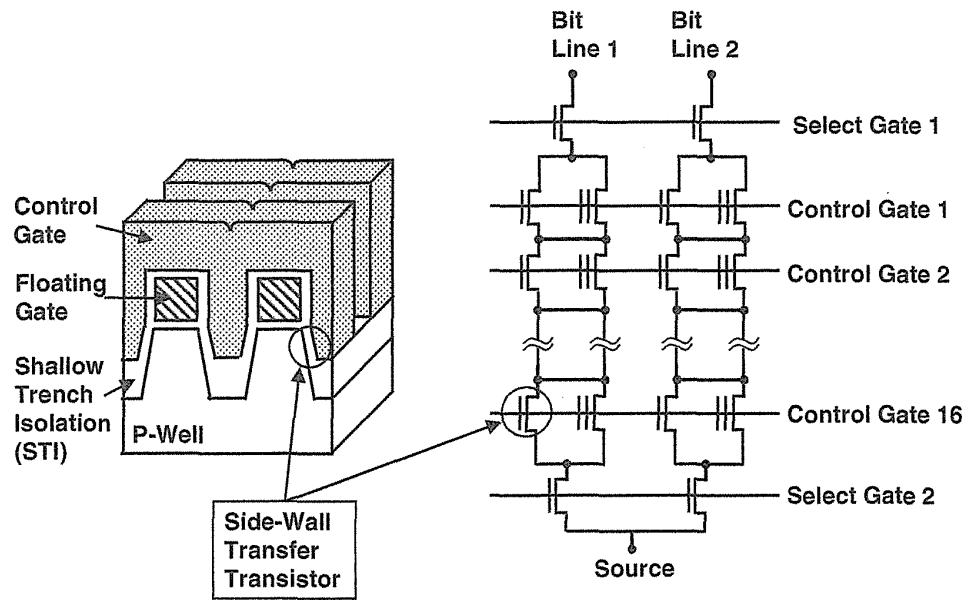
FIGURE 3.48 The schematic view and equivalent circuit of the sidewall transfer transistor cell (SWATT cell). A transfer transistor is located at the sidewall of the shallow trench isolation (STI) region and is connected in parallel with the floating-gate transistor.
