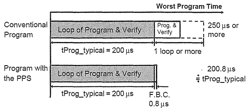
FIGURE 4.14 Program performance of a conventional page program and a page program with PPS.
