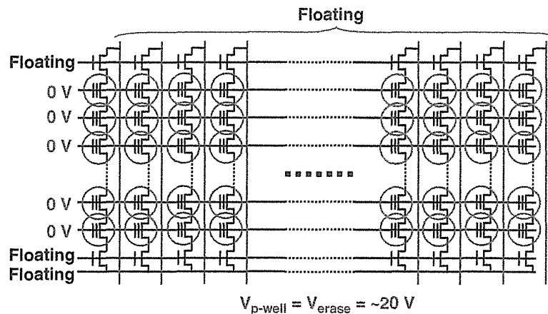
FIGURE 2.15 Erase operation of NAND flash cell array. Block erase: 128- to 256-KByte (2-KByte \times 2 \times 32) cells are erased at the same time. Erase speed, t_{erase} : 2–5 ms with erase verify.
