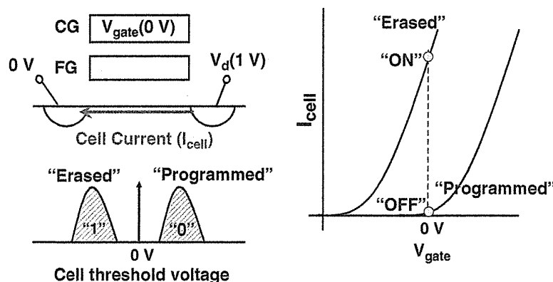
FIGURE 2.7 Principle of read of single cell. Erased: Positive charge in FG. I_{\text{cell}} “ON”. Programmed: Negative charge in FG. I_{\text{cell}} “OFF”.
