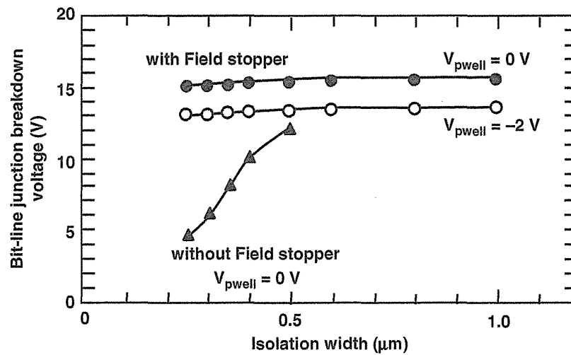
FIGURE 3.21 A breakdown voltage of the bit-line junctions, which is isolated by STI. There is no punch-through at less than 15 V, which is the junction breakdown voltage using boron field stopper implantation.
