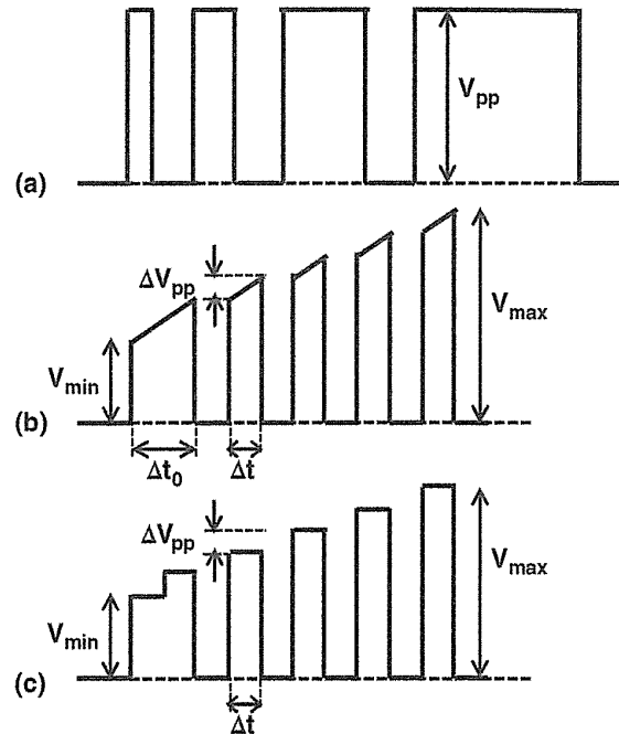
FIGURE 4.5 Program pulse waveforms: (a) conventional, (b) trapezoidal, and (c) staircase (incremental step pulse programming (ISPP)). A verify step is carried out after each pulse.
