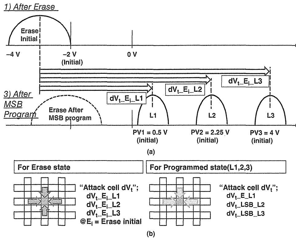
FIGURE 5.11 The FG–FG coupling for the erase state. (a) The attack cell (neighbor of target cell) V_t shift of dV_{t\_E\_L1} or dV_{t\_E\_L2} or dV_{t\_E\_L3} are subjected to the erased target cell. The V_t shift of the erased state is larger than that of programmed state because an attack cell V_t shift for erased state is larger than that of programmed state (see Fig. 5.10), and also (b) all of the surrounding cells have been subjected to erased cells, compared to the fact that all of surrounding cells have not been subjected to a programmed state.
