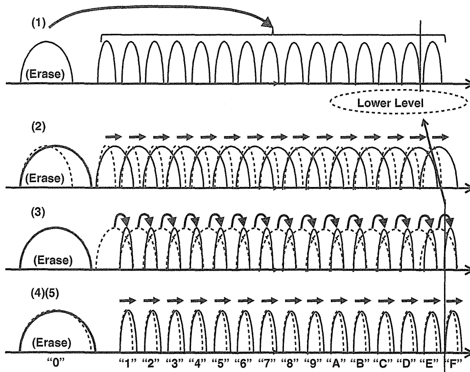
FIGURE 4.30 V_{th} distribution transition of 16LC (QLC, 4 bits/cell).
