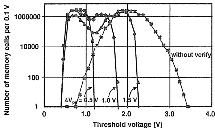
FIGURE 4.6 V_t distribution after programming in a 16-Mbit memory array, with/without verify, using staircase pulses (ISPP) with length of 20 \mu s and V_{pgm} step of 0.5, 1.0, 1.5 V.
