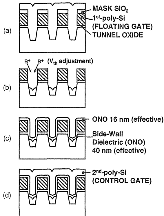
FIGURE 3.51 The process sequence of the SWATT process. (a) Trench etching, LP-CVD \text{SiO}_2 fill-in. (b) Oxide etch-back and B + implantation of the V_{th} adjustment of the side wall transfer transistor. (c) ONO formation. (d) Control gate formation. The thermal oxide of the STI sidewall is about two times thicker than that on the poly-silicon due to oxidation enhancement at the STI sidewalls.
