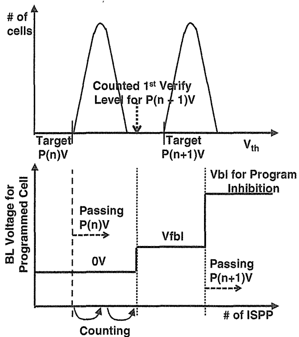
FIGURE 4.11 Forcing BL voltage by latch counting.
