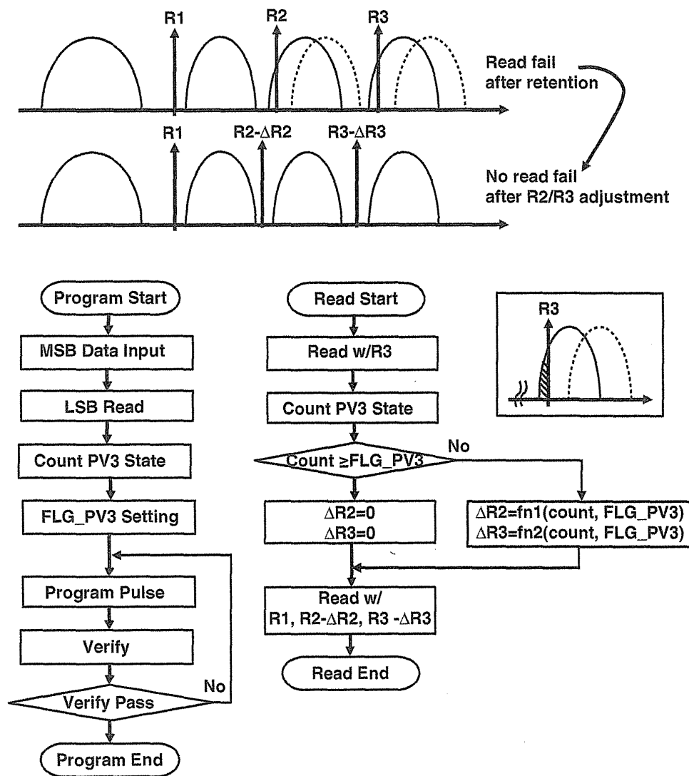
FIGURE 4.36 Moving read algorithm.
