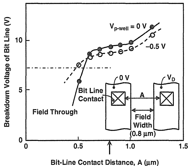
FIGURE 3.8 The breakdown voltage of the bit-line junction. The punch-through voltage and junction breakdown voltage are higher than 7 V at a 0.8- \mu\text{m} bit-line contact distance. Copyright 1994, The Japan Society of Applied Physics.
