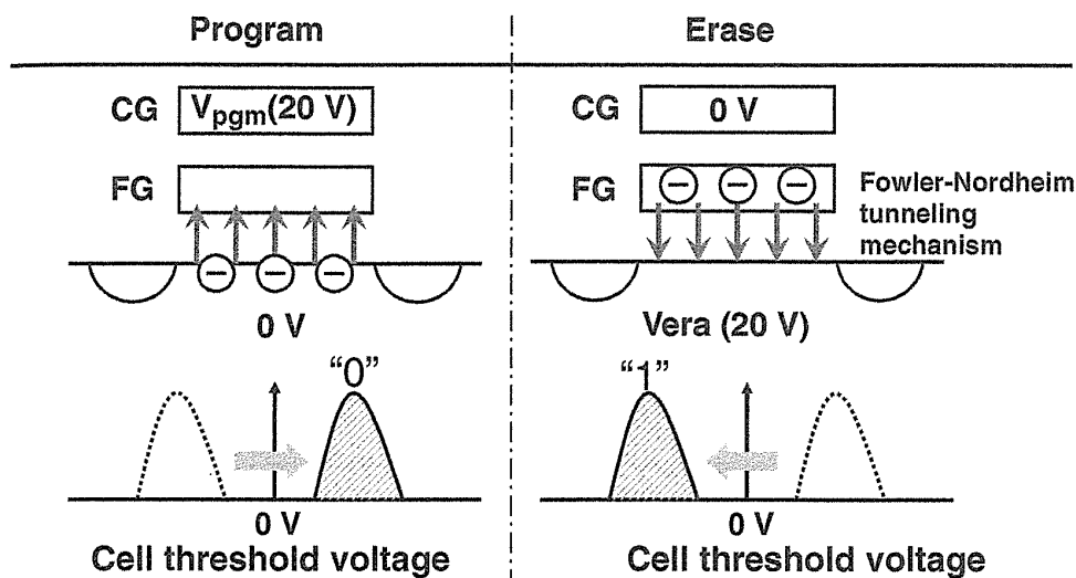
FIGURE 2.10 Principle of single-cell program and erase. Program: Injected electron to the FG through tunnel oxide. Erase: Ejected electron from the FG.
