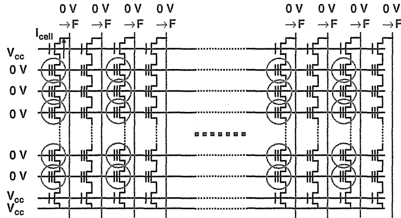
FIGURE 2.17 Erase verify operation.
