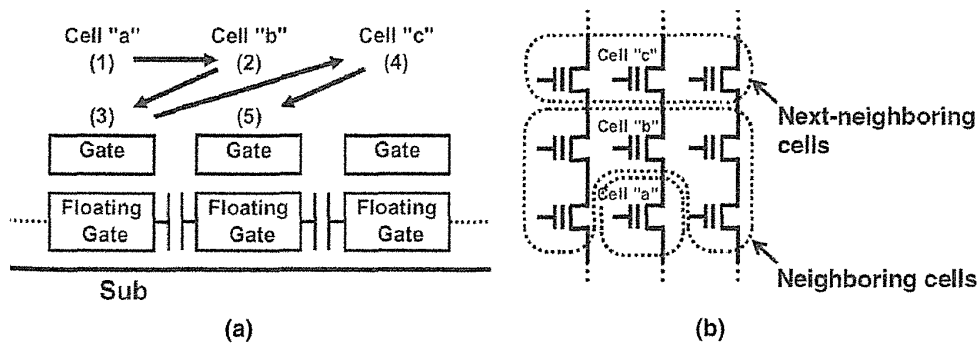
FIGURE 4.21 Programming order over word lines.
