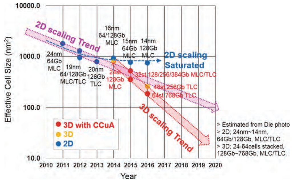
Fig. 5.34 Effective cell size trend
