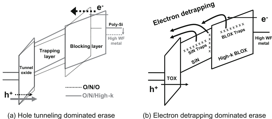
Fig. 4.33 TANOS erase due to reduced electron back tunneling [48]
