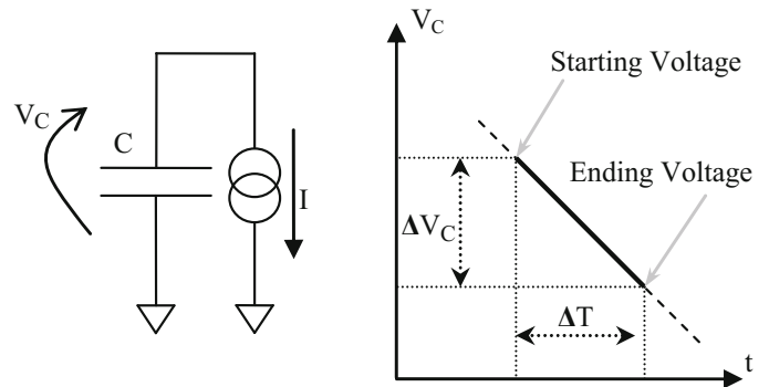
Fig. 6.21 Capacitor discharge through a constant current source
