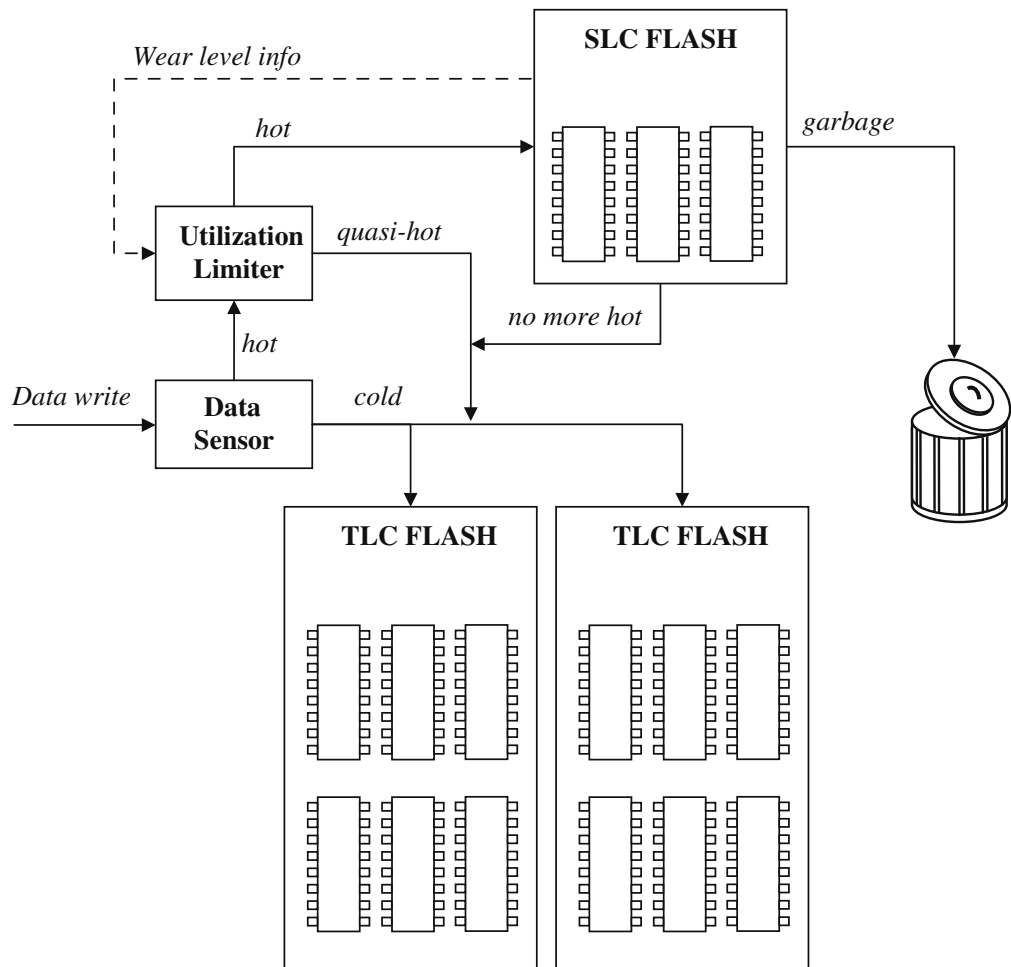
Fig. 3.10 Write flow
