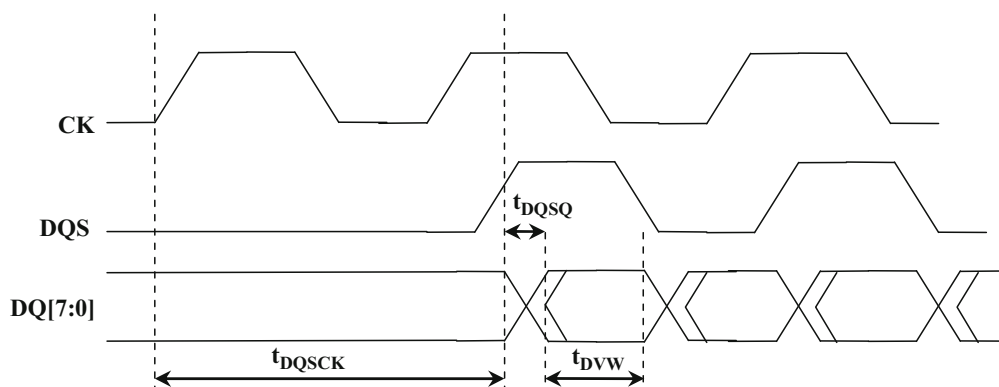
Fig. 6.10 DDR timing diagram
