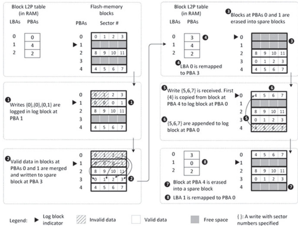
Fig. 10.4 A scenario of our disk-emulation algorithm
