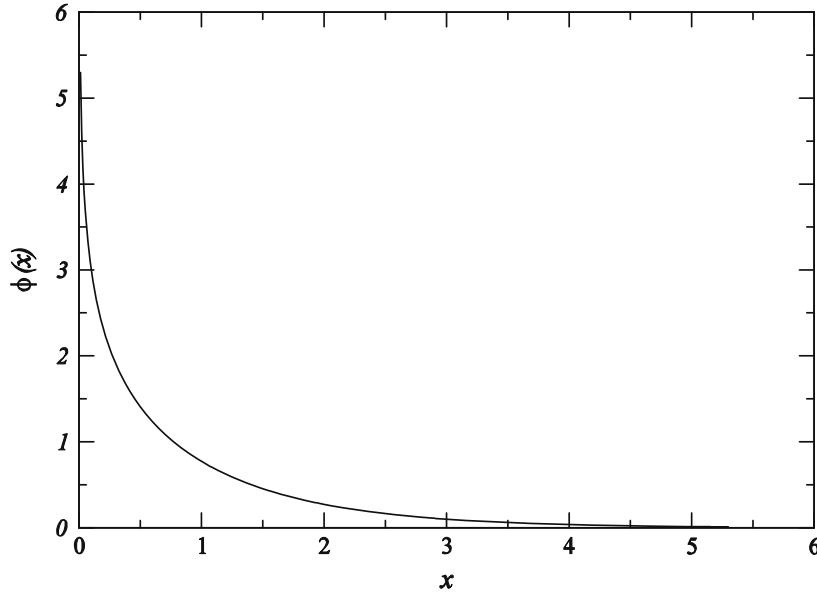
Fig. 12.15 Plot of function \varphi(x) = -\log(\tanh(x/2)) .
