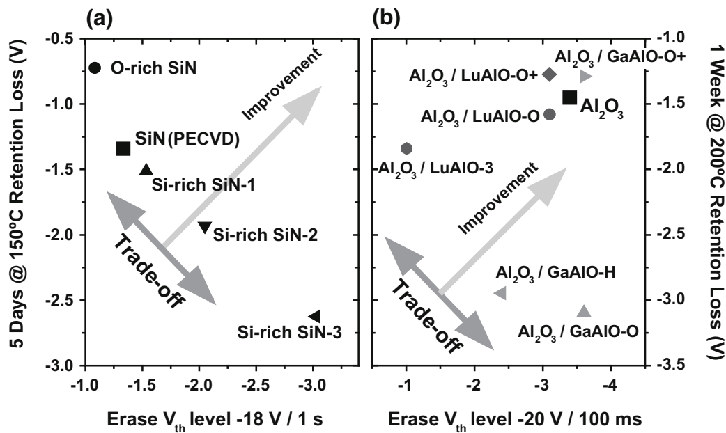
Fig. 4.35 TANOS trade-off between erasability and retention performance on large memory cells ( \mu\text{m} range) with variation of the Si content in the SiN CTL (a) [50], and for different high-k layers on top of the Al 2 O 3 blocking oxide (b) [51]
