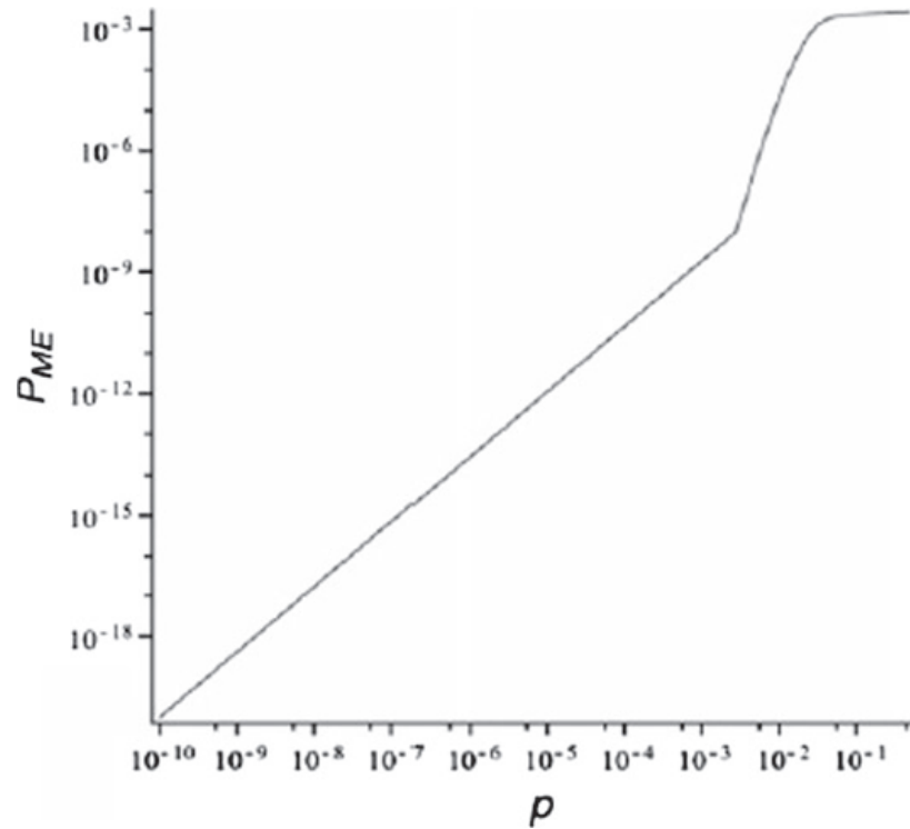
Fig. 11.8 P_{ME} behavior for BCH[255,207,13]
