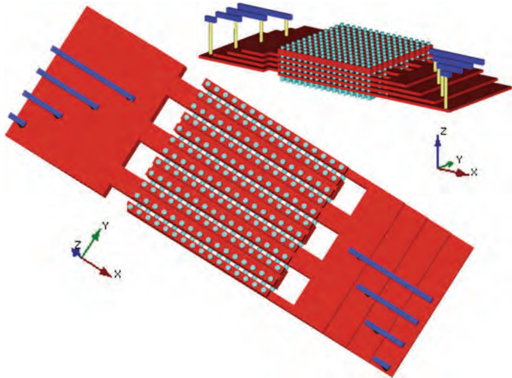
Fig. 5.10 Fork-shaped fan-out
