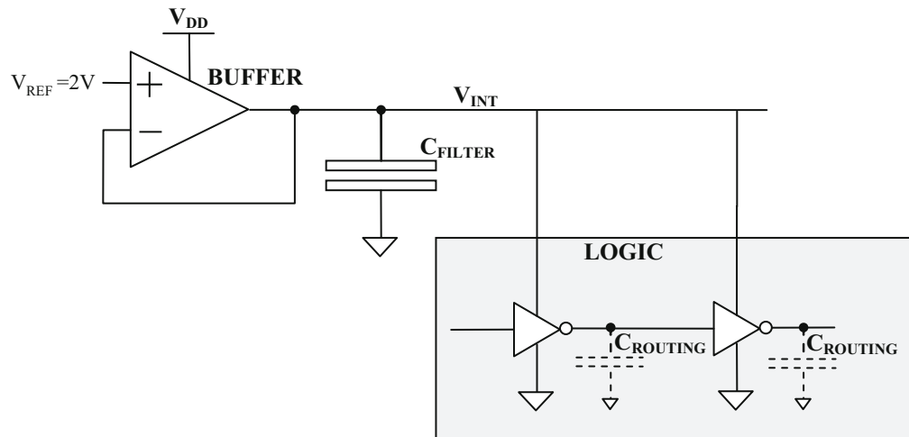
Fig. 6.38 Conceptual scheme of a DC-DC converter
