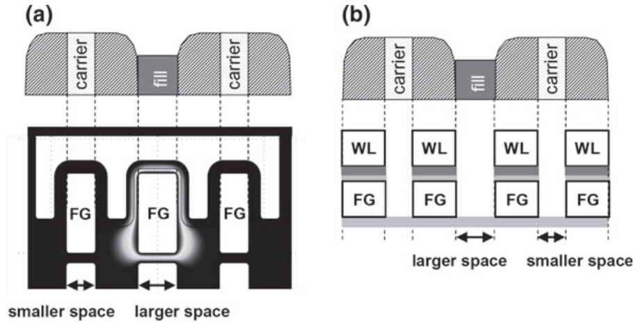
Fig. 4.31 Major variations in LBF (a) and LBS (b) pitch fragmentation sequences [28]
