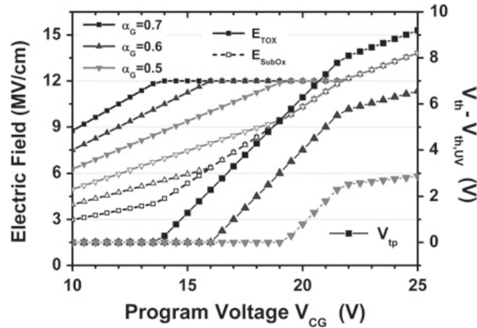
Fig. 4.8 Effect of FG cell geometrically increased gate coupling ratio \alpha_G on program saturation. The TOX thickness t_{TOX} = 8 nm and the ONO layer thicknesses ( t_{SubOx}/t_{SiN}/t_{TopOx} = 4/4/4 nm) are unchanged
