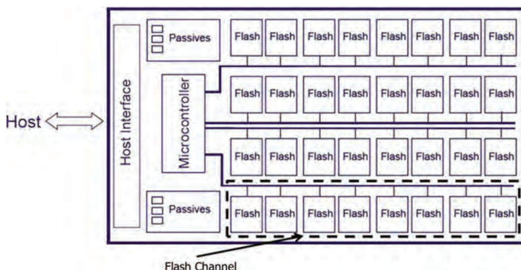
Fig. 1.1 Block diagram of a SSD
