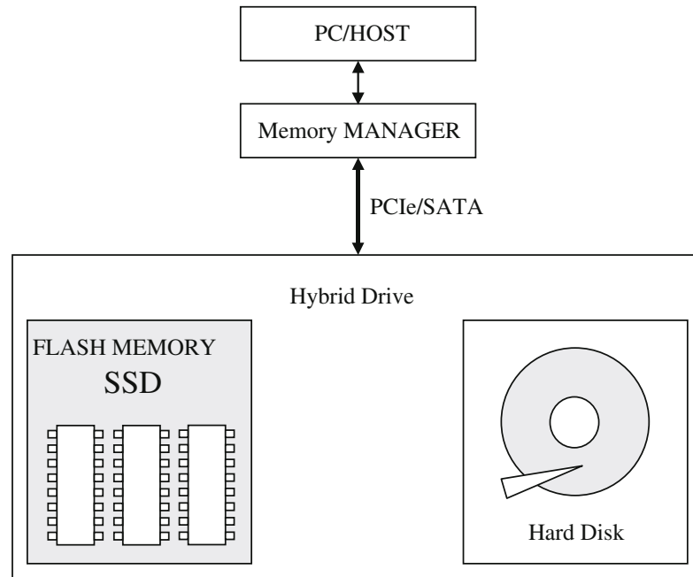
Fig. 3.6 Monolithic hybrid drive
