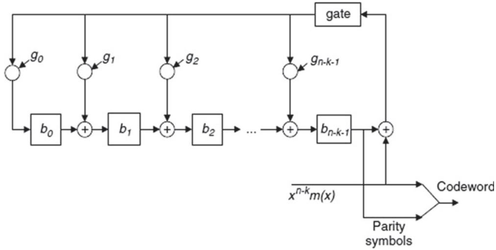
Fig. 11.4 Binary BCH encoder
