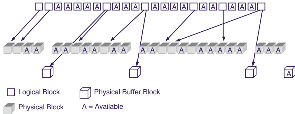
Fig. 1.10 Logical to physical block management
