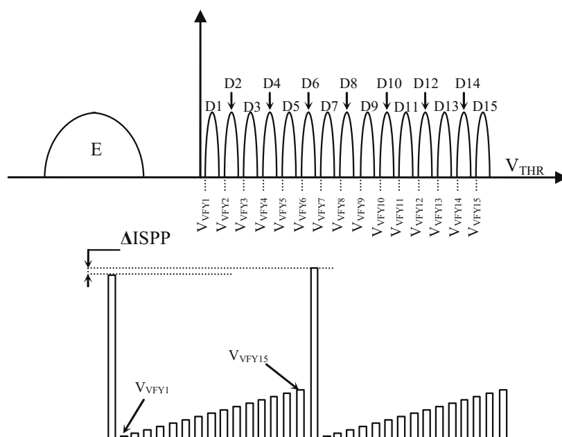
Fig. 6.34 4 bit/cell programming algorithm
