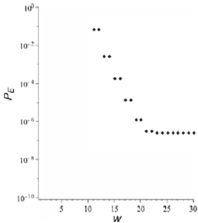
Fig. 11.16 P_E zoom on the first weights for BCH [4095,3975,21]
