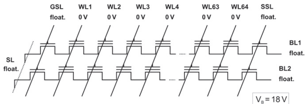
Fig. 4.13 The erase of floating gate cells in the NAND array is carried out in electrically separated erase sectors. By applying a positive voltage (e.g. V_B = 18 V) to the well of the erase sector, all cells are erased at the same time
