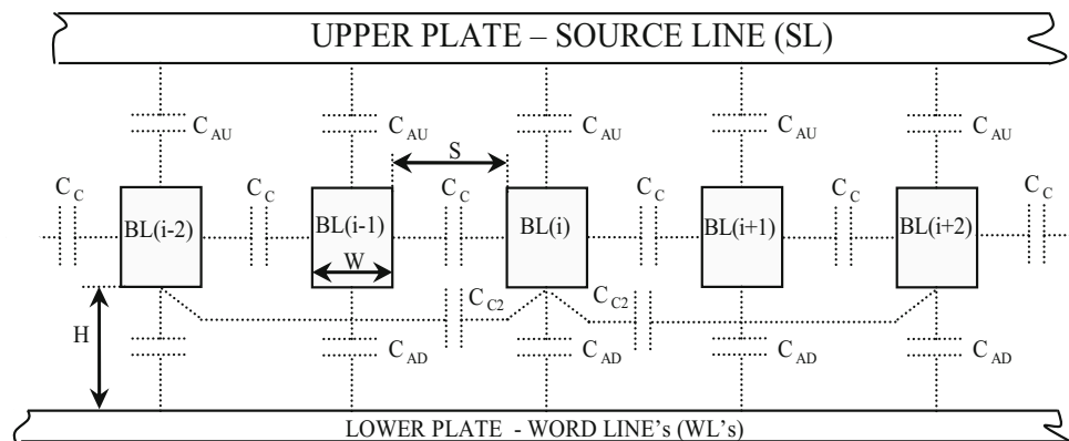
Fig. 6.24 Bitline parasitic capacitors
