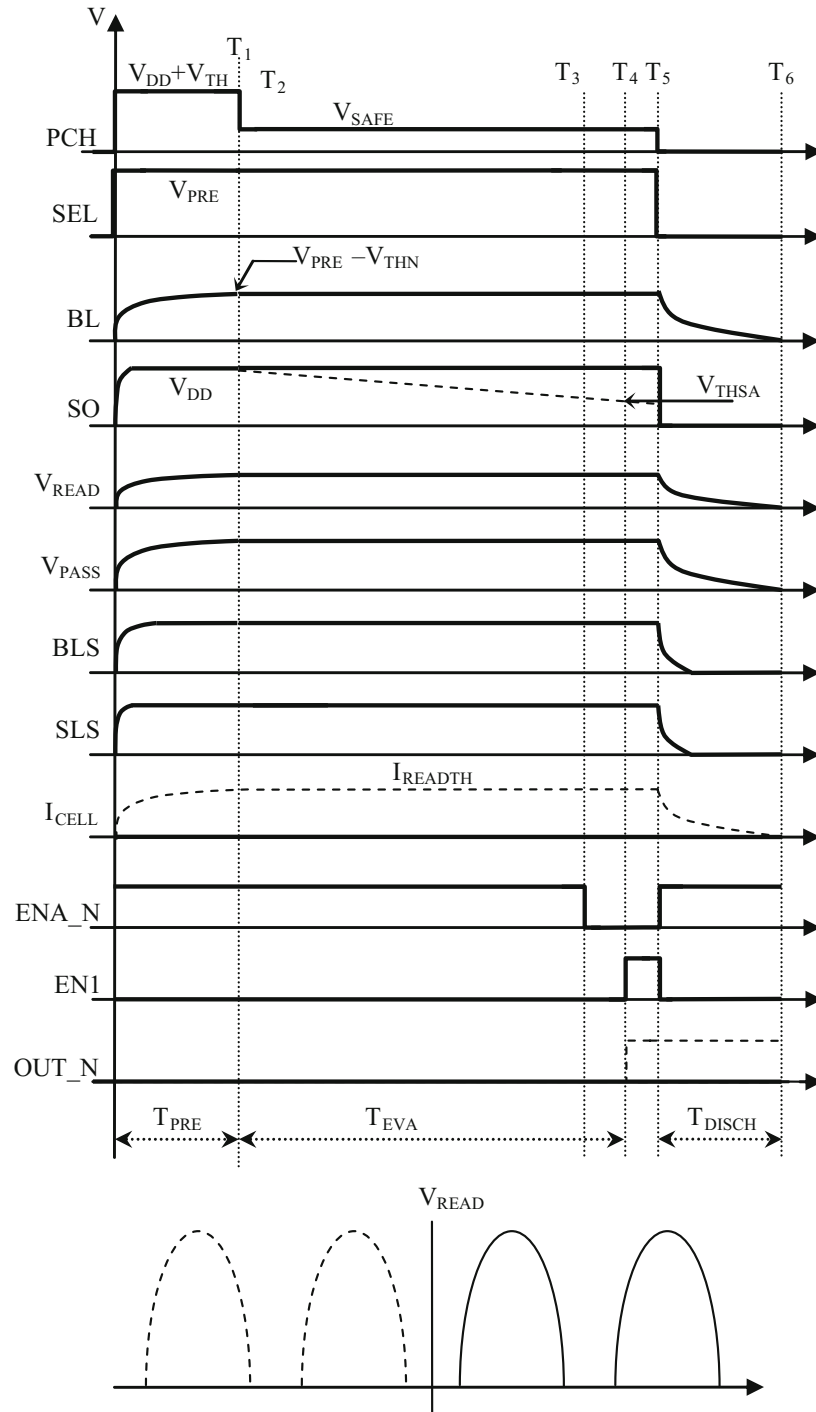
Fig. 6.27 ABL single read operation (SRO) timing diagram
