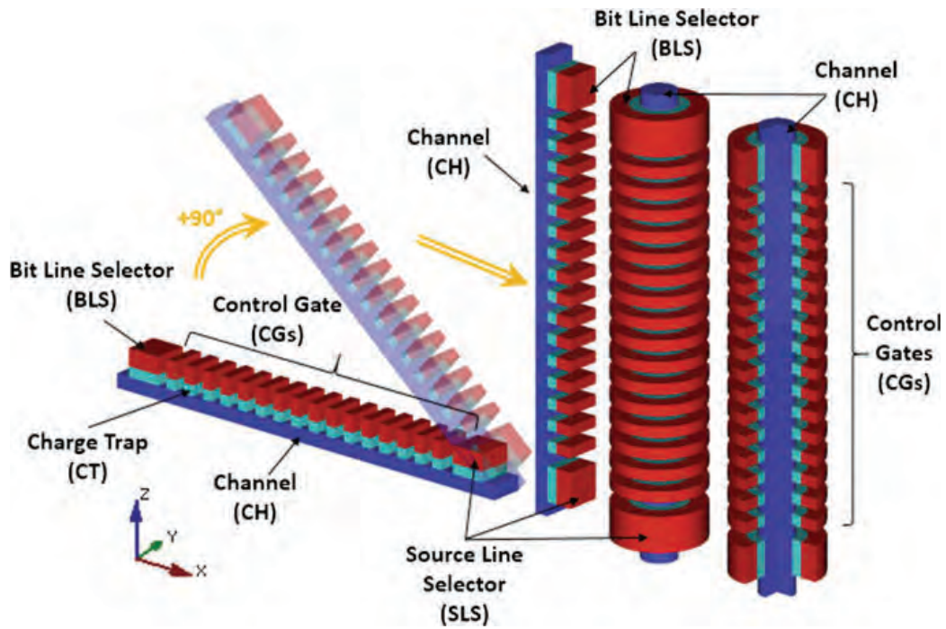
Fig. 5.2 The NAND Flash string goes vertical
