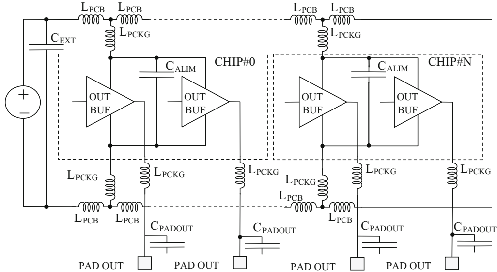
Fig. 6.15 Model example used to evaluate SSN
