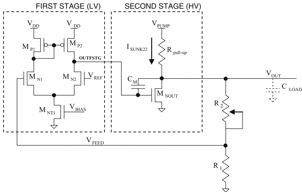
Fig. 6.40 Double-supply voltage regulator
