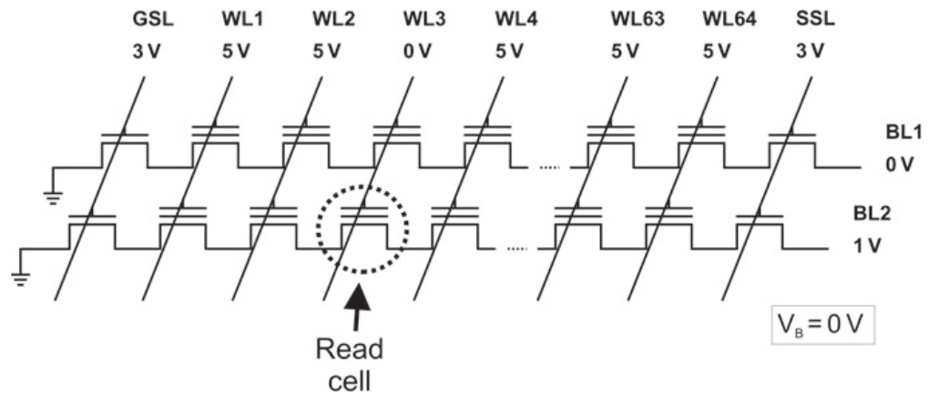
Fig. 4.14 Read operation in the NAND Flash array
