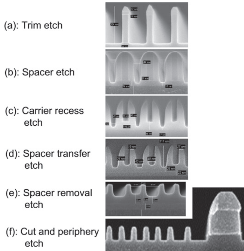
Fig. 4.30 Exemplary line-by-spacer process sequence [28, 39]
