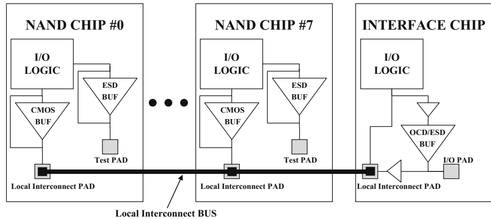
Fig. 6.12 Local interconnect bus architecture
