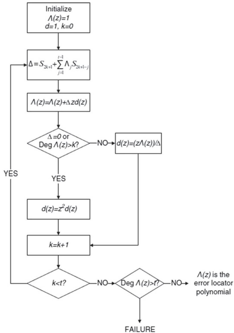
Fig. 11.5 Flow diagram for the Berlekamp algorithm
