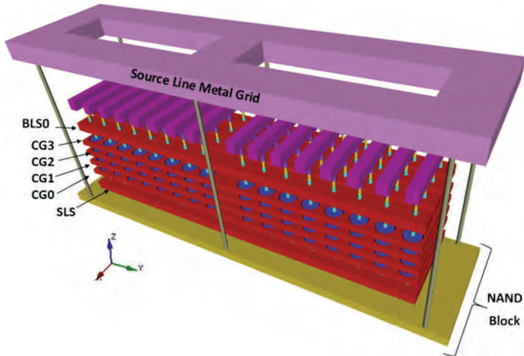
Fig. 5.21 C-FG array with source line metal grid
