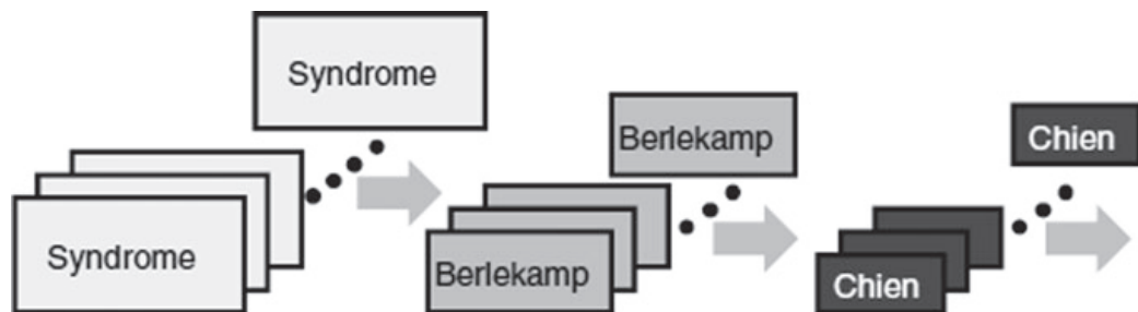
Fig. 11.24 ECC decoding structure for handling multiple channels
