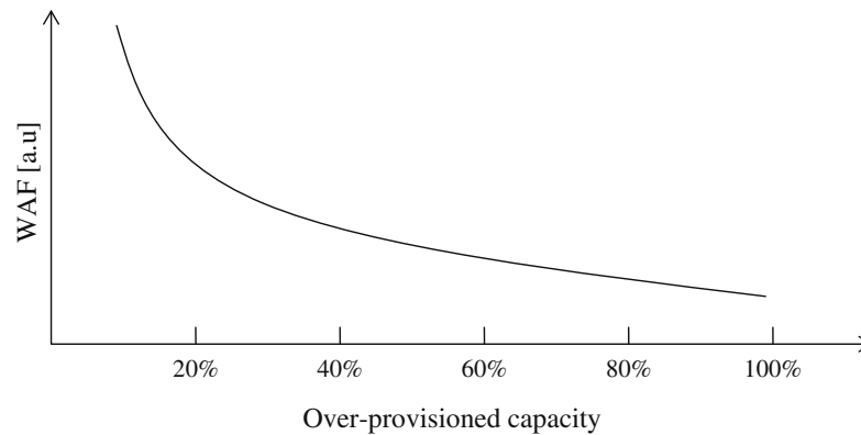
Fig. 3.12 Write amplification factor (WAF) versus over-provisioned capacity
