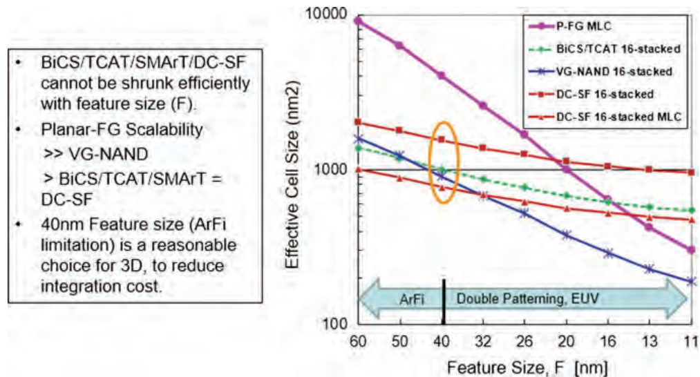
Fig. 5.1 3D NAND Flash scaling [7]
