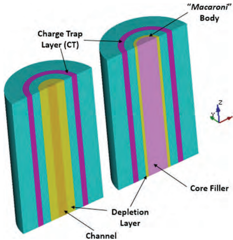
Fig. 5.6 A vertical transistor (right) modified with Macaroni body (left)
