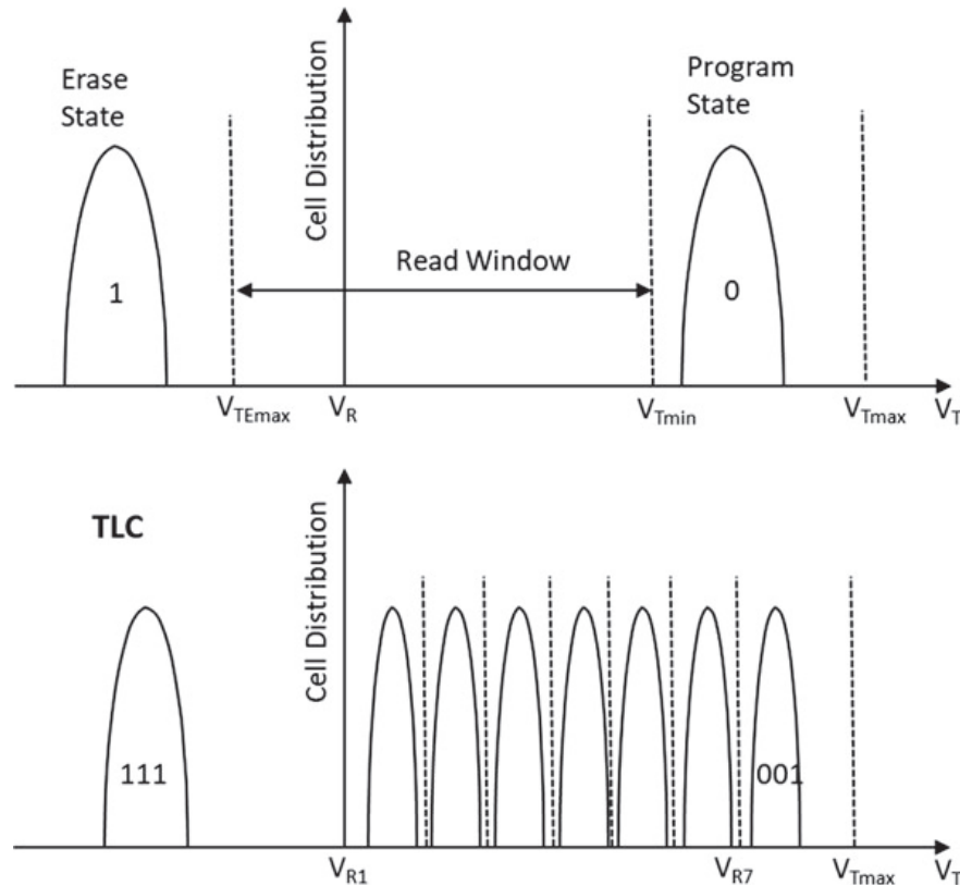
Fig. 8.2 Threshold voltage distributions in a SLC (top) and a TLC (bottom) NAND Flash array. V_{Tmin} and V_{Tmax} represent the minimum and the maximum target V_T for a programmed cell, respectively. V_{TEmax} represents the maximum V_T for an erased cell while V_R denotes the read voltage
