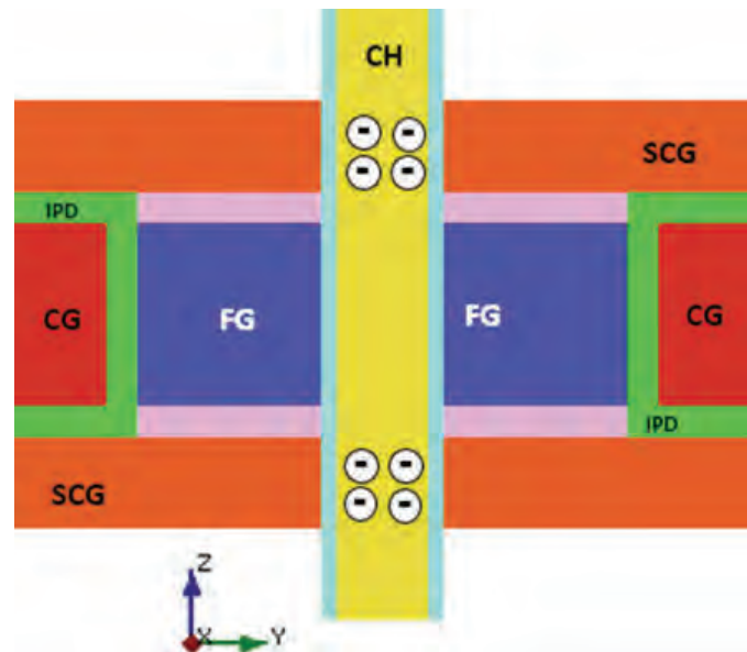
Fig. 5.26 Common SCG approach to enable Source/Drain inversion
