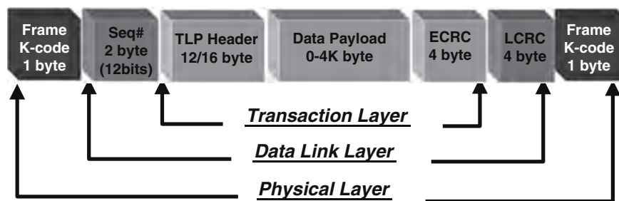
Fig. 1.21 Transaction layer packet (TLP) assembly
