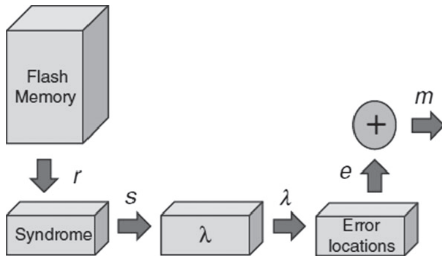
Fig. 11.3 Structure of a binary BCH decoder
