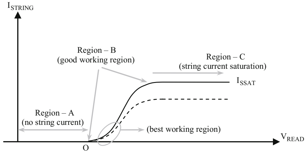
Fig. 6.20 Cell current characteristics versus gate voltage
