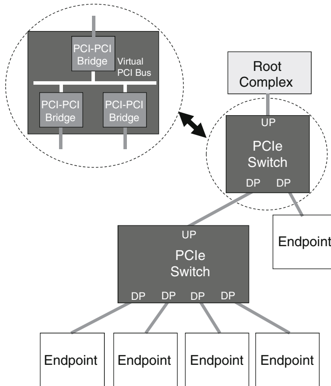
Fig. 1.18 PCIe tree topology
