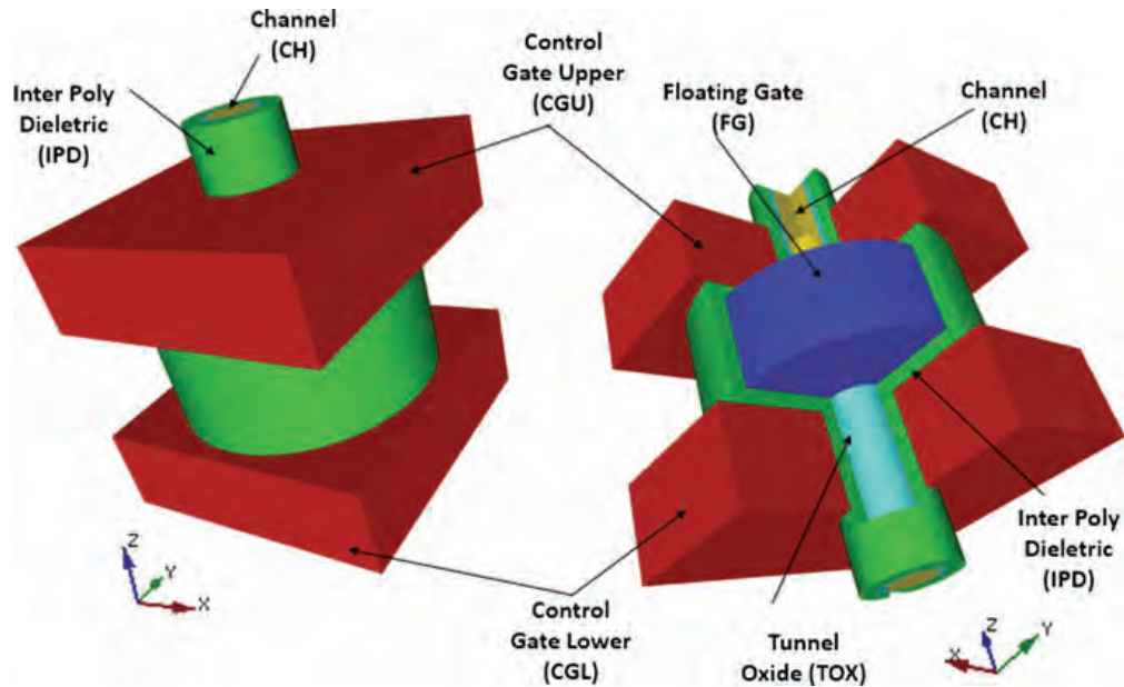
Fig. 5.23 DC-SF NAND Flash cell
