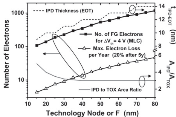
Fig. 4.25 Number of electrons as a function of the technology node F . To have the programming voltages remain similar over different technology generations, the gate coupling ratio is optimized by means of an IPD EOT reduction and an increase of the CG-FG to TOX area ratio
