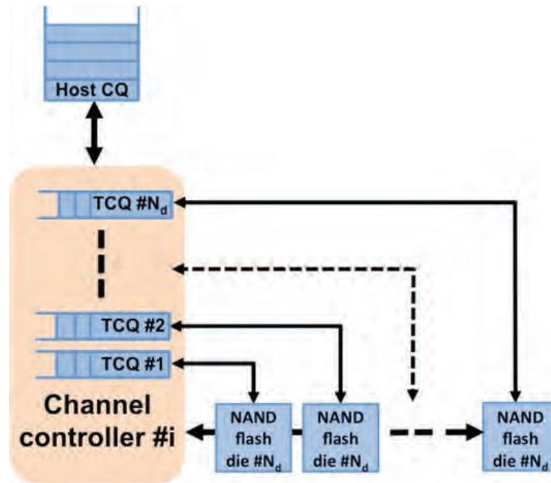
Fig. 7.8 Queuing hierarchy implemented inside the SSD controller for a generic channel. Reproduced with permission from L. Zuolo, C. Zambelli, R. Micheloni and P. Olivo, “Solid-State Drives: Memory Driven Design Methodologies for Optimal Performance”, in Proceedings of the IEEE, vol. 105, no. 9, pp. 1589–1608, Sept 2017. © 2017 IEEE
