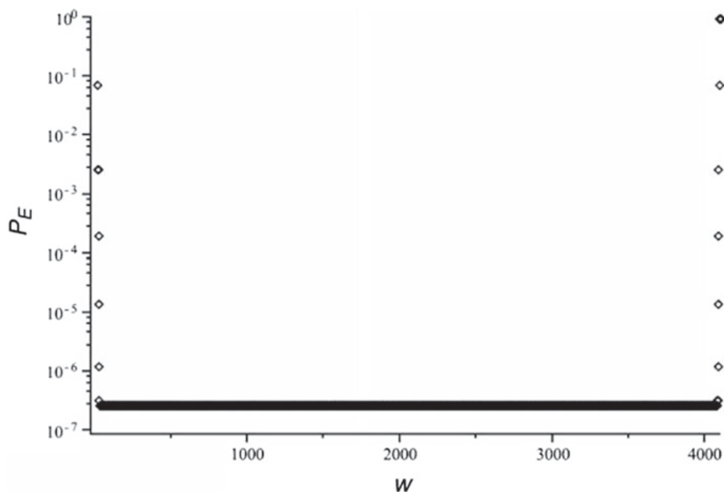
Fig. 11.15 P_E behavior for BCH[4095,3975,21]
