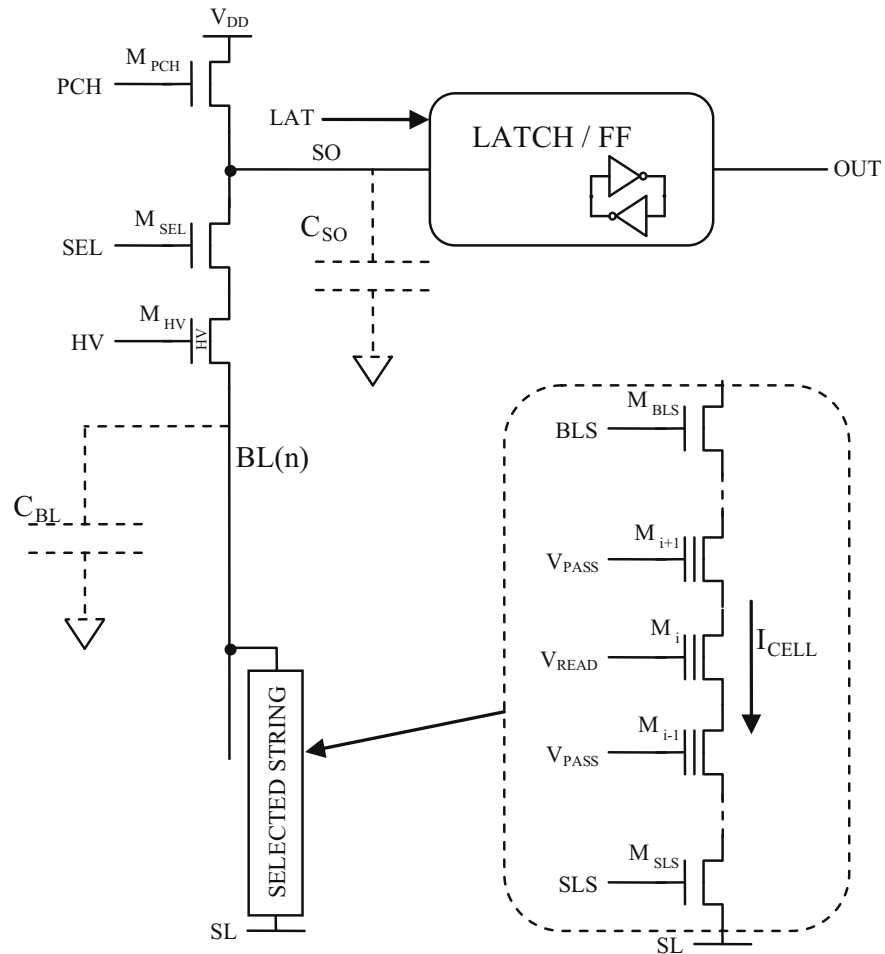
Fig. 6.23 Basic elements of the sense amplifier
