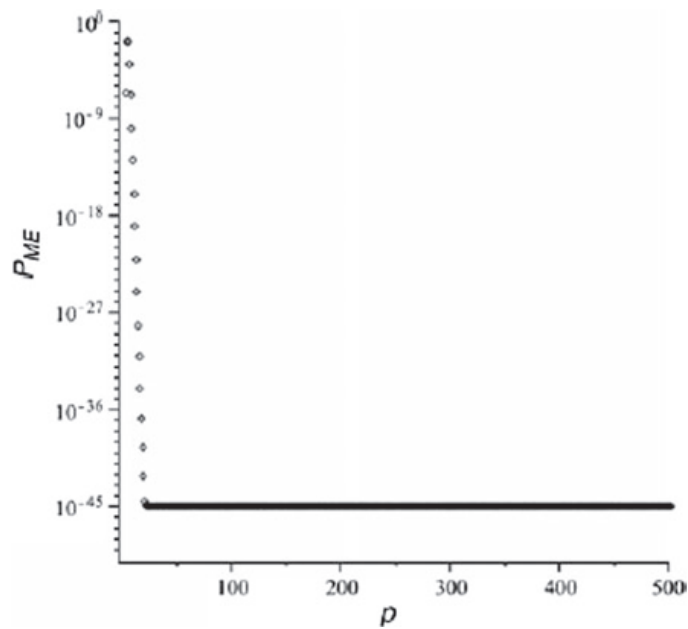
Fig. 11.18 P_{ME} behavior for BCH[16383,15851,77]
