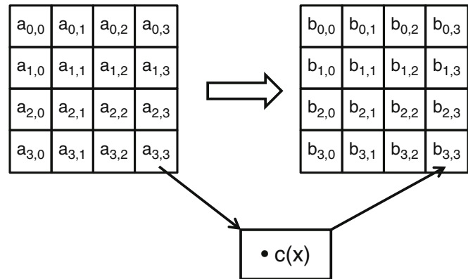
Fig. 13.21 Representation of the MixColumn operation
