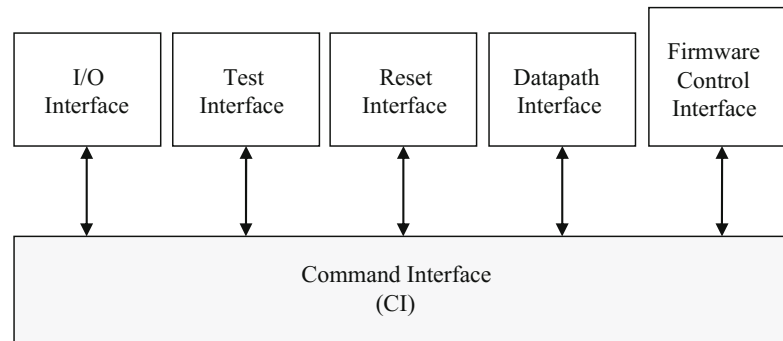
Fig. 6.3 Command interface and its interaction blocks
