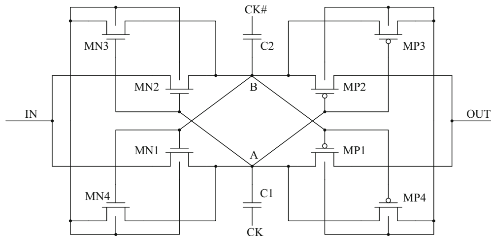
Fig. 6.35 Basic stage of a voltage doubler
