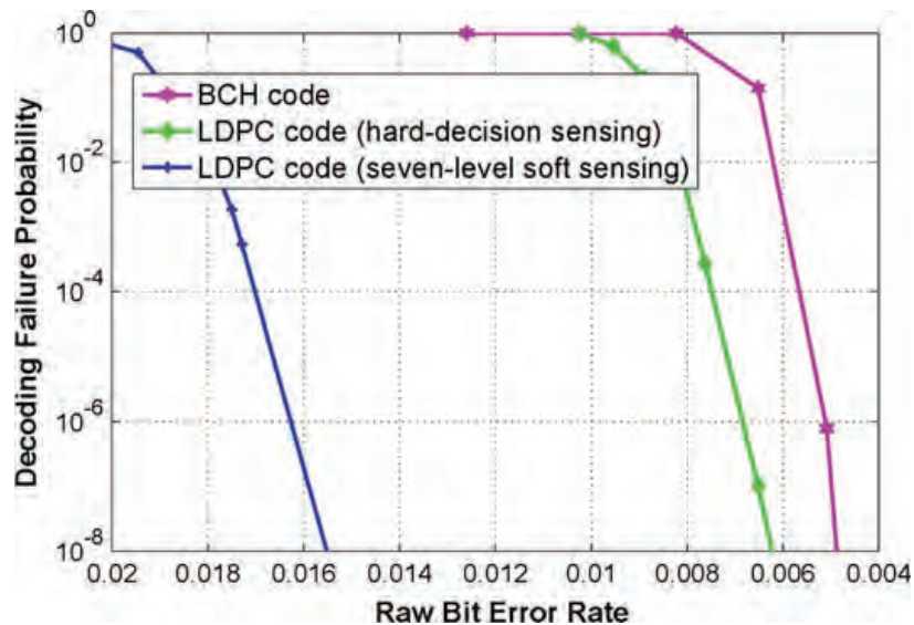
Fig. 8.9 Simulation results of BCH and LDPC codes to be exploited in NAND Flash raw bit errors mitigation. Reproduced with permission from [30]. © 2013 IEEE
