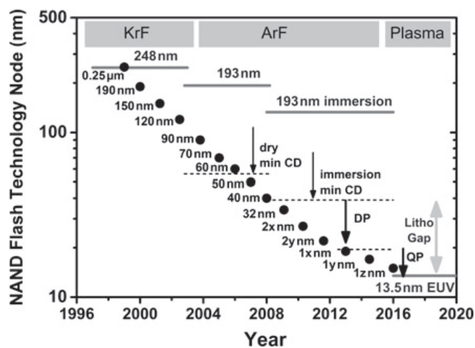
Fig. 4.28 NAND Flash technology generations and lithographic resolutions
