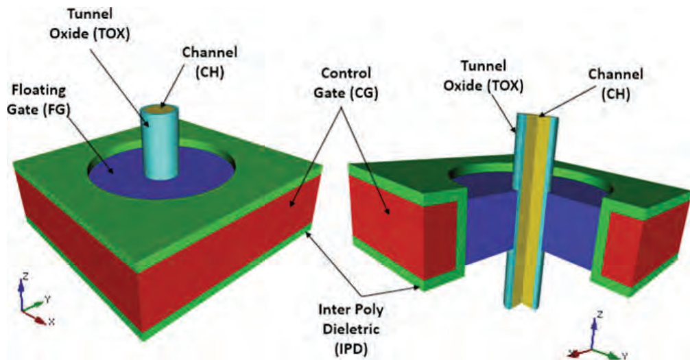
Fig. 5.17 3D C-FG cell
