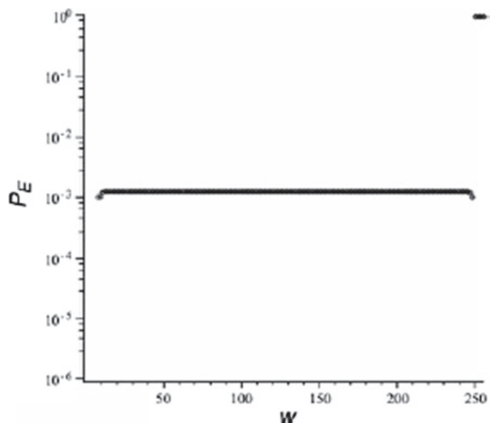
Fig. 11.20 P_E behavior for BCH[255,207,13] using Peterson estimation
