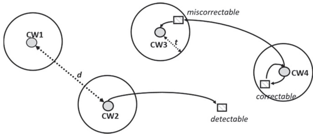
Fig. 11.26 Sphere-packing scheme for a bounded distance decoder
