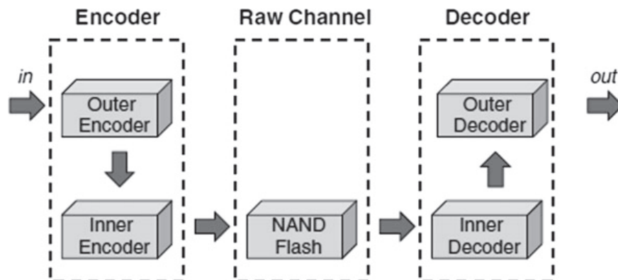
Fig. 11.2 Schematic diagram of code concatenation
