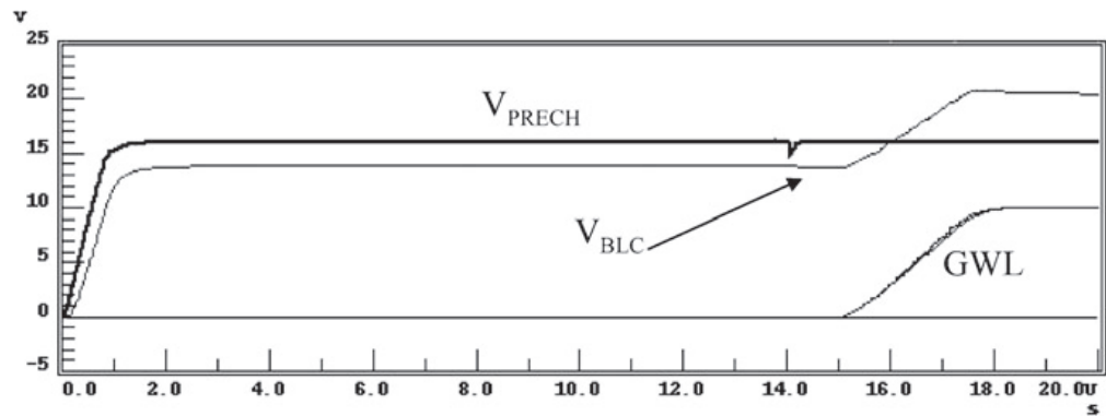
Fig. 6.42 Simulation of the circuit sketched in Fig. 6.39
