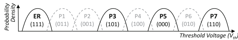
Fig. 9.34 States used when a TLC cell (with 8 states) is downgraded to an MLC cell (with 4 states). Reproduced from [15]
