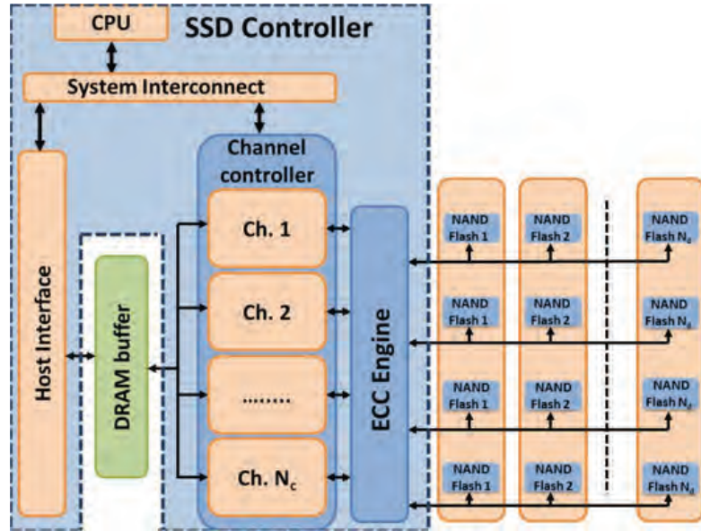
Fig. 7.7 Schematic representation of the SSD controller, considering N_c channels and N_d memory dies connected to each channel. Reproduced with permission from L. Zuolo, C. Zambelli, R. Micheloni and P. Olivo, “Solid-State Drives: Memory Driven Design Methodologies for Optimal Performance”, in Proceedings of the IEEE, vol. 105, no. 9, pp. 1589–1608, Sept 2017. © 2017 IEEE
