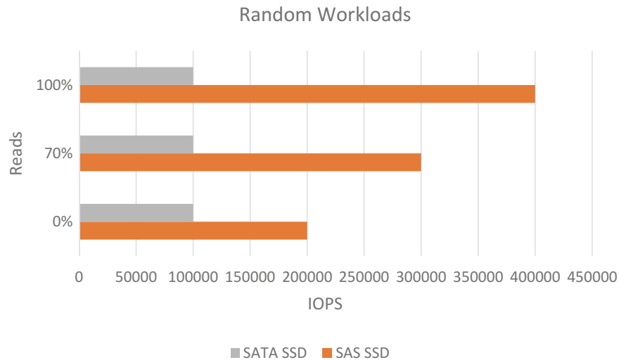
Fig. 2.8 SAS versus SATA under random workloads
