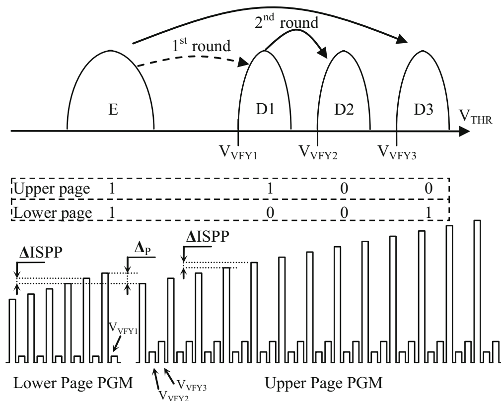
Fig. 6.33 Two rounds MLC program operation
