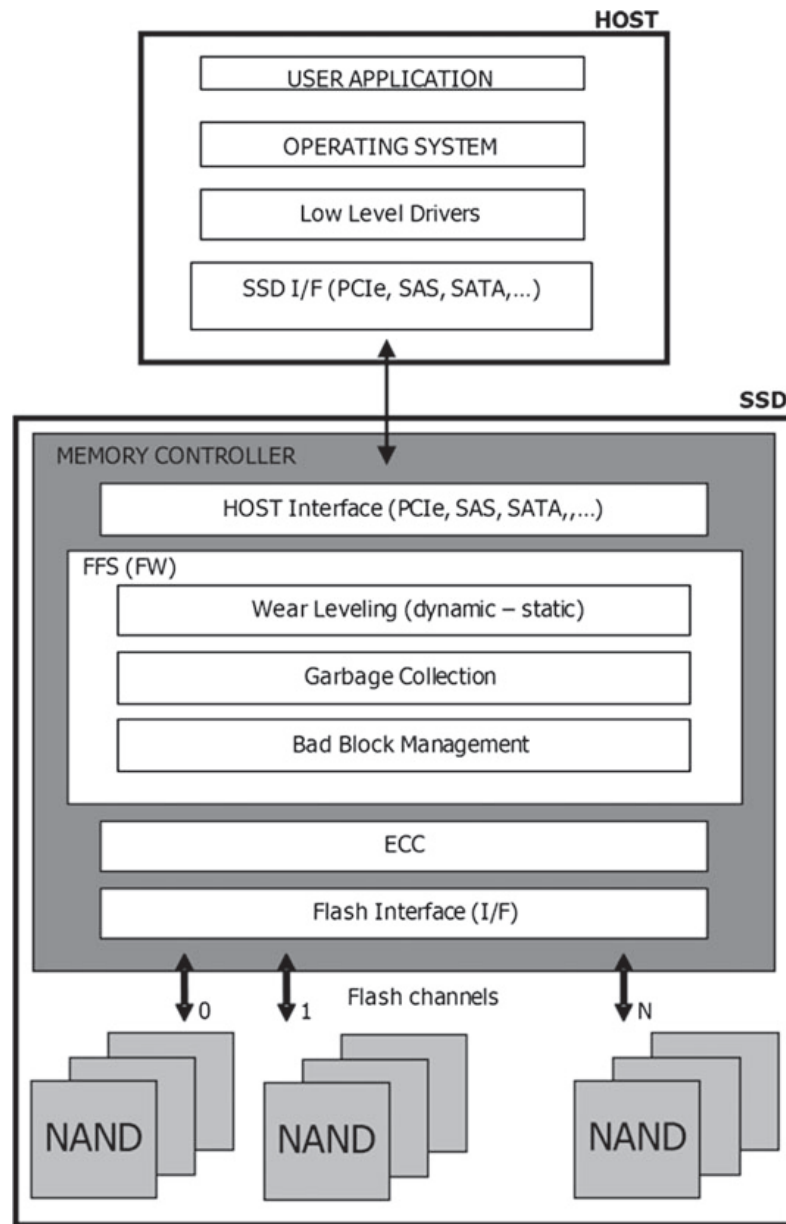
Fig. 1.9 High level view of a flash controller
