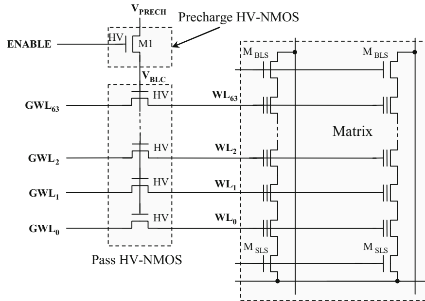
Fig. 6.41 All-NMOS wordline driver
