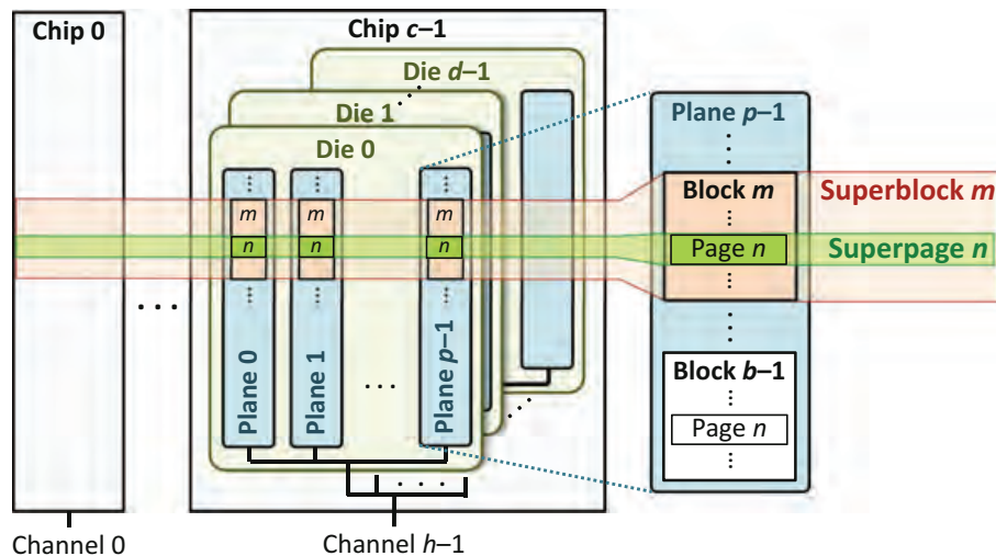
Fig. 9.2 Flash memory organization. Reproduced from [15]
