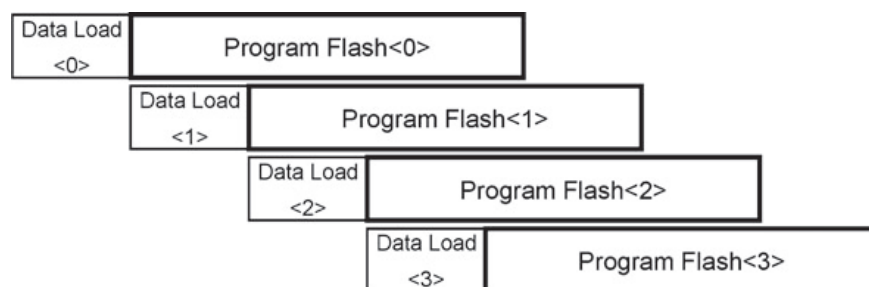
Fig. 1.13 Interleaved operations on one flash channel
