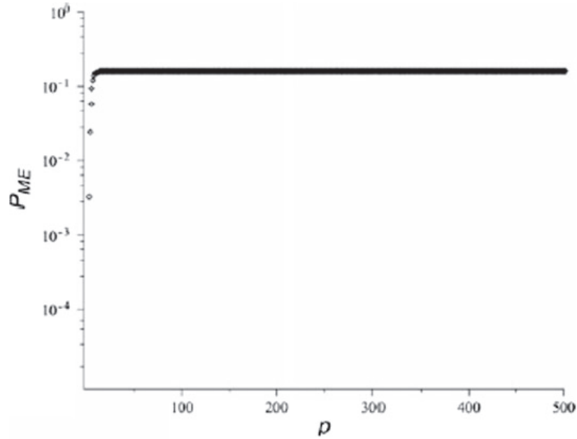
Fig. 11.13 P_{ME} behavior for BCH[1023,993,7]
