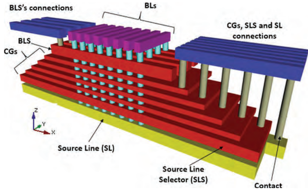
Fig. 5.7 Fan-out of the BiCS array
