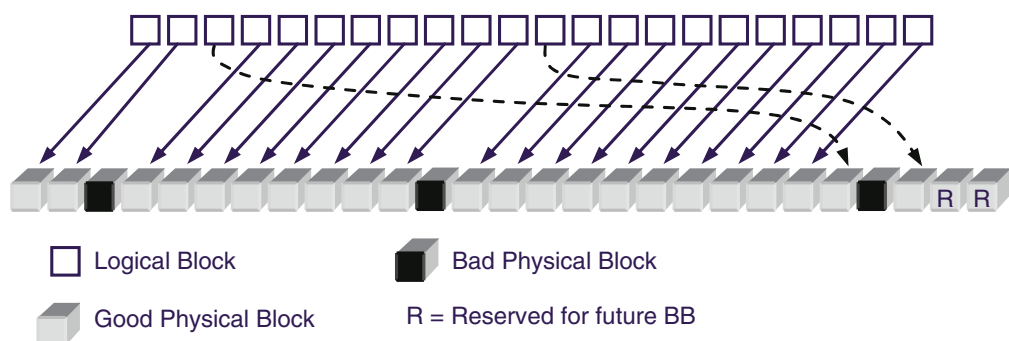
Fig. 1.12 Bad block management (BBM)
