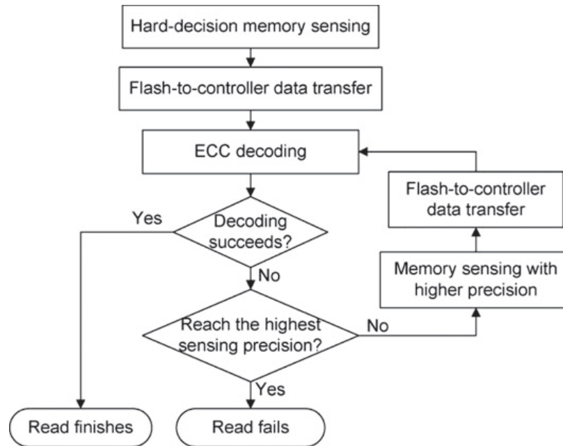
Fig. 8.8 Illustration of operational flow of progressive soft-decision sensing. Reproduced with permission from [30]. © 2013 IEEE
