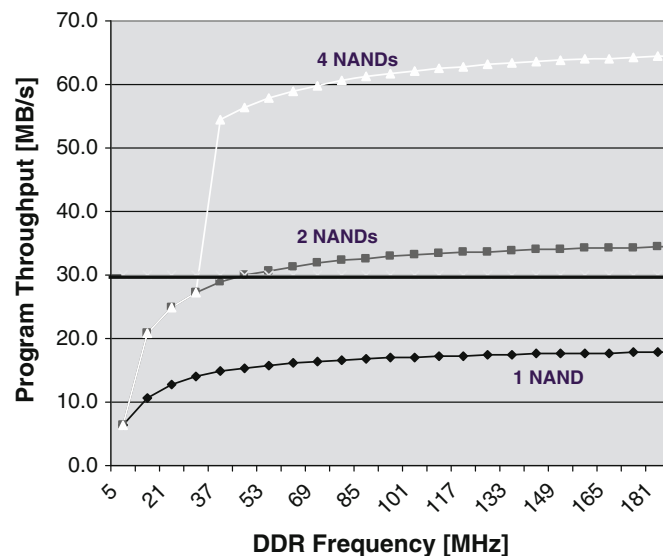
Fig. 1.15 Program throughput with an interleaved architecture as a function of the channel DDR frequency. 4 kB page program time is 200 μs
