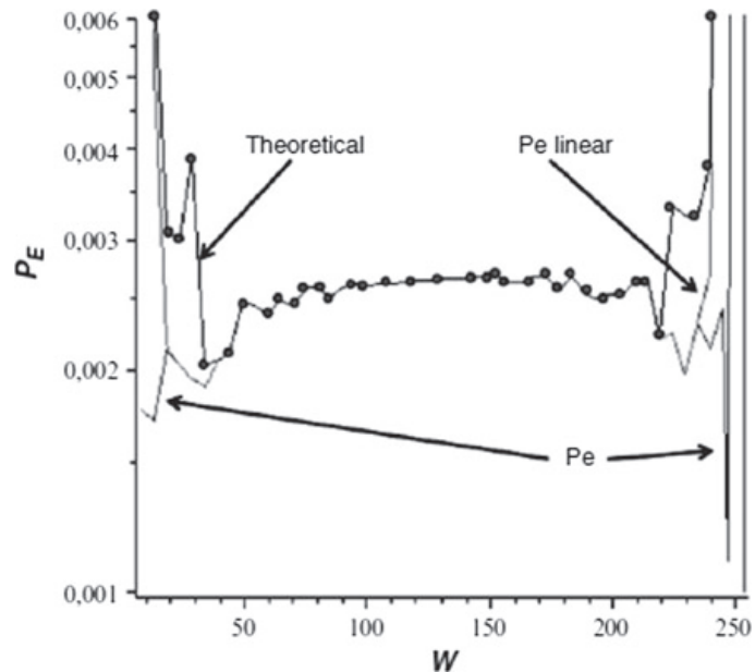
Fig. 11.9 P_E behavior for BCH[255,207,13]. The graph shows the real P_E , the one obtained with linear programming technique and the one obtained by taking the minimum among all the theoretical estimations
