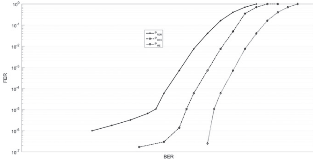
Fig. 11.29 FER versus BER curve for LDPC code
