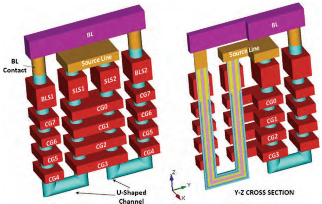
Fig. 5.8 P-BICS NAND strings
