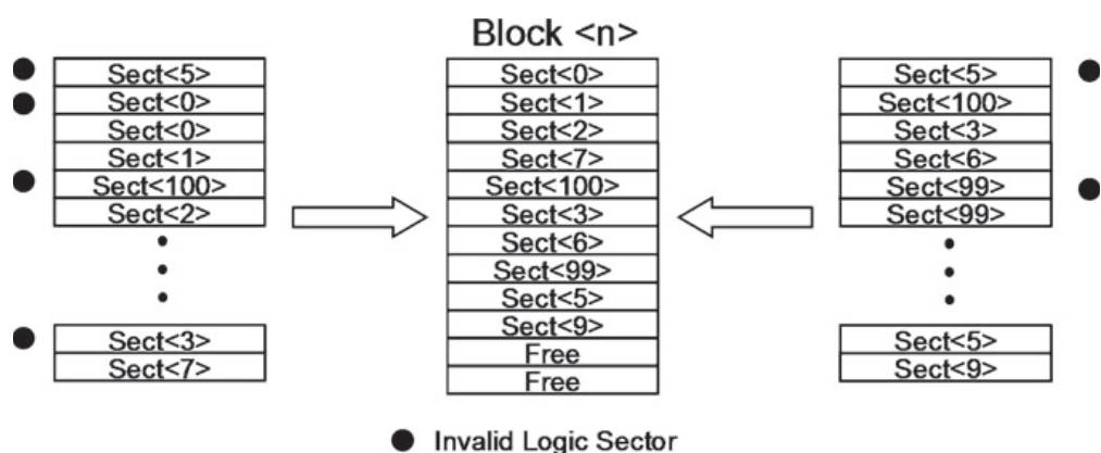
Fig. 1.11 Garbage collection
