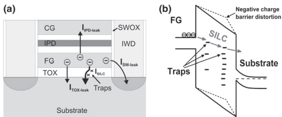
Fig. 4.16 Possible leakage path for charge loss from the floating gate (a). Tunnel oxide damage due to program/erase cycling and the resulting stress-induced leakage current (SILC) are usually the main reasons for retention loss (a, b). Negative trap charge built up over cycling additionally induces a barrier distortion which results in an increased tunnel barrier (b) [12]
