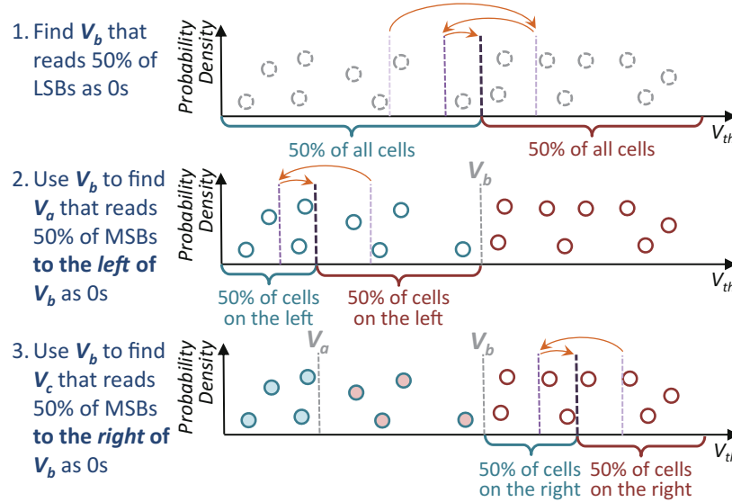
Fig. 9.28 Disparity-based read reference voltage approximation to find V_{initial} for MLC NAND flash memory. Each circle represents a cell, where a dashed border indicates that the LSB is undetermined, a solid border indicates that the LSB is known, a hollow circle indicates that the MSB is unknown, and a filled circle indicates that the MSB is known. Reproduced from [15]
