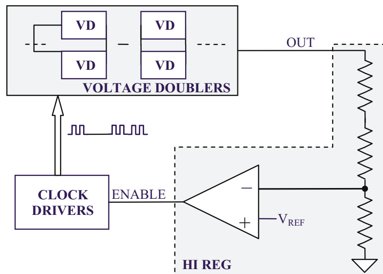
Fig. 6.37 Charge pump architecture
