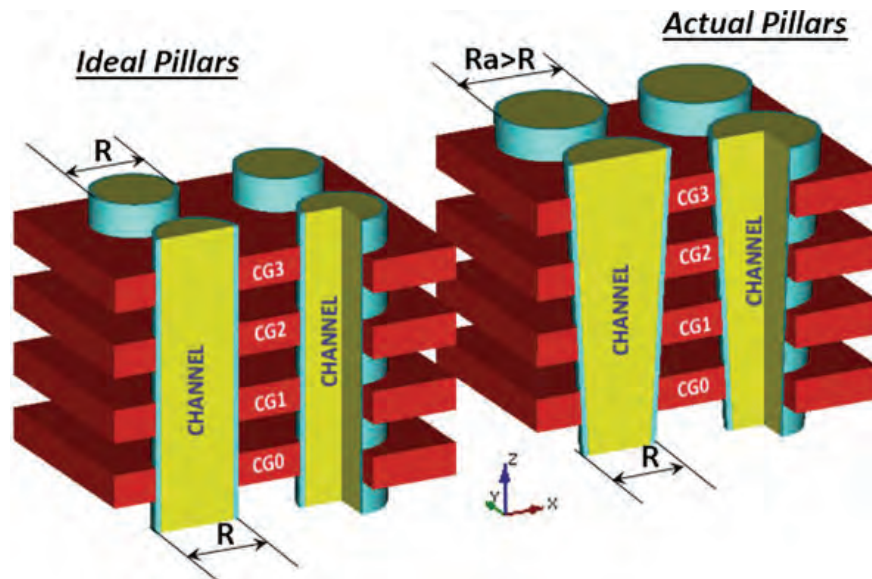
Fig. 5.16 Ideal versus actual shape of pillars
