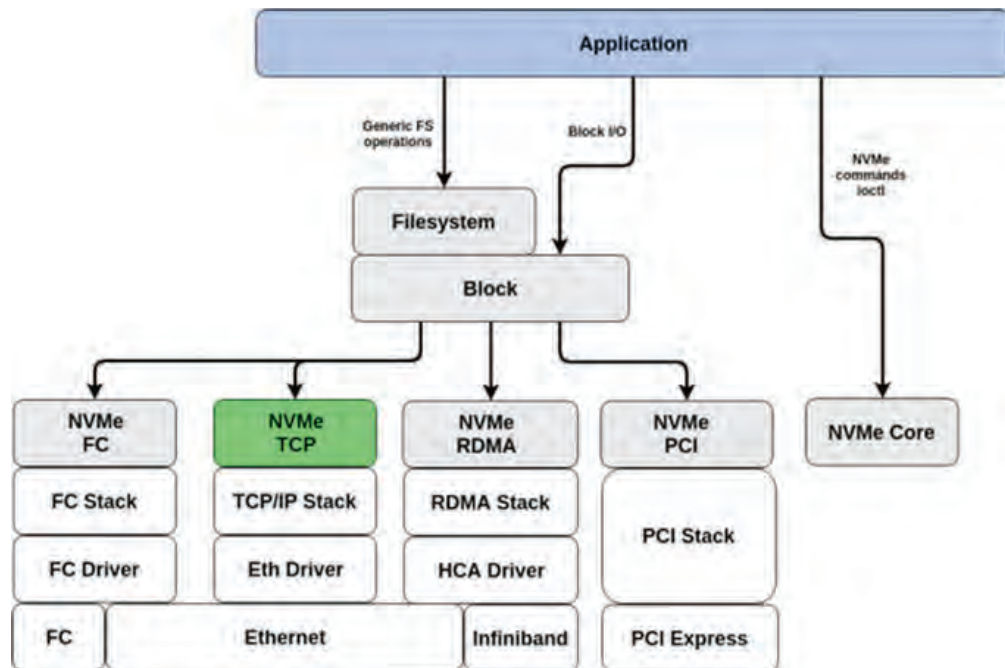
Fig. 1.28 Different types of fabric transports for NVMe
