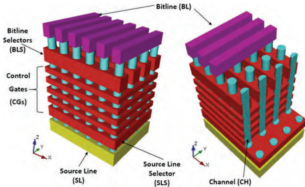
Fig. 5.3 BiCS architecture
