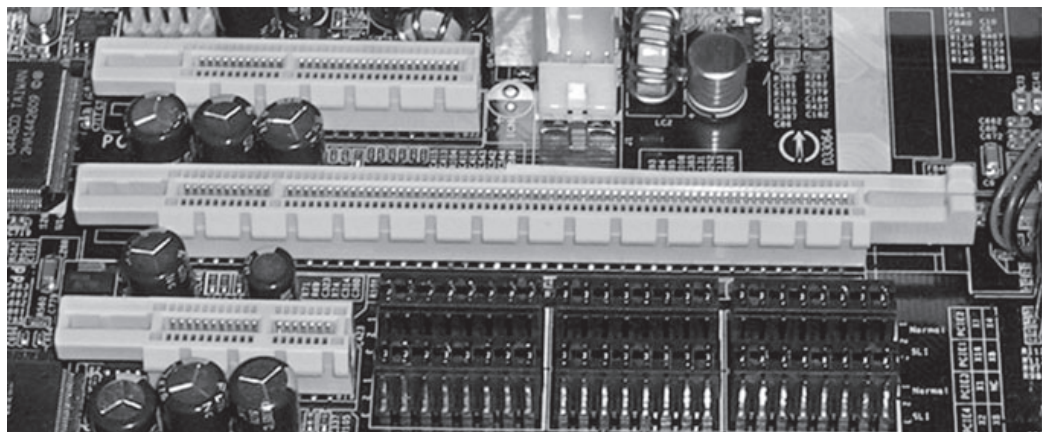
Fig. 1.17 Various PCIe slots. From top to bottom: PCIe \times 4 , PCIe \times 16 , PCIe \times 1
