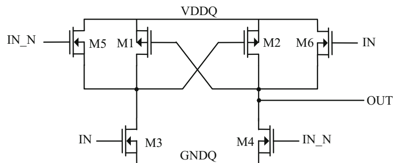
Fig. 6.18 Level shifter modified
