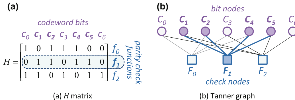
Fig. 9.36 Example LDPC code for a seven-bit codeword with a four-bit data message (stored in bits c_0 , c_1 , c_2 , and c_3 ) and three parity check equations (i.e., n = 7 , k = 4 ), represented as a an H matrix and b a Tanner graph
