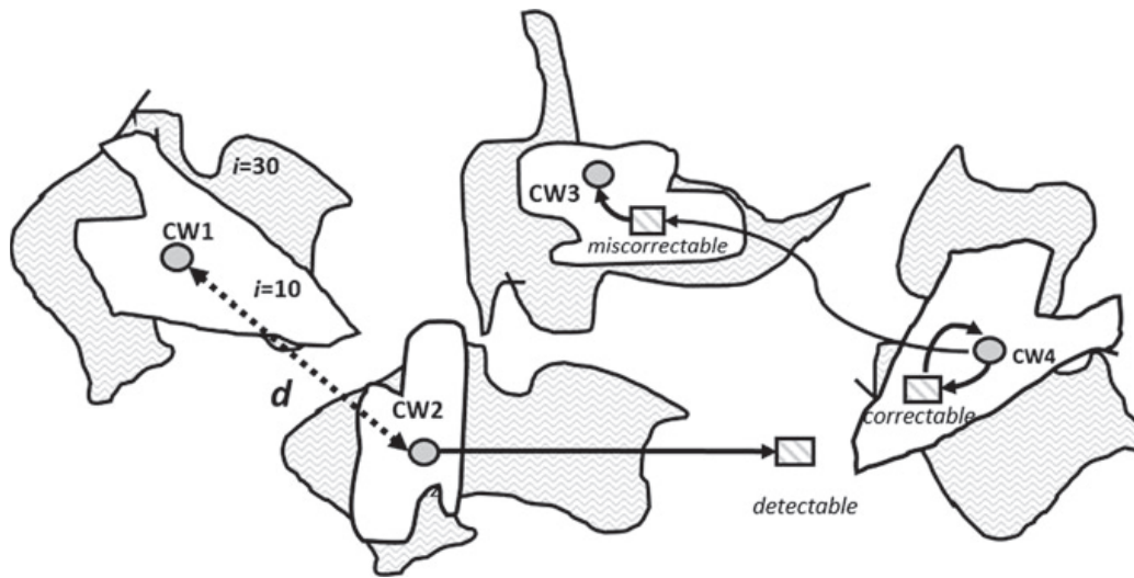
Fig. 11.27 Correction areas for hard LDPC belief propagation decoding algorithm
