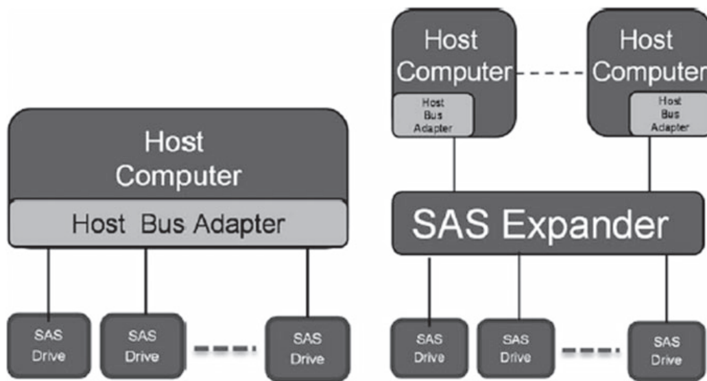
Fig. 2.2 SAS connectivity
