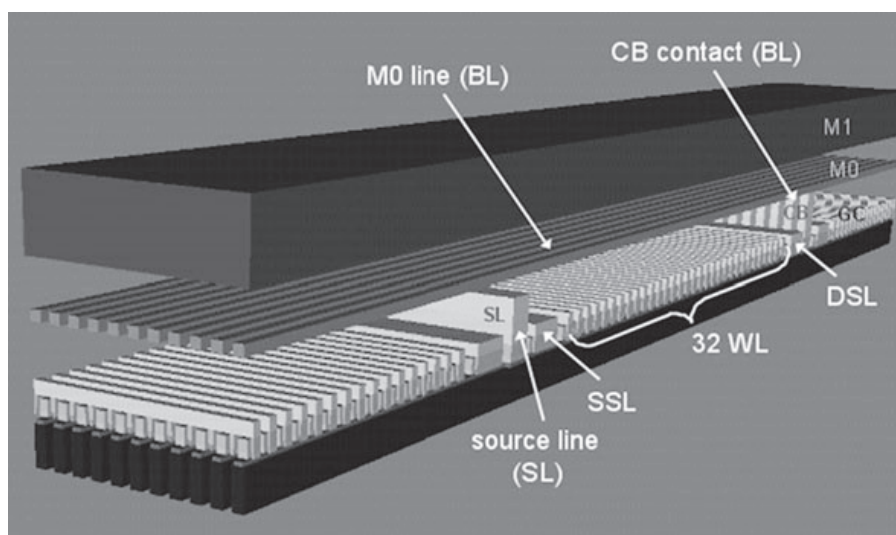
Fig. 1.4 NAND array section along the bitline direction
