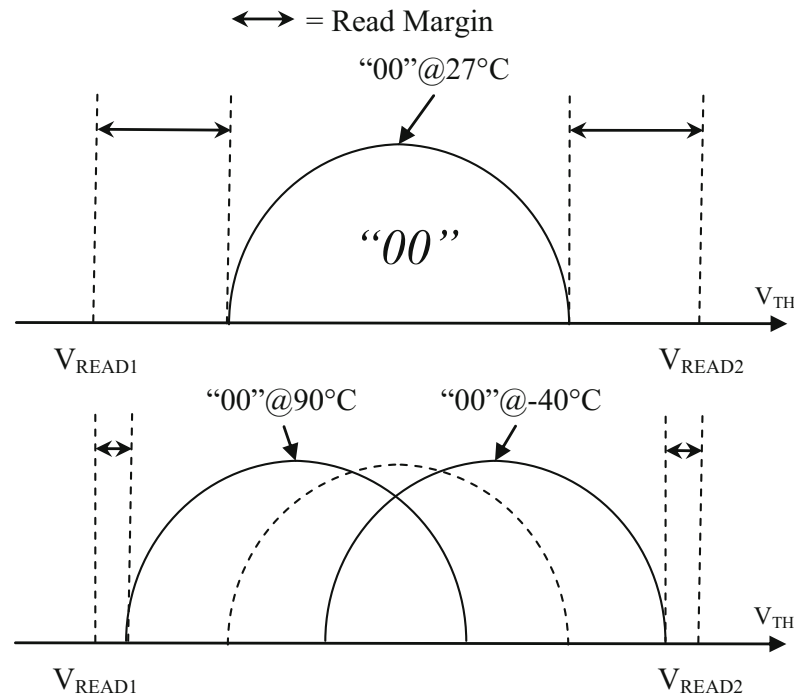
Fig. 6.29 V_{TH} variations with temperature
