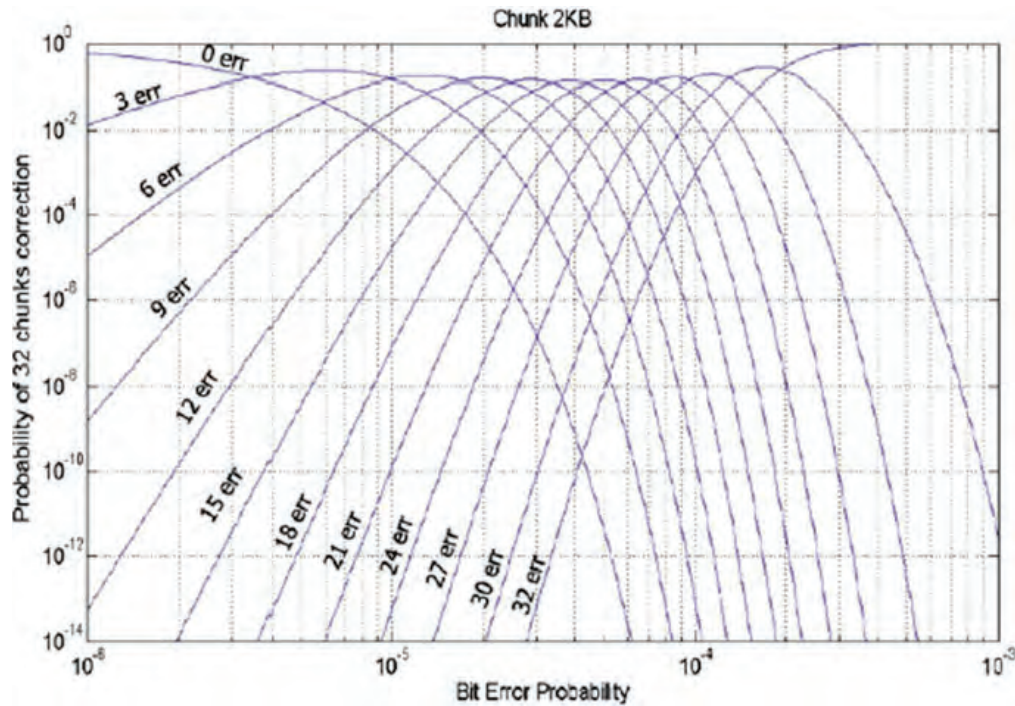
Fig. 11.23 Probability of n chunks over 32 requiring correction
