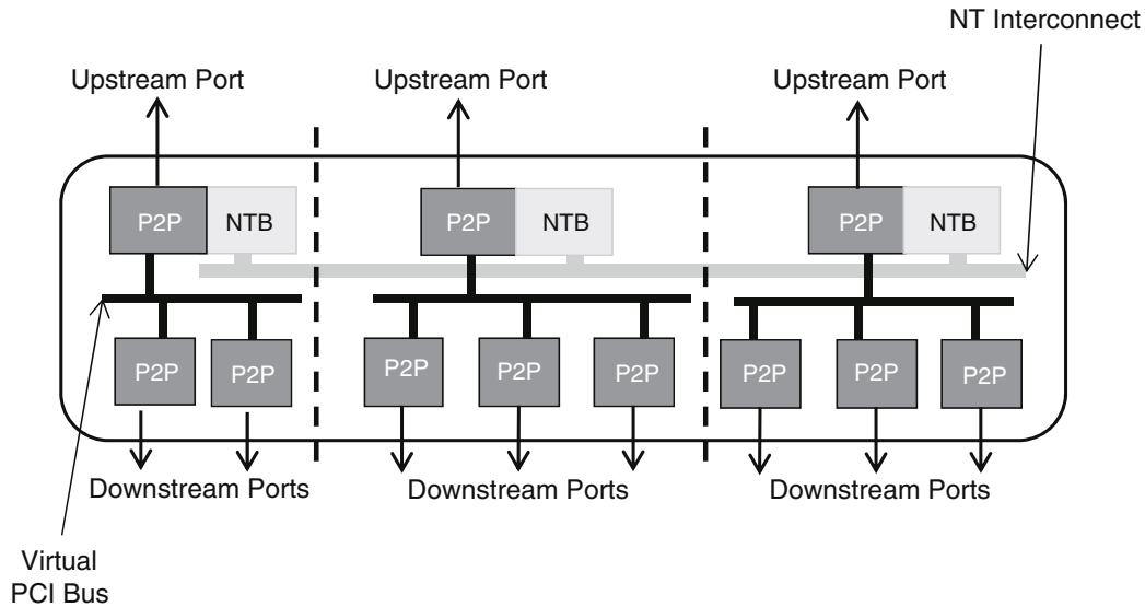
Fig. 1.19 PCIe switch with multiple NTB functions
