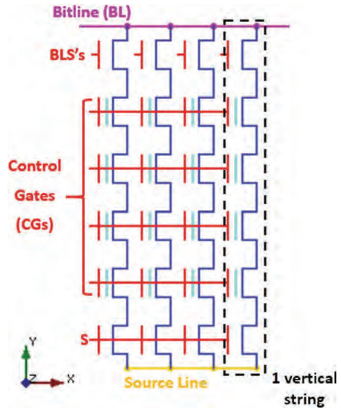
Fig. 5.4 Equivalent circuit of a BiCS array
