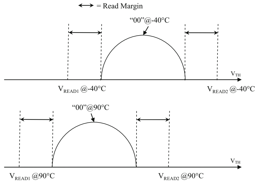
Fig. 6.30 V_{\text{READ}} tracking of V_{\text{TH}} variations with temperature
