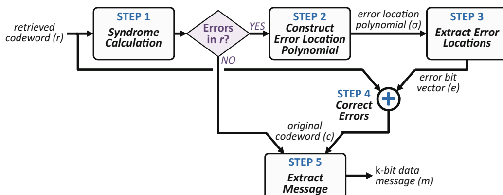
Fig. 9.35 BCH decoding steps
