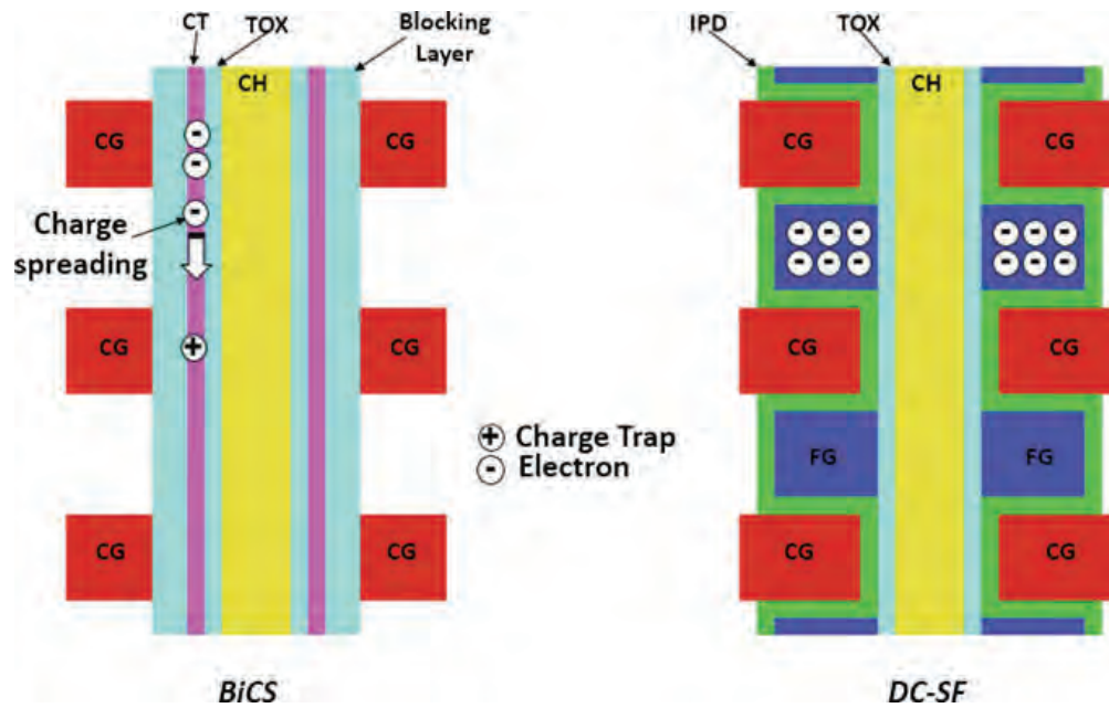
Fig. 5.24 BiCS versus DC-SF
