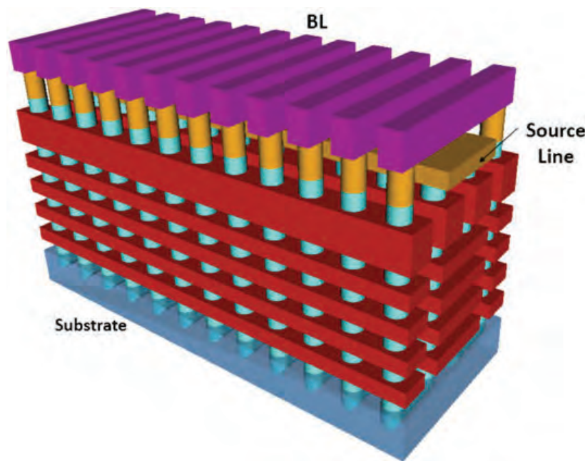
Fig. 5.9 P-BICS NAND Flash array
