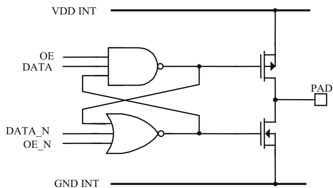
Fig. 6.14 Pre-driver to avoid crowbar in push-pull stage
