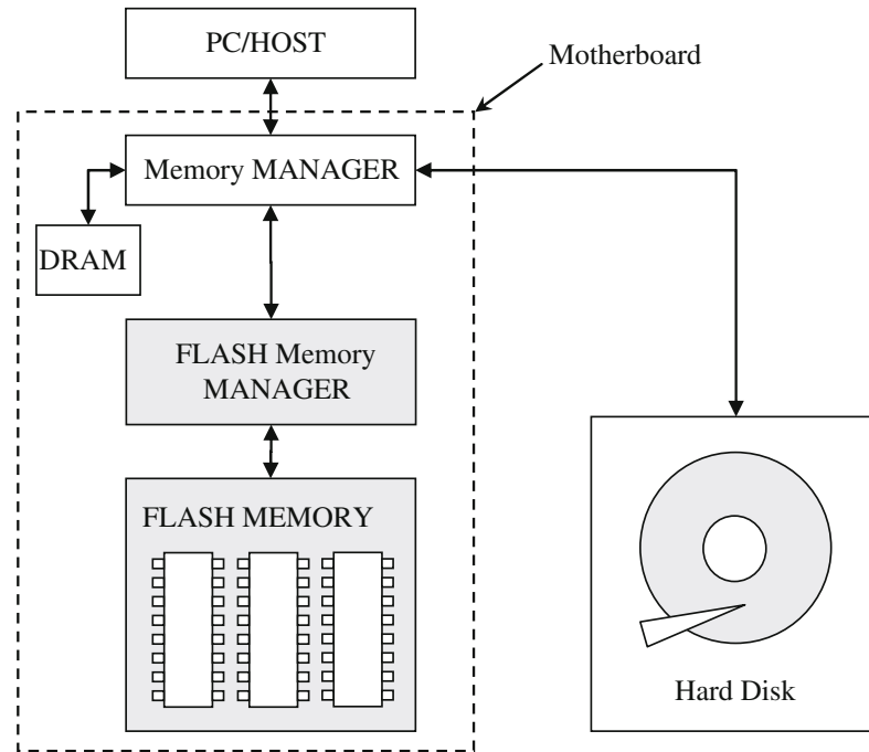
Fig. 3.5 Flash on computer motherboard
