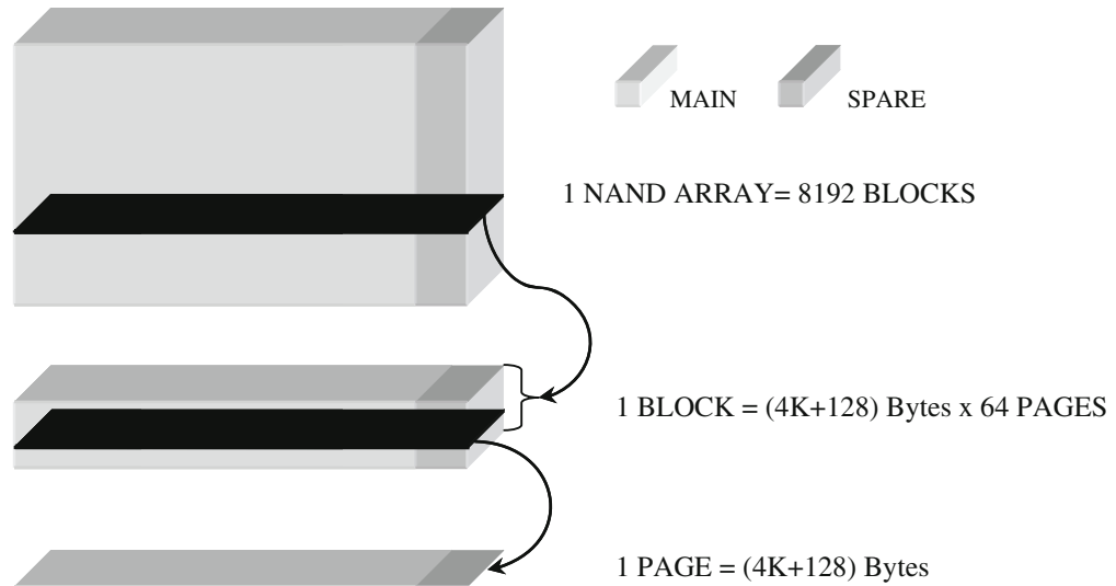
Fig. 1.5 32 Gbit memory logic organization
