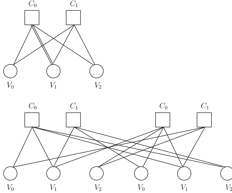
Fig. 12.9 Conceptual example of copy-and-permute protograph procedure
