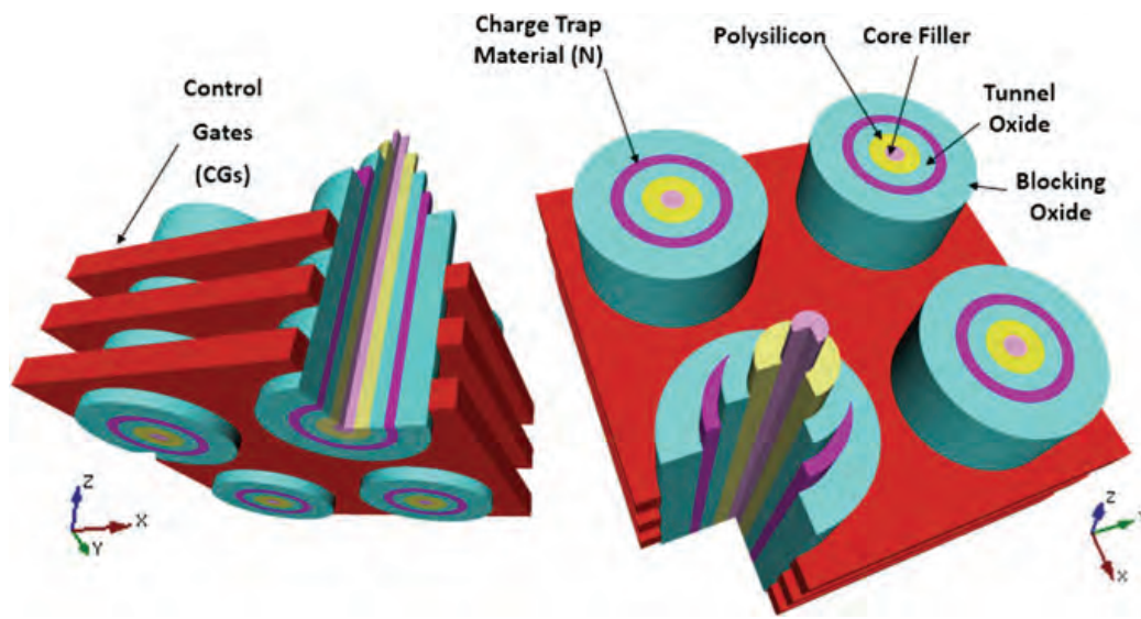
Fig. 5.5 BiCS memory cells
