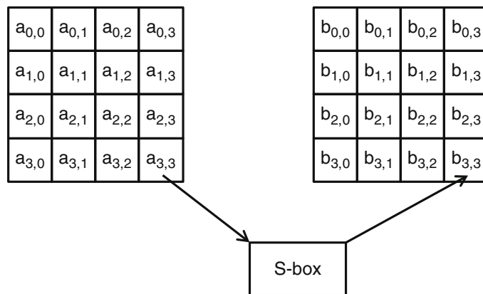
Fig. 13.19 Representation of the SubBytes operation
