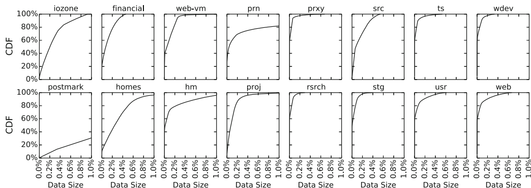
Fig. 9.30 Cumulative distribution function of the fraction of writes performed by a workload to NAND flash memory pages, for 16 evaluated workloads. For every workload except postmark , over 95% of all writes performed by the workload are destined for less than 1.0% of the workload's pages. Total data footprint of each workload is 217.6 GB, i.e., 1.0% on the x-axis represents 2.176 GB of data. Reproduced from [161]
