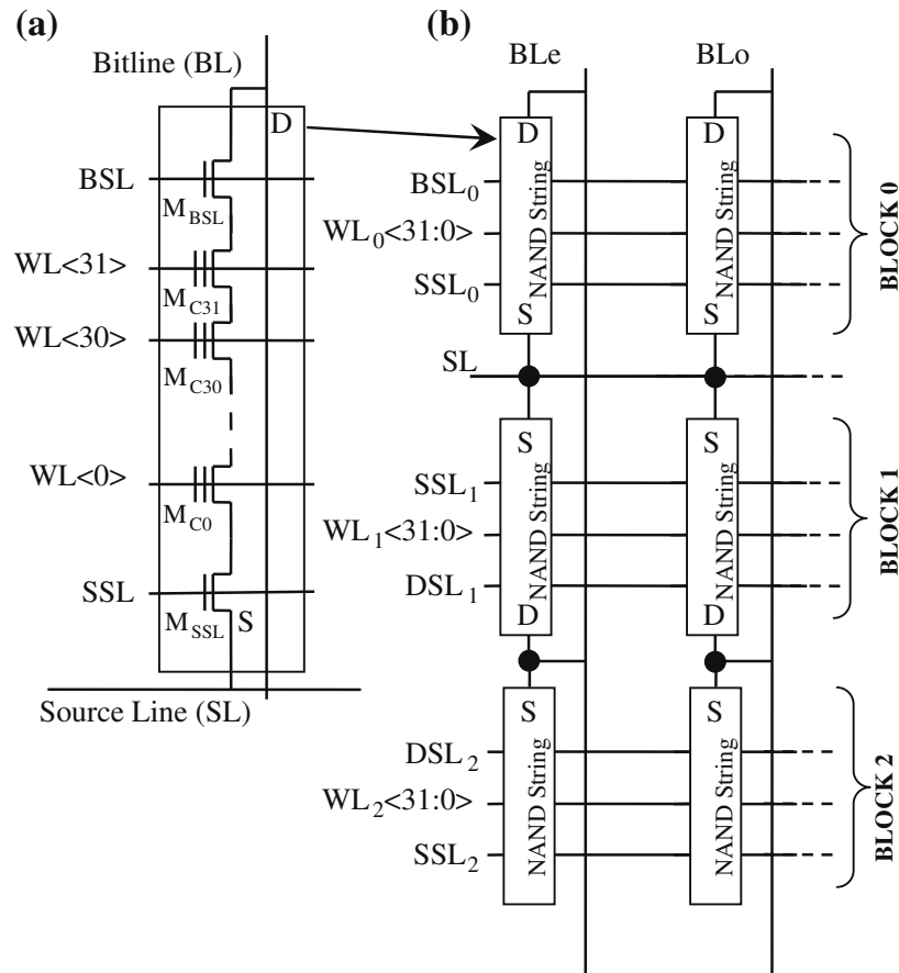
Fig. 1.3 NAND String (a) and NAND array (b)
