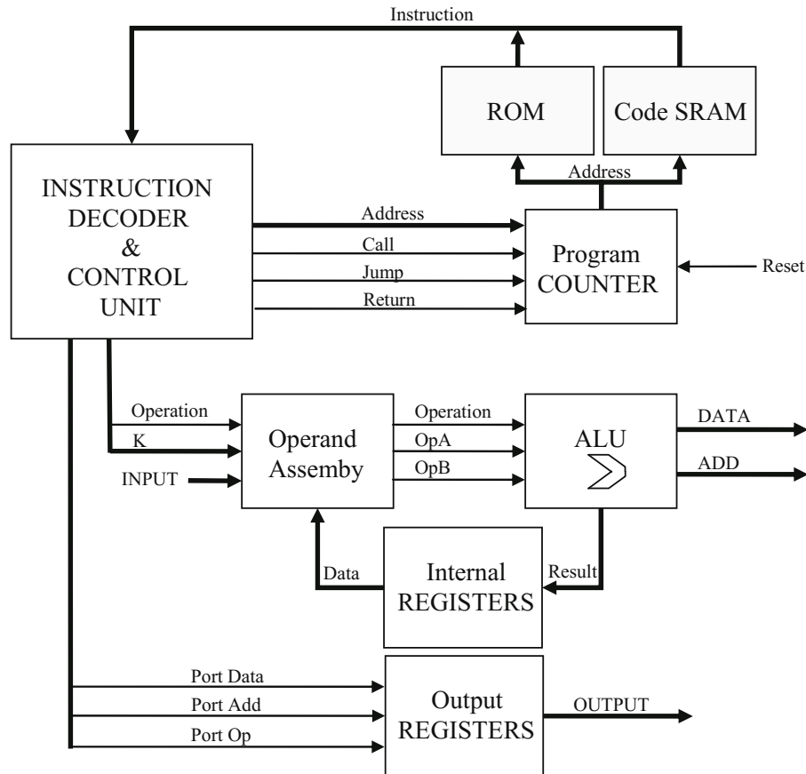
Fig. 6.7 Microcontroller structure with ROM and RAM memories
