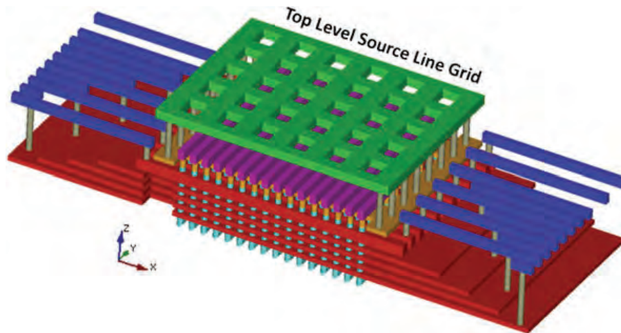
Fig. 5.11 P-BiCS: source line metal mesh
