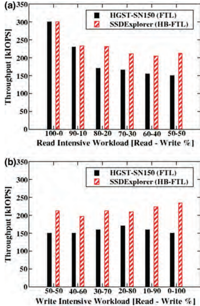
Fig. 7.12 Throughput (expressed in kIOPS) of HGST SN150 Ultrastar SSD architecture compared to that of a simulated HB-FTL-based drive with the same configuration: (top) read intensive and (bottom) write intensive workloads. A queue depth of 32 commands is used. Simulations have been performed with SSDExplorer [22]. Reproduced with permission from L. Zuolo, C. Zambelli, R. Micheloni and P. Olivo, “Solid-State Drives: Memory Driven Design Methodologies for Optimal Performance”, in Proceedings of the IEEE, vol. 105, no. 9, pp. 1589–1608, Sept 2017. © 2017 IEEE
