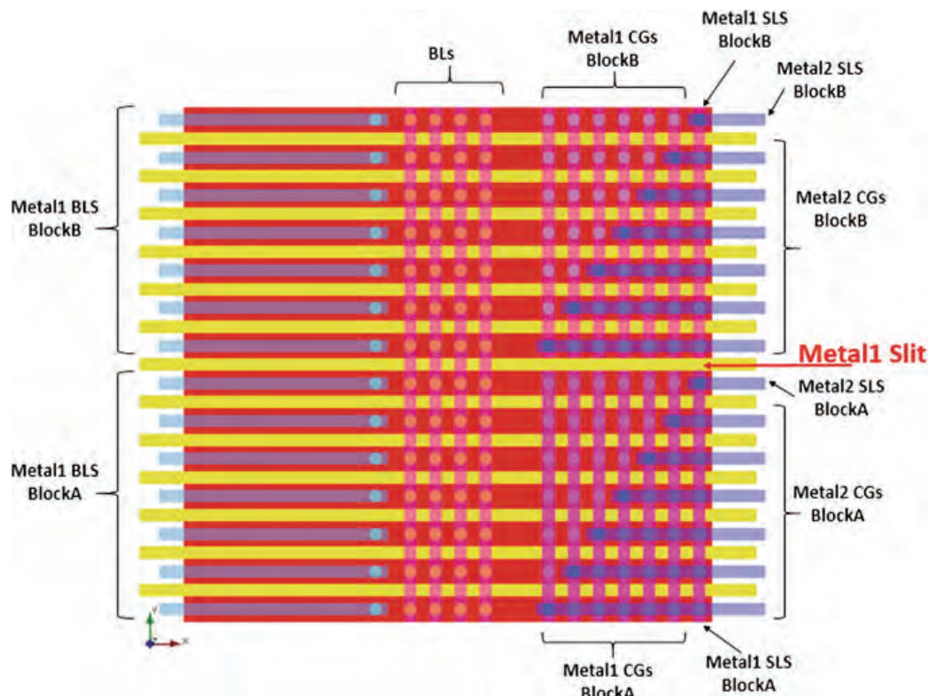
Fig. 5.13 Top view of Fig. 5.12
