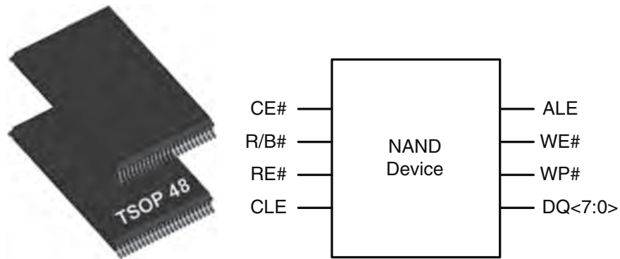
Fig. 1.6 TSOP package ( left ) and related pinout ( right )
