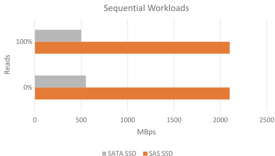
Fig. 2.9 SAS versus SATA under sequential workloads
