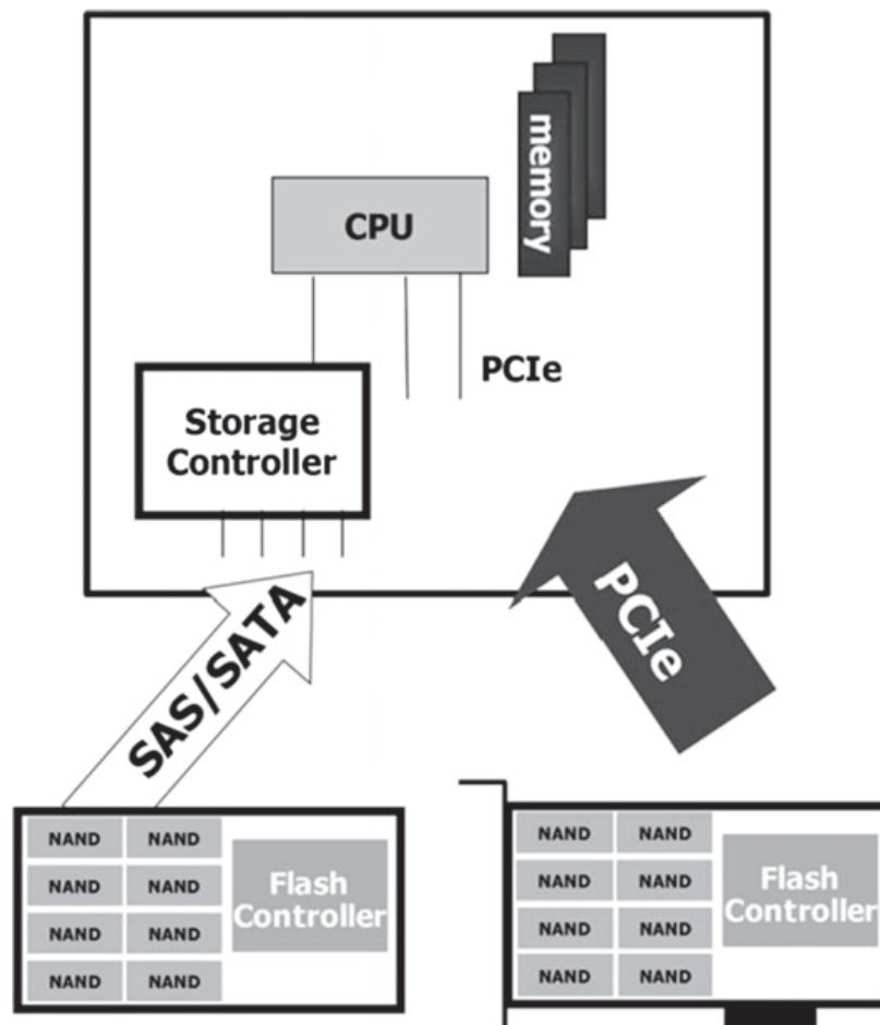
Fig. 1.24 PCIe SSD versus SAS/SATA SSD
