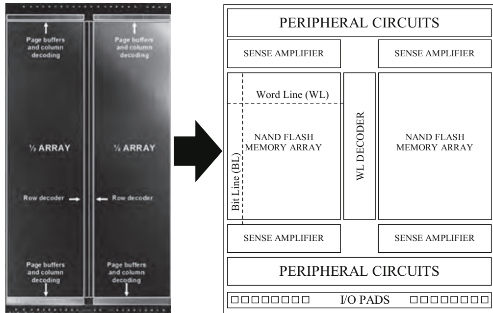
Fig. 6.1 A typical NAND Flash floorplan [1]
