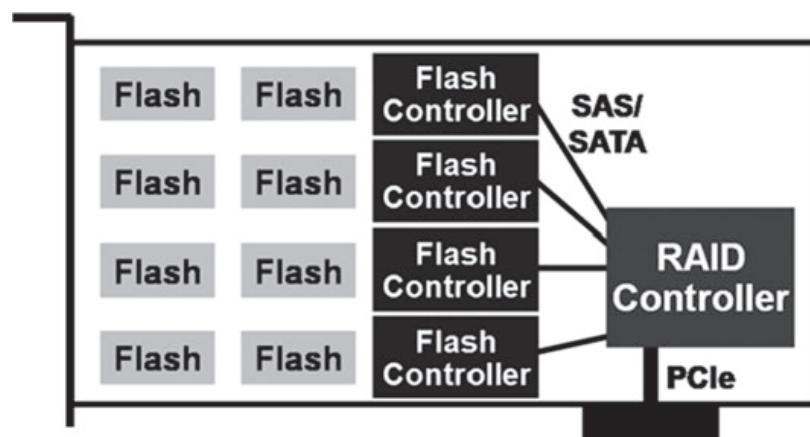
Fig. 1.25 RAID-based PCIe SSDs not optimized for performance/power
