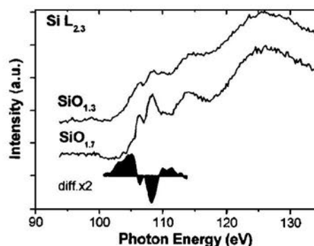
FIG. 5. \text{Si } L_{2,3} absorption spectra of \text{SiO}_x thin films with different O/Si ratios. The shadowed curve corresponds to the difference spectra between the two plots.
