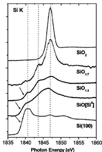
FIG. 6. Si K-edge absorption spectra of \text{SiO}_x thin films of the indicated O/Si ratios. Sample \text{SiO}[\text{Si}^0] corresponds to a \text{SiO}_{1.3} thin film heated at 750 K for 3 h under vacuum.
