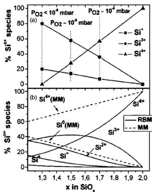
FIG. 1. (a) Distribution of \text{Si}^{n+} species as a function of the oxygen content determined experimentally for \text{SiO}_x thin films prepared by evaporation. (b) Distribution of \text{Si}^{n+} species as a function of the oxygen content predicted by the MM and RBM.
