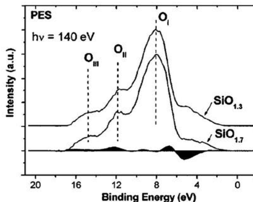
FIG. 3. PES spectra ( h\nu = 140 eV) of two SiO x thin films with different O/Si ratios. The shadowed curve corresponds to the difference spectra between the two plots.
