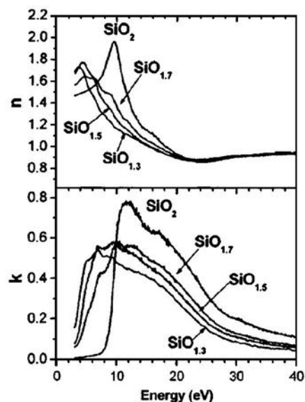
FIG. 10. n and k functions derived from the REELS spectra for the indicated \text{SiO}_x samples.
