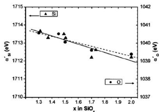
FIG. 2. Evolution of the Auger parameters of Si and O as a function of the oxygen content in \text{SiO}_x thin films prepared by evaporation.
