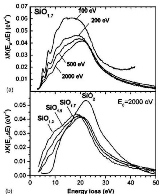
FIG. 7. (a) REELS spectra of sample \text{SiO}_{1.7} recorded with increasing primary energies. (b) REELS spectra recorded with E_0=2000 eV for \text{SiO}_x samples of different stoichiometries.
