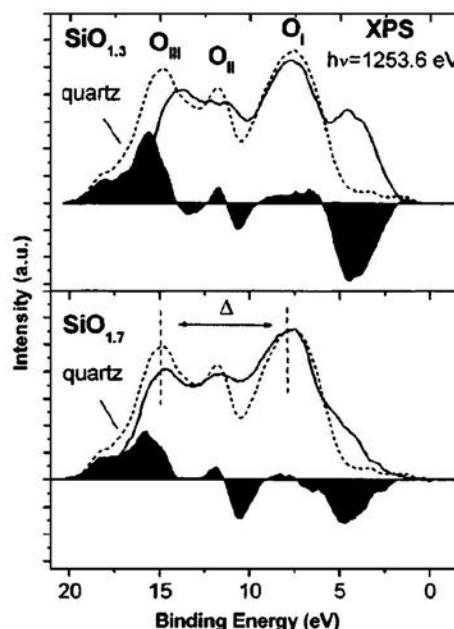
FIG. 4. XPS spectra ( h\nu = 1253.6 eV) of two SiO x thin films with different O/Si ratios. The dashed curve is the spectrum of a fully stoichiometric SiO 2 , while the shadowed curves are the difference spectra between the spectra of SiO x and SiO 2 .
