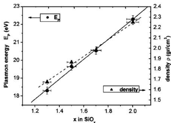
FIG. 8. Position of the bulk plasmon and density of the films determined by means of expression (5) for samples with different O/Si ratios.
