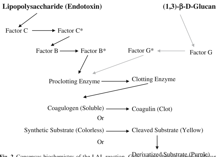
Fig. 2 Consensus biochemistry of the LAL reaction. Only arrows denote alternate glucan-mediated pathway
