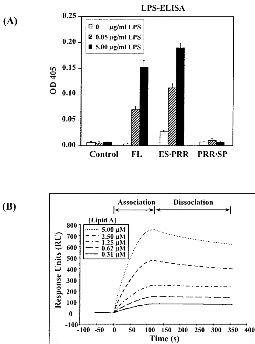
FIG. 4. Functional analysis of FC. A , ligand binding assays of FC samples. ELISA of 10 \mu g each of protein samples: control serum-free medium, FL, ES-PRR, and PRR-SP partially purified through Sephadex G-100 (void fraction). Three concentrations of LPS (0, 0.05, and 5 \mu g/ml) were used. Error bars represent the S.E. ( n = 3 ). B , a sensorgram depicting the interaction (in response units (RU)) of captured FL with various concentrations of lipid A. ES-PRR gave similar response profiles. 100 \mu l of five concentrations (5.00, 2.50, 1.25, 0.62, and 0.31 \mu M) of lipid A were injected. The affinity constants were calculated using the BIAevaluation program version 3.0.2 and reconfirmed using CLAMP (21).
