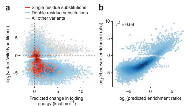
Figure 4 | Prediction of WW domain folding energies and double-mutant enrichment ratios. (a) The Rosetta framework was used to calculate folding energies for 16,363 full-length hYAP65 WW domain variants. Predicted folding energies relative to the wild-type WW domain energy are plotted against the observed fitness (variant/wild type) for the variants containing one, two or more mutations. (b) Using a basis set of single mutant enrichment ratios, we predicted double-mutant enrichment ratios using a product model.
