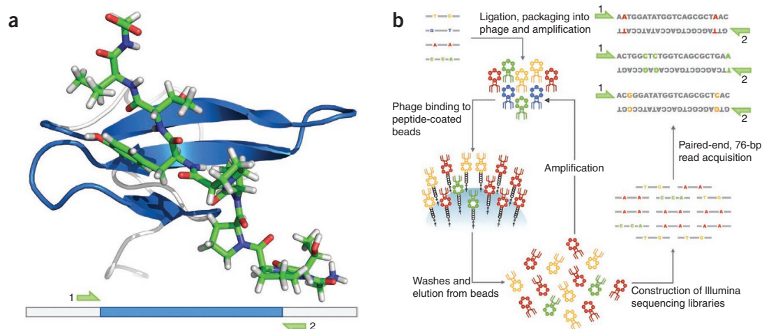
Figure 1 | A highly parallel assay for exploring protein sequence-function relationships. (a) PyMOL software-generated cartoon of the NMR spectroscopy structure of the hYAP65 WW domain (Protein Data Bank identifier 1jmq) in complex with its peptide ligand 16 . The portion of the mutagenized region of the hYAP65 WW domain whose encoding DNA was sequenced is shown in blue. Arrows indicate locations of sequencing primers. (b) A library of sequences encoding variant WW domains was generated using chemical DNA synthesis with doped nucleotide pools, PCR-amplified and displayed as a fusion to T7 capsid protein. The input phage library was subjected to successive rounds of selection. Each round consisted of phage binding to peptide ligand immobilized on beads, washing to remove unbound phage, and elution and amplification of bound phage. Sequencing libraries were created using PCR from input phage and from phage after three and six rounds of selection, and were sequenced using overlapping paired-end reads on the Illumina platform. An example of four unique variants of differing affinity are shown in different colors. Green arrows indicate locations of sequencing primers.
