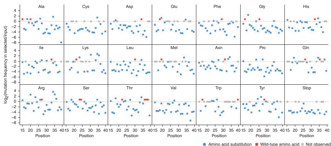
Figure 3 | Comprehensive sequence-function map of the WW domain. We calculated enrichment ratios (round-six/input libraries) for each amino acid at each position in the WW domain. Each plot corresponds to a different amino acid substitution profile as indicated. The x axes indicate position along the WW domain and the y axes indicate \log_2 (enrichment ratio). Blue dots indicate a measured enrichment ratio and red dots indicate the wild type sequence, which enriched 1.7-fold. Gray dots indicate mutations not observed and were arbitrarily placed at zero. The alanine plot corresponds to a traditional alanine scan of the WW domain.
