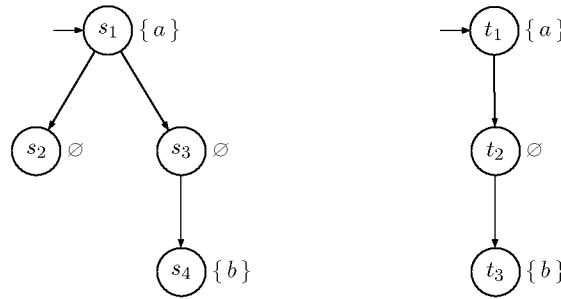
Figure 7.26: TS_1 \preceq TS_2 , but Traces(TS_1) \not\subseteq Traces(TS_2) .
