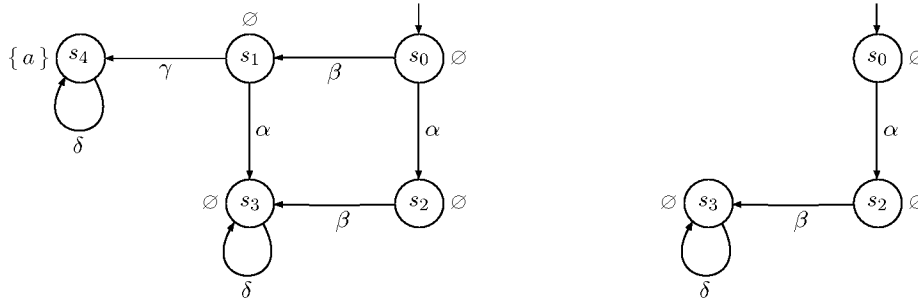
Figure 8.8: A possible, though unsound reduction that satisfies (A2') but not (A2).
