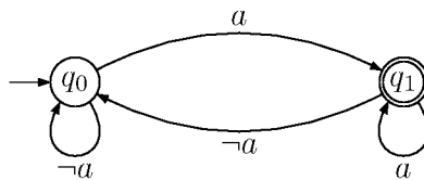
Figure 10.9: A DBA for \Box\Diamond a .
