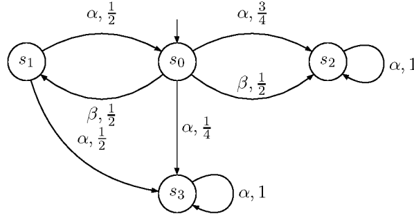
Figure 10.20: Example MDP for max reachability.
