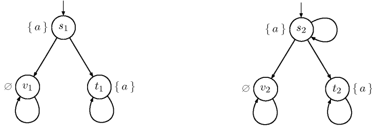
Figure 7.28: TS_1 \preceq TS_2 , but TS_2 \not\preceq TS_1 .
