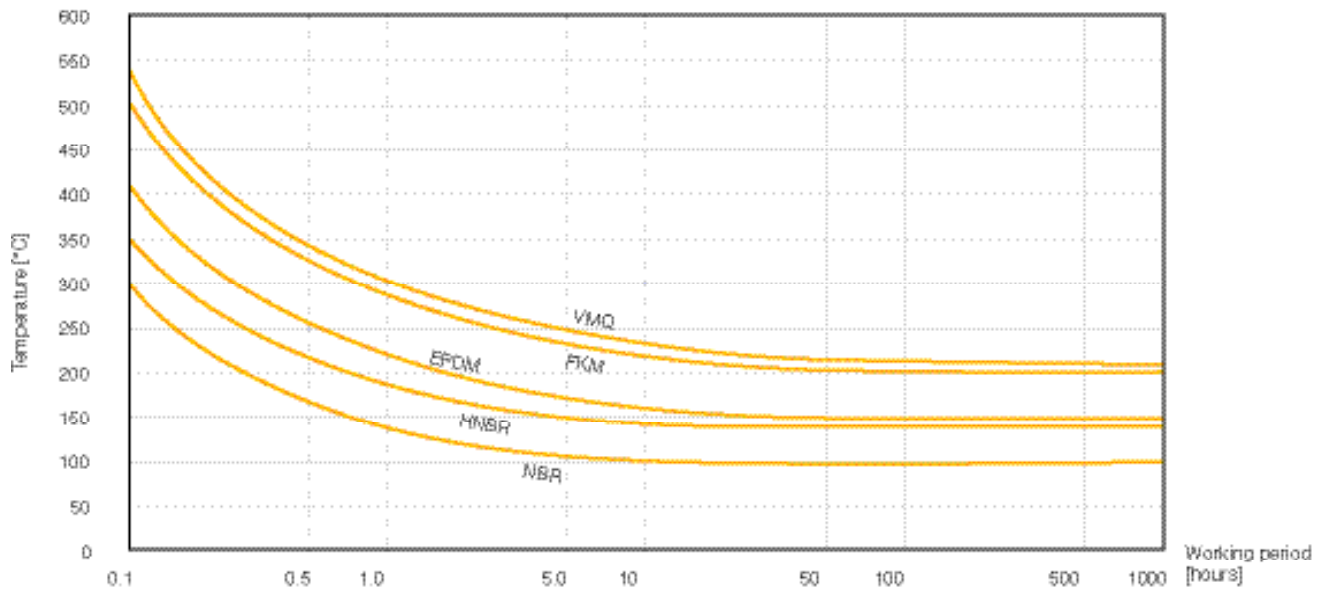
Fig. 7.1 High-temperature limits for various elastomeric materials
