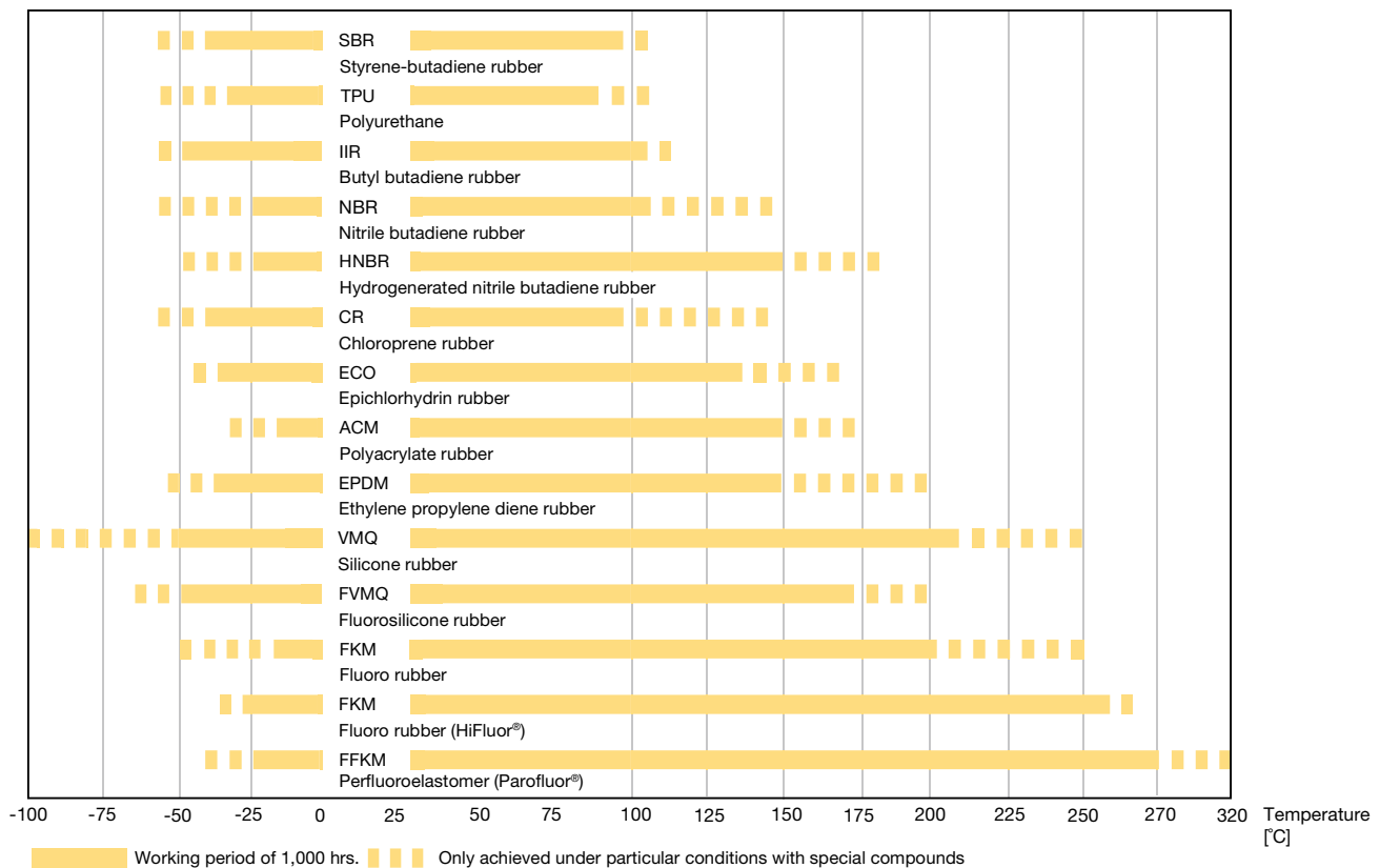
Fig. 7.1 High-temperature limits for various elastomeric materials
