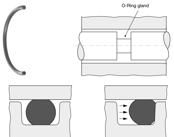
Fig. 1.1 O-ring deformation through system pressure
