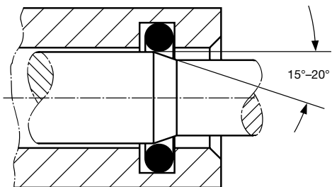
Fig. 2.23 Assembly example of rod
