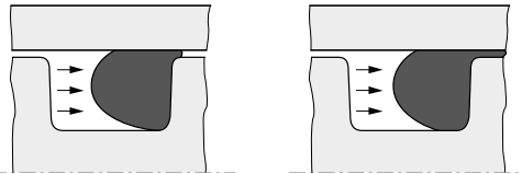
Fig. 10.3 At higher pressure a larger O-ring volume is pushed into the gap. A back-up ring prevents gap extrusion.
