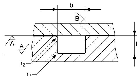
Fig. 7.6 Dimensions of vacuum gland, static application
