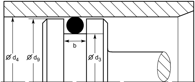
Fig. 3.13 Piston seal – radial compression
