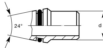
Fig. 4.2 Threaded fitting with 24° conical seal face: form A for welded connector
