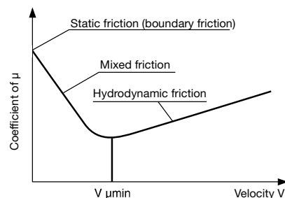
Fig. 8.18 Stribeck curve
