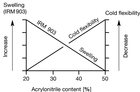
Fig. 6.3 Influence of the acrylonitrile content
