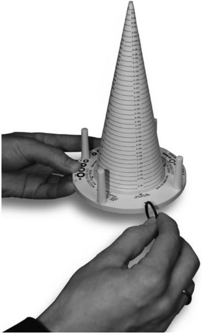
Fig. 5.7 Determination of the cross-section
