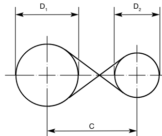
Fig. 2.20 Crossed design
