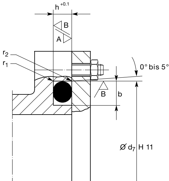
Fig. 2.8 Pressure from inside
