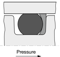
Fig. 10.4 The back-up ring on the non-pressurised side prevents gap extrusion.
