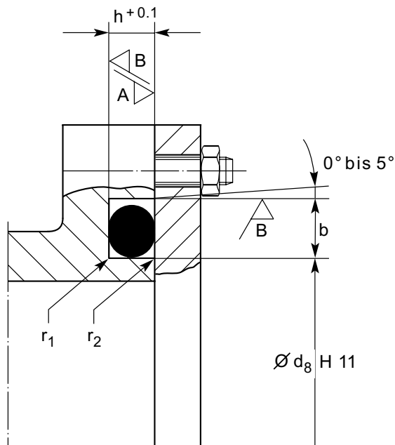
Fig. 2.9 Pressure from outside
