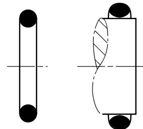
Fig. 8.12 left: unstretched O-ring, right: stretched O-ring
