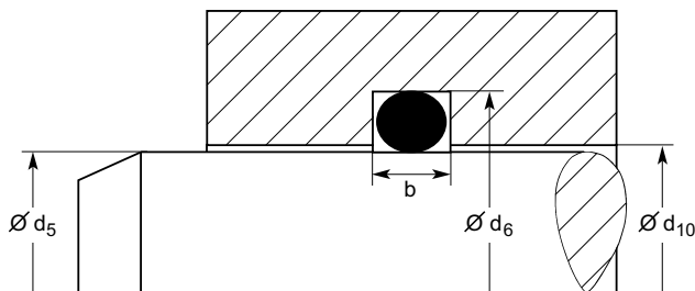
Fig. 3.2 Rod seal – radial compression
