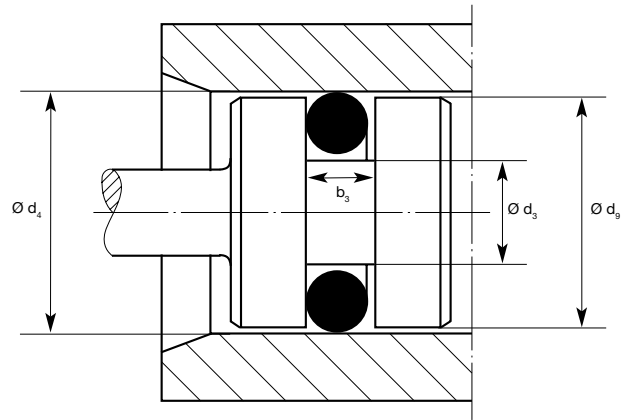
Fig. 3.15 Floating design – no compression
