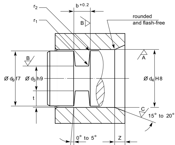
Fig. 2.15 Piston seal – hydraulic and pneumatic
