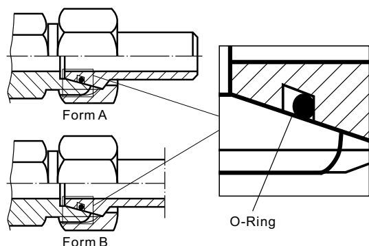
Fig. 4.4 Assembly
