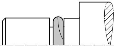
Fig. 2.28 O-ring fitted rolled
