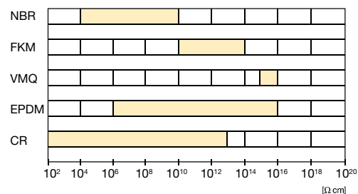
Fig. 8.9 Specific electrical resistance (according to DIN 53596)
