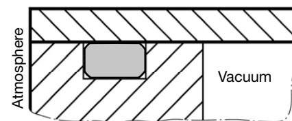
Fig. 7.5 Vacuum O-ring gland
