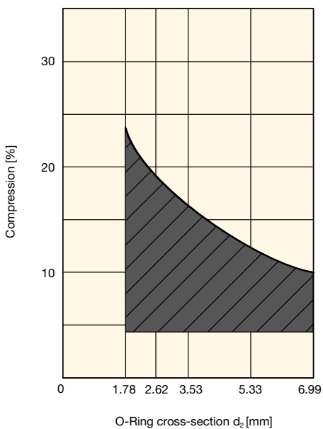
Fig. 8.33 Permissible compression is dependent upon cross-section d_2 – reciprocating seal pneumatic
