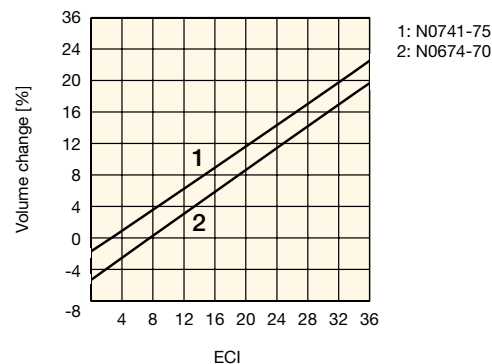
Fig. 8.8 Swelling characteristics of Parker compounds
