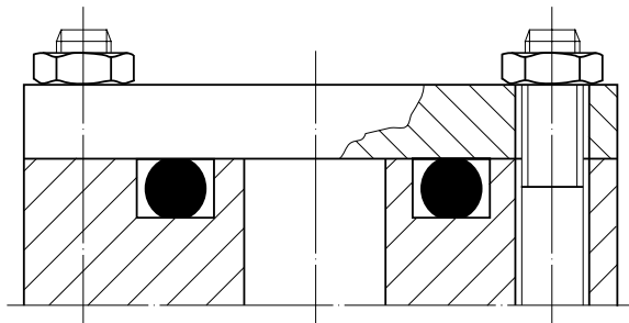
Fig. 2.3 Face seal: O-ring with axial compression
