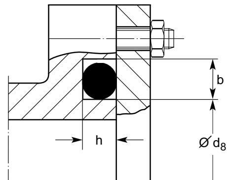
Fig. 3.4 Flange seal – axial compression
