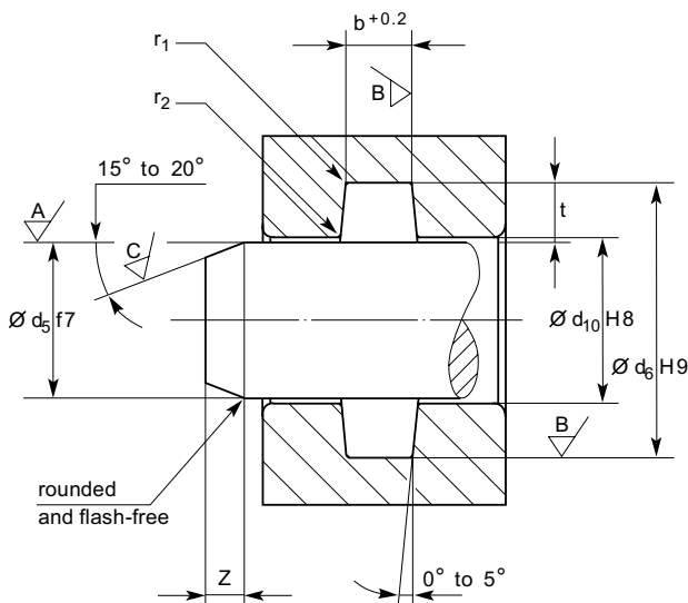
Fig. 2.14 Rod seal – hydraulic and pneumatic
