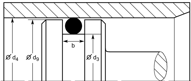
Fig. 3.1 Piston seal – radial compression
