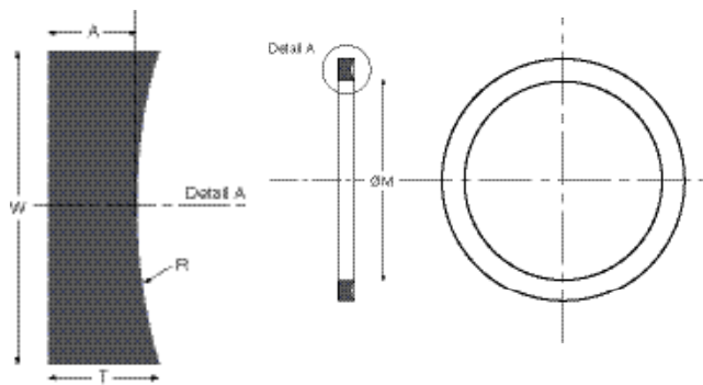
Fig. 4.11 Parbak® back-up ring
