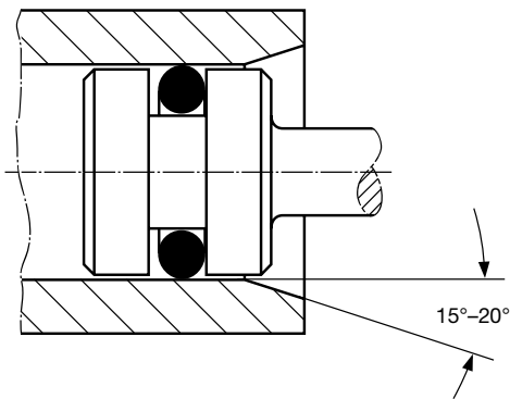
Fig. 2.22 Assembly example of piston
