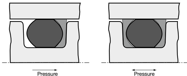
Fig. 4.9 Function of an O-ring-Parbak® combination
