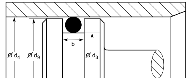
Fig. 3.9 Piston seal – radial compression
