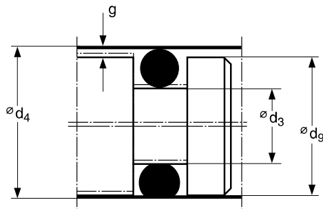
Fig. 8.35 With maximum radial play
