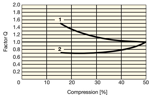
1: dry O-Ring 2: lubricated O-Ring Parker Super-O-Lube
