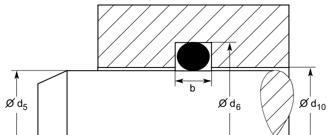
Fig. 3.10 Rod seal – radial compression
