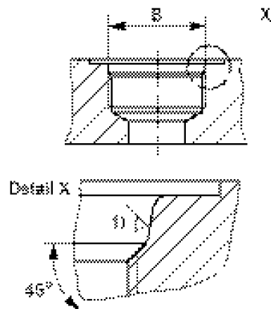
Fig. 4.1 Threaded connector with conical counterbore
