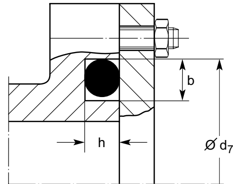
Fig. 3.3 Flange seal – axial compression
