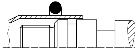
Fig. 2.29 Use of a fitting aid
