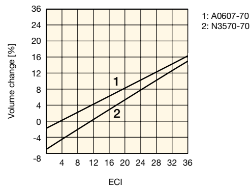
Fig. 8.7 Swelling characteristics of Parker compounds
