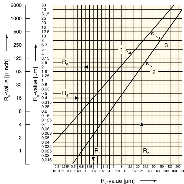
Fig. 8.16 Relationship between R_a and R_z
