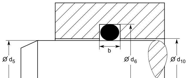
Fig. 3.14 Rod seal – radial compression
