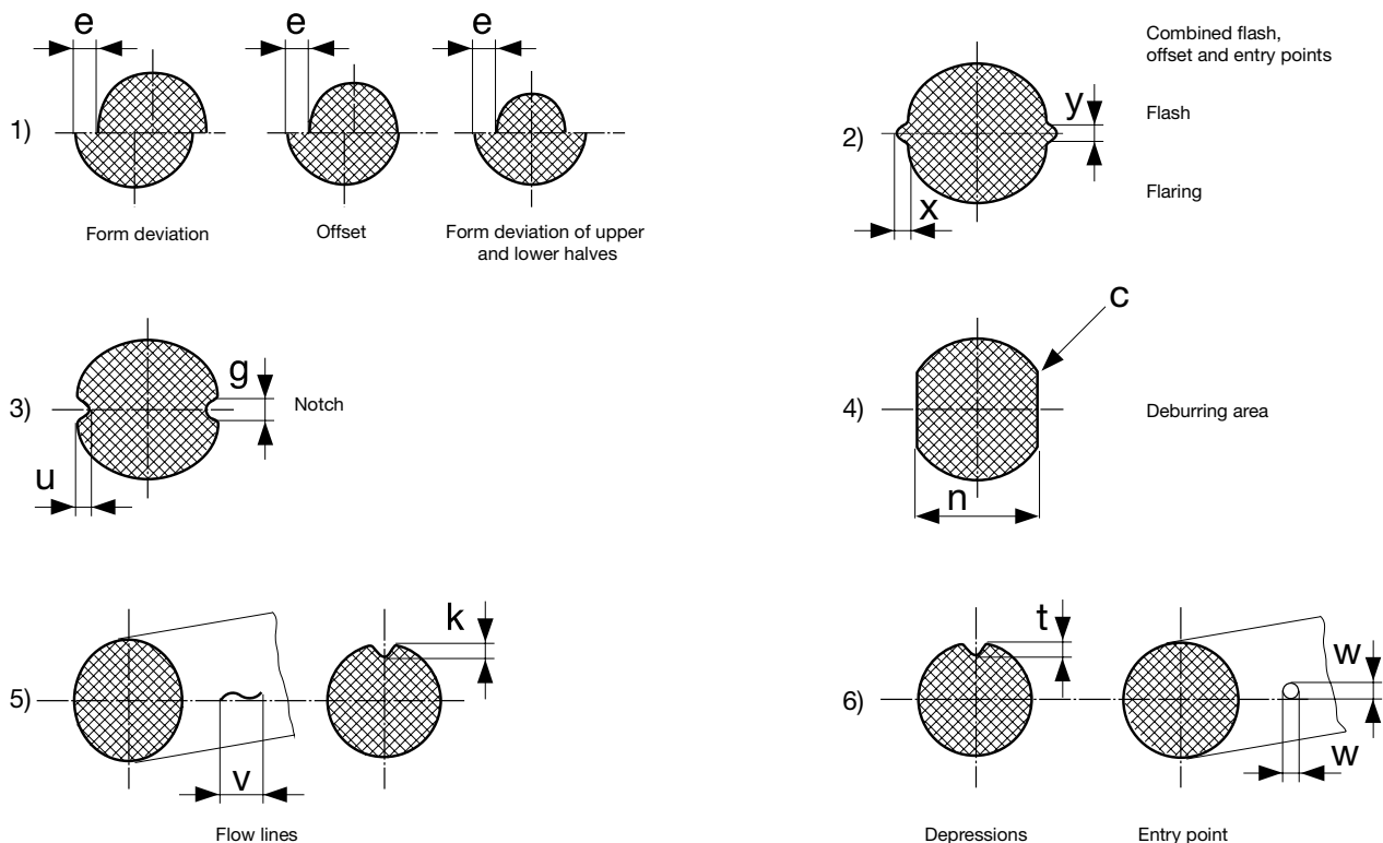
Fig. 9.1 Form and surface finish defects
