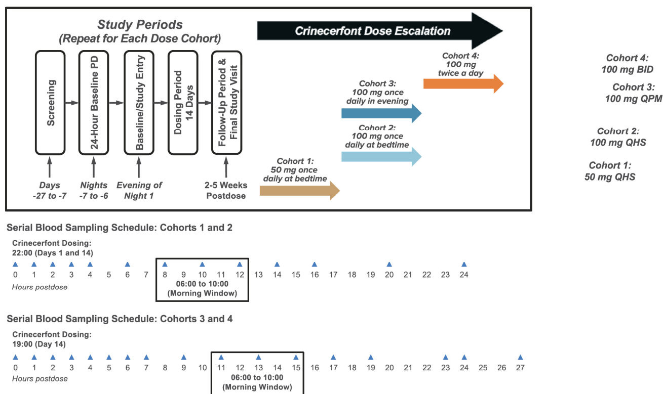
Figure 1. Study design. Blue triangles denote sample collection. In all cohorts, sampling for the 24-hour baseline period (day -7 to -6) matched the sampling schedule during crinecerfont treatment. For the baseline and day 1 visits, participants received their prescribed glucocorticoid dose after sample collection at 10:00 (end of the morning window); for the day 14 visit, glucocorticoid was administered after sample collection at 14:00. GC, glucocorticoid.
