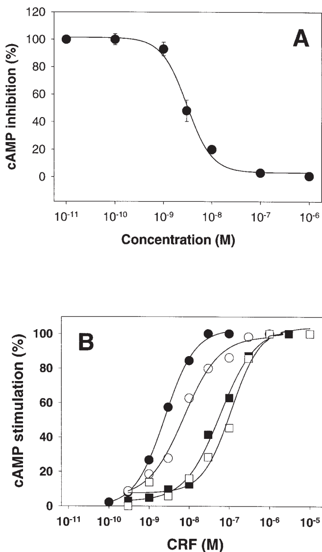
Fig. 2. Antagonism by SSR125543A of CRF-induced cAMP synthesis in Y 79 cells. A, concentration effect of SSR125543A for the inhibition of cAMP synthesis stimulated by 10 nM rat/human CRF. Results are expressed as the percentage of inhibition of the maximal increase induced by CRF. B, concentration-response curves for CRF-stimulated cAMP synthesis in Y 79 cells in the absence (●) or presence of SSR125543A at 3 nM (○), 30 nM (■), and 100 nM (□). Results are expressed as percentage of increase induced by CRF in the presence or absence of competitor. For both experiments, the data are the means of three independent experiments ( \pm S.E.M., Fig. 3A).
