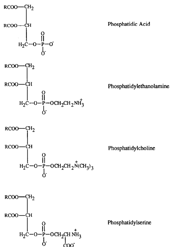
Fig. 2. Phospholipid structures; R is an alkyl chain from 8–24 units long.
