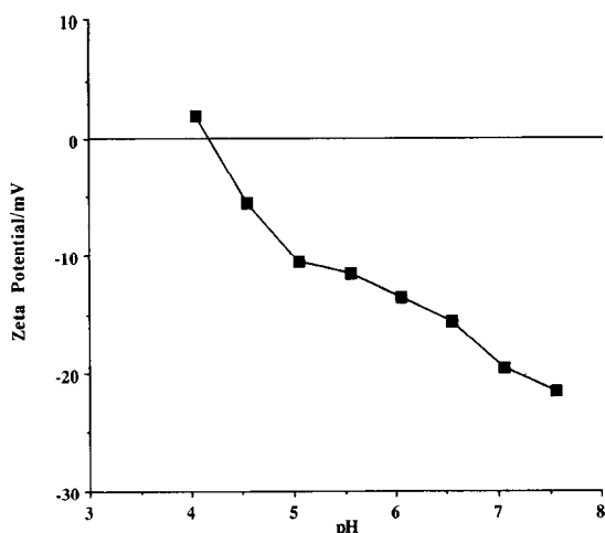
Fig. 10. Zeta potential of an Ovothin 200 stabilized triglyceride emulsion as a function of pH.
