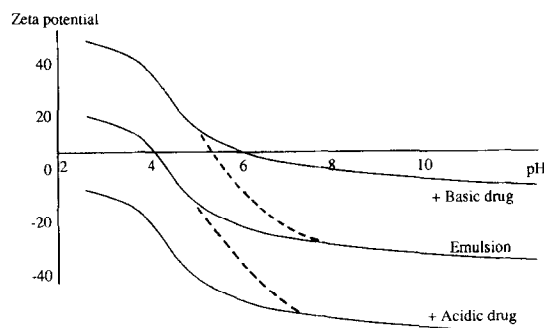
Fig. 9. Hypothetical zeta potential vs. pH for emulsions containing acidic or basic drugs. The dashed lines indicate the transition between ionized and neutral forms of a drug with pK 6.0.
