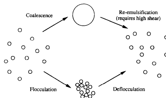
Fig. 1. Flocculation and coalescence in colloidal dispersions.
