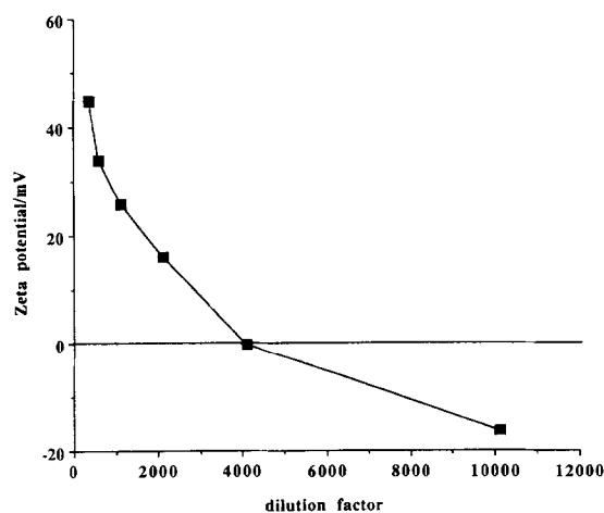
Fig. 15. Measured zeta potential of 2% emopamil in 20% soya oil/Ovothin 200 emulsion as a function of sample dilution (pH 5).
