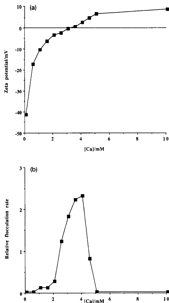
Fig. 7. (a) Zeta potential and (b) relative flocculation rate of Intralipid in calcium chloride solutions.
