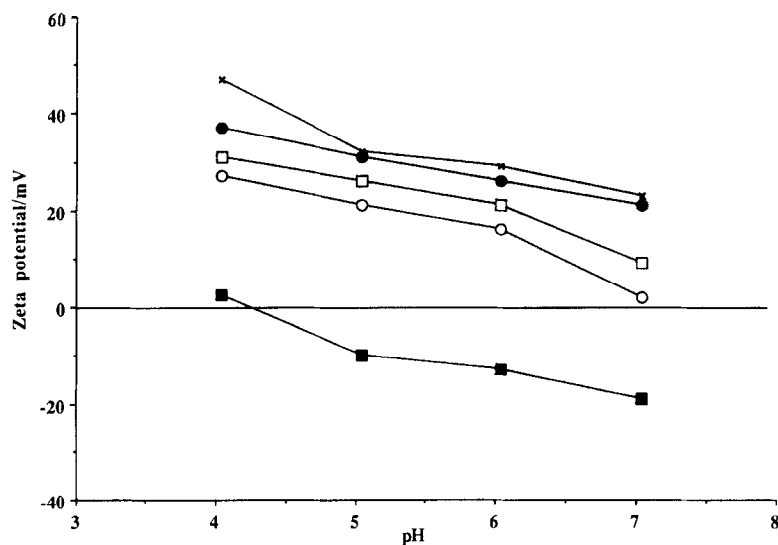
Fig. 13. Zeta potential/pH curves for Emopamil-containing emulsions stabilized by Ovothin 200. ■, 0% Emopamil; ○, 0.2%; □, 0.5%; ●, 1%; ×, 2%.
