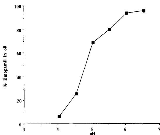
Fig. 14. Distribution of emopamil in emulsion as a function of pH.
