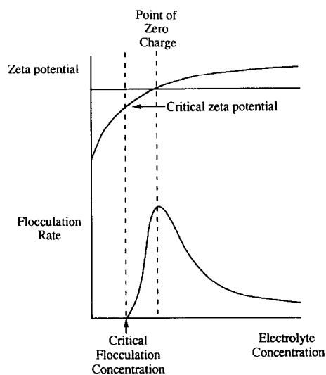
Fig. 6. Zeta potential and flocculation (specific adsorption).
