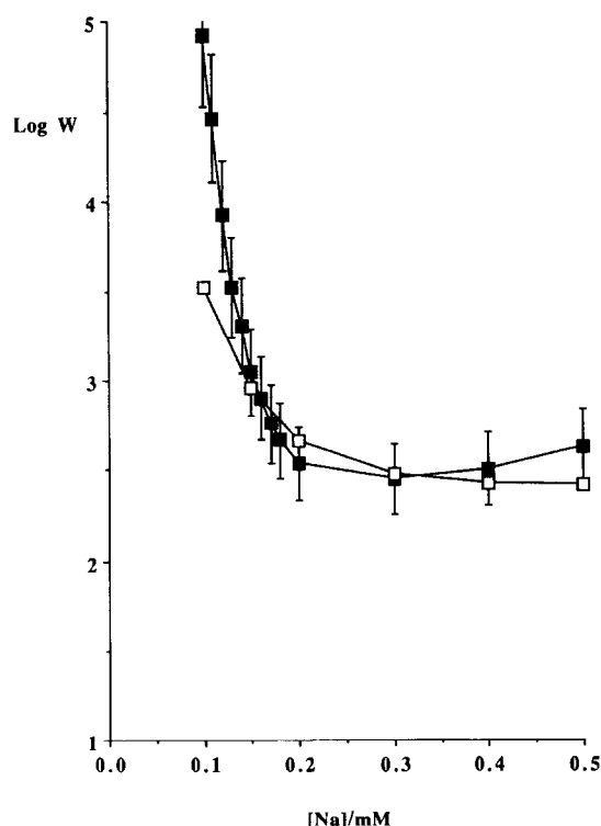
Fig. 5. Measured ■ and calculated □ stability ratios for a triglyceride emulsion in sodium chloride solutions.
