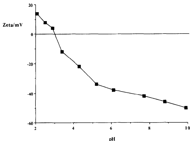
Fig. 8. Zeta potential of Intralipid as a function of pH.
