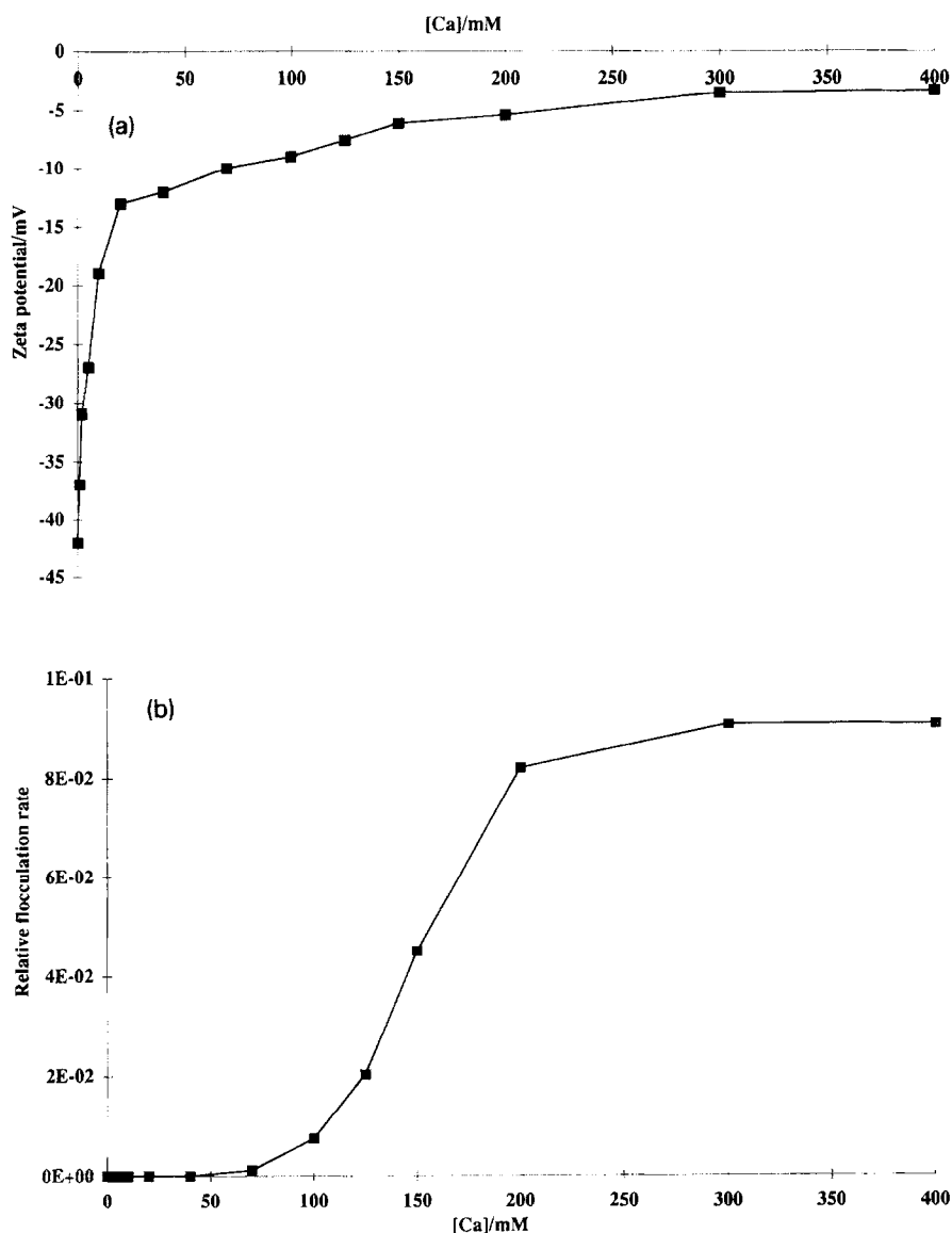
Fig. 4. (a) Zeta potential and (b) relative flocculation rate of Intralipid in sodium chloride solutions.
