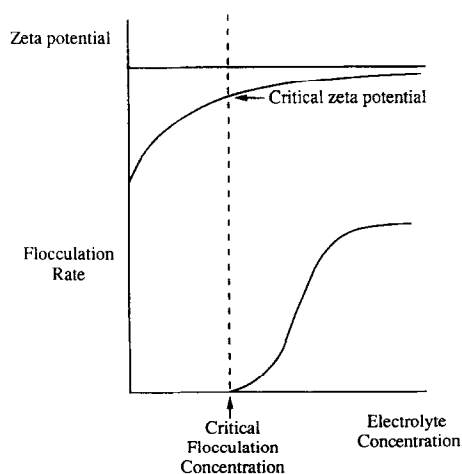
Fig. 3. Zeta potential and flocculation (nonspecific adsorption).
