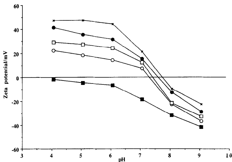
Fig. 12. Zeta potential/pH curves for Emopamil-containing emulsions stabilized by Ovothin 180. ■, 0% Emopamil; ○, 0.2%; □, 0.5%; ●, 1%; ×, 2%.
