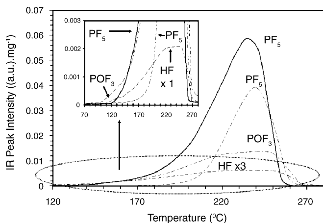
Fig. 3. Evolution of gaseous products as a function of temperature during thermal decomposition of \text{LiPF}_6 at a heating rate of 10^\circ\text{C min}^{-1} in argon (flow rate: 220\text{ ml min}^{-1} ) containing less than 10 ppm water (solid line) and with 300 ppm water vapor (dashed line).
