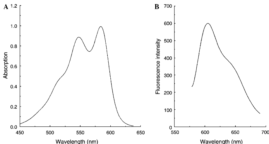
Fig. 3. Absorption and fluorescence spectra of the Morgan–Elson colored product. (A) Absorption spectrum obtained for GlcNAc (final concentration of 12 \mu\text{g}/\text{ml} of 0.1 M formate buffer containing 0.1 M NaCl, pH 3.9). (B) Fluorescence spectrum obtained for GlcNAc (final concentration of 0.98 \mu\text{g}/\text{ml} of 0.1 M formate buffer containing 0.1 M NaCl, pH 3.9). Excitation wavelength was 545 nm.
