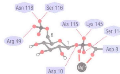
Figure 2-41 The phosphoenzyme–substrate intermediate in the active site of beta-phosphoglucmutase from Lactococcus lactis . In the active site of beta-phosphoglucmutase, phosphoryl-group transfer occurs via aspartic acid 8, which can be phosphorylated to form a stable phosphoaspartyl-enzyme. In the reaction glucose 6-phosphate (G6P) to glucose 1-phosphate (G1P), for example, the unphosphorylated C1 OH of the substrate is positioned such that it can become linked to the phosphoaspartyl group as shown. In this intermediate, the phosphate being transferred is pentavalent and is still associated with both aspartic acid 8 (in a mixed anhydride linkage) while becoming covalently linked to the G6P substrate to form the intermediate 1,6-bisphosphoglucose–enzyme complex. Subsequent reaction of the phosphoryl group at the 6 position of the sugar with the aspartic acid 8 is thought to complete the transfer to C1, forming G1P and regenerating the phosphoaspartyl-enzyme.
