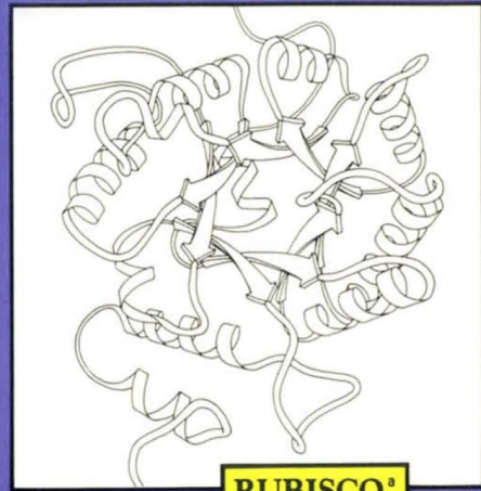
RUBISCO a
