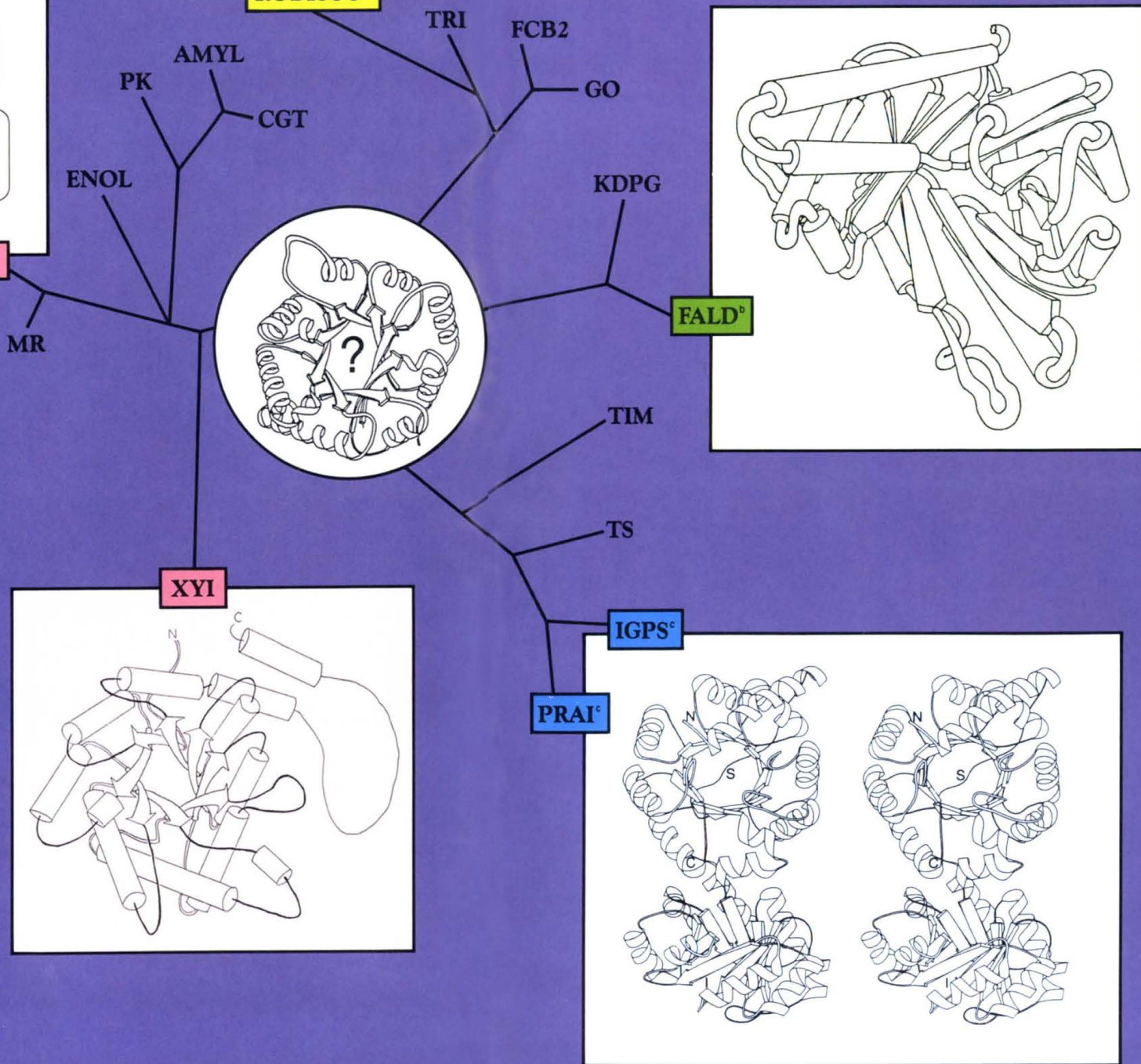
RUBISCO a
