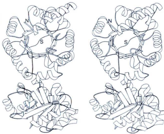
PRAI c
