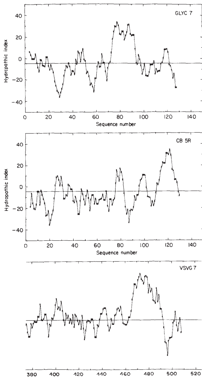
FIG. 5. SOAP profiles for 3 different proteins that have membrane affiliation. In the upper panel, the plot is that of erythrocyte glyophorin (GLYC), which has an easily recognized membrane-spanning segment in the region of residues 75 to 94. In the middle panel, rabbit cytochrome b_5 (CB5R) is depicted. In this case there is a membrane-anchoring unit involving the 20-residue carboxy-terminal segment. In the lower panel, the carboxy-terminal region of vesicular stomatitis virus glycoprotein (VSVG) is shown; a membrane-spanning segment is clearly evident from residues 470 to 490. All profiles are at span settings of 7.
