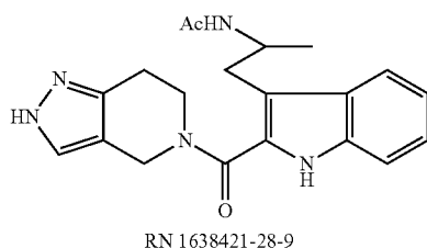
[Chemical Formula 1]
