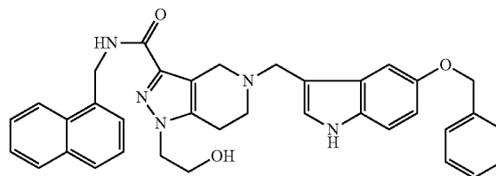
[Chemical Formula 2]
