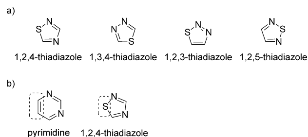
Figure 1. a) Core structures of thiadiazoles discussed in this Minireview. b) A side by side comparison of the basic structures of the pyrimidine and 1,2,4-thiadiazole scaffold.
