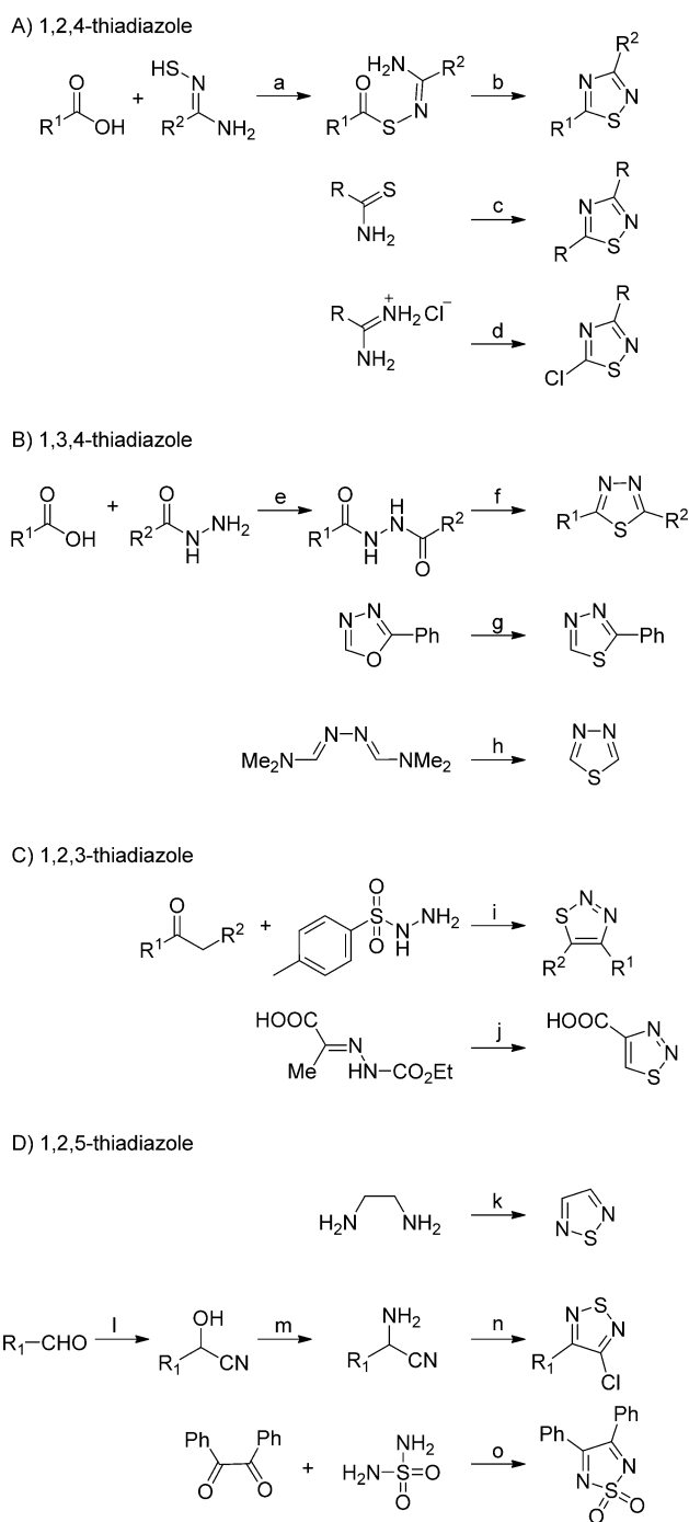
Scheme 2. Synthesis of A) 1,2,4-thiadiazole: a) Carbonyldiimidazole (CDI), DMF; b) CDI, DMF, Δ; c) I 2 , EtOH; d) CCl 3 SCl, NaOH, CH 2 Cl 2 , 8 °C; B) 1,3,4-thiadiazole: e) 1-Ethyl-3-(3-dimethylaminopropyl)carbodiimide (EDCI), hydroxybenzotriazole (HOBt), THF, RT; f) Lawesson's reagent, THF, reflux; g) P 4 S 10 , xylene, Δ; h) H 2 S, MeOH, RT; C) 1,2,3-thiadiazole: i) 1. EtOH, reflux, 3 h; 2 SOCl 2 , CHCl 3 , 0–5 °C, 4 h; j) SOCl 2 , 60 °C; D) 1,2,5-thiadiazole: k) S 2 Cl 2 , DMF, 80 °C; l) KCN/H 2 O/HOAc; m) NH 4 Cl/NH 3 (aq); n) S 2 Cl 2 /DMF; o) HCl, EtOH, RT.
