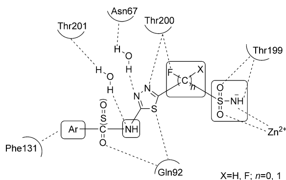
Figure 3. A function model of CA inhibitors. [15]
