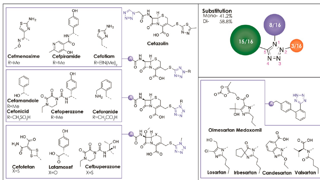
Figure 11. Pharmaceuticals containing tetrazoles.
