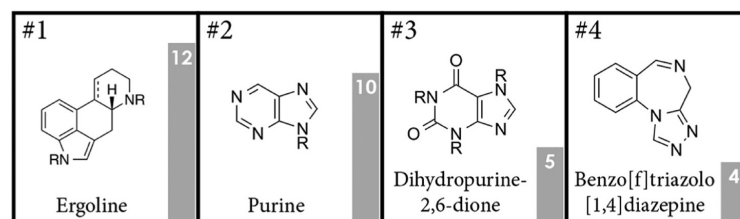
Figure 24. Top four most common fused nitrogen heterocycles.
