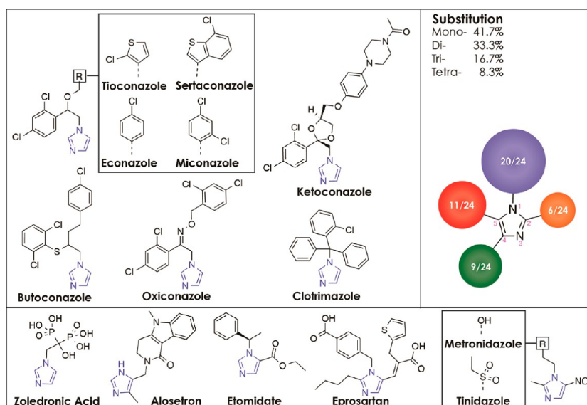
Figure 9. Pharmaceuticals containing imidazoles.
