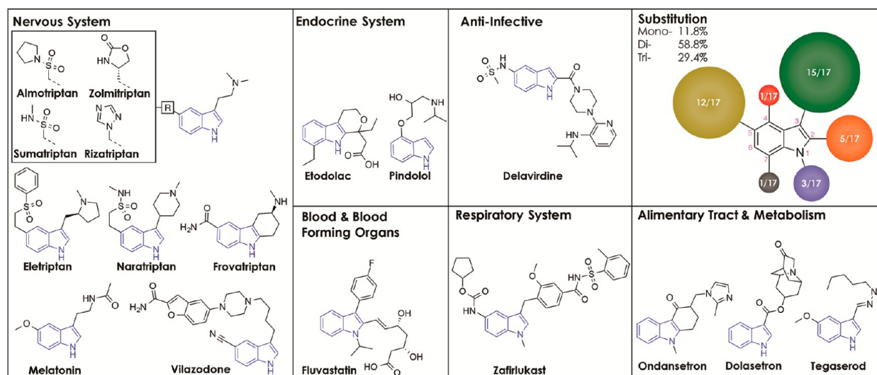
Figure 10. Pharmaceuticals containing indoles.
