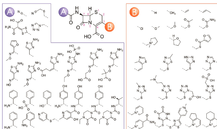
Figure 5. Structural variations of approved cephem pharmaceuticals.
