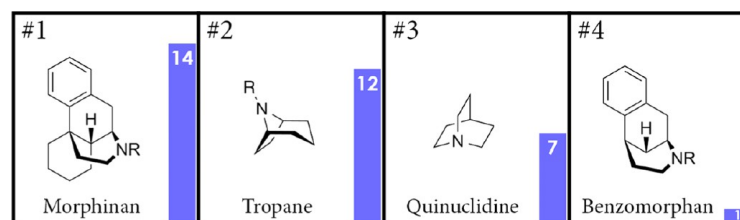
Figure 27. Top four most common bridged bicyclic nitrogen heterocycles.
