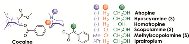
Figure 29. Pharmaceuticals containing tropanes.
