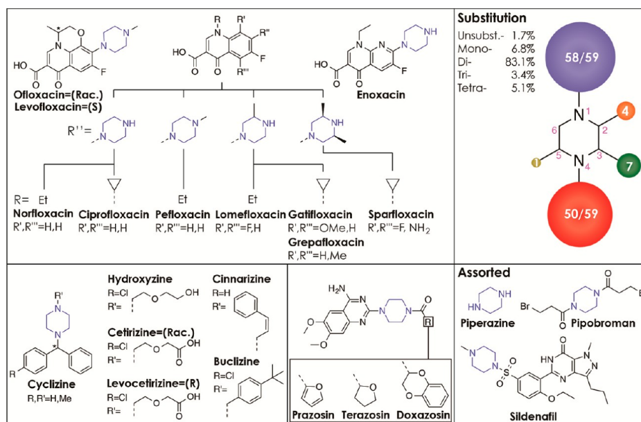
Figure 20. Pharmaceuticals containing piperazines.
