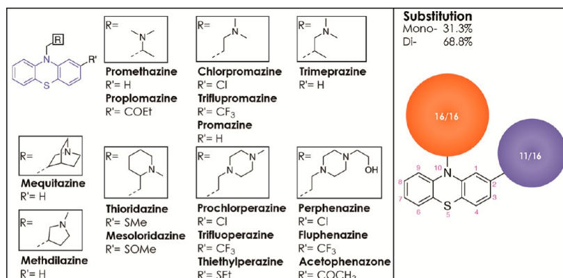
Figure 21. Pharmaceuticals containing phenothiazines.
