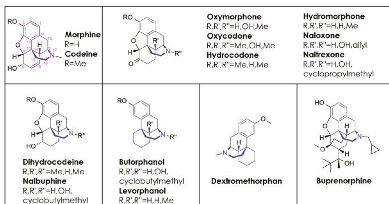
Figure 28. Pharmaceuticals containing morphinans.
