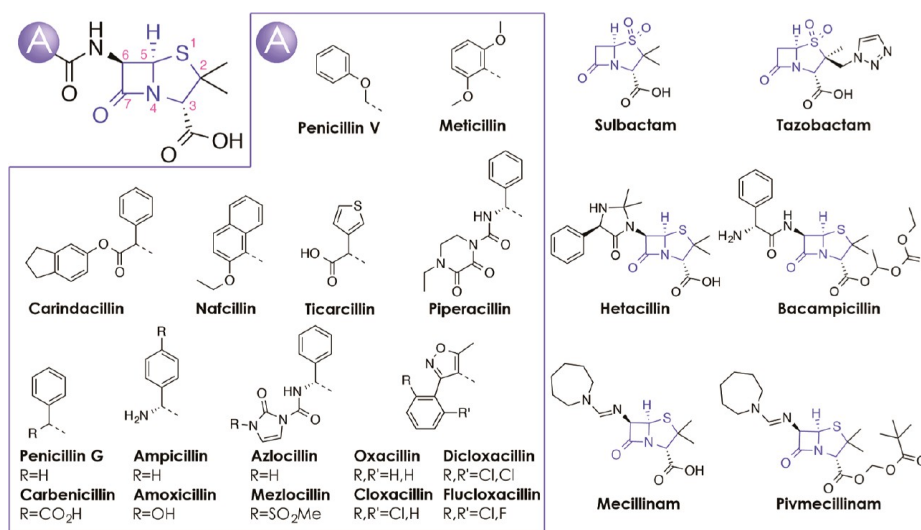
Figure 6. Structural variations of approved penam pharmaceuticals.
