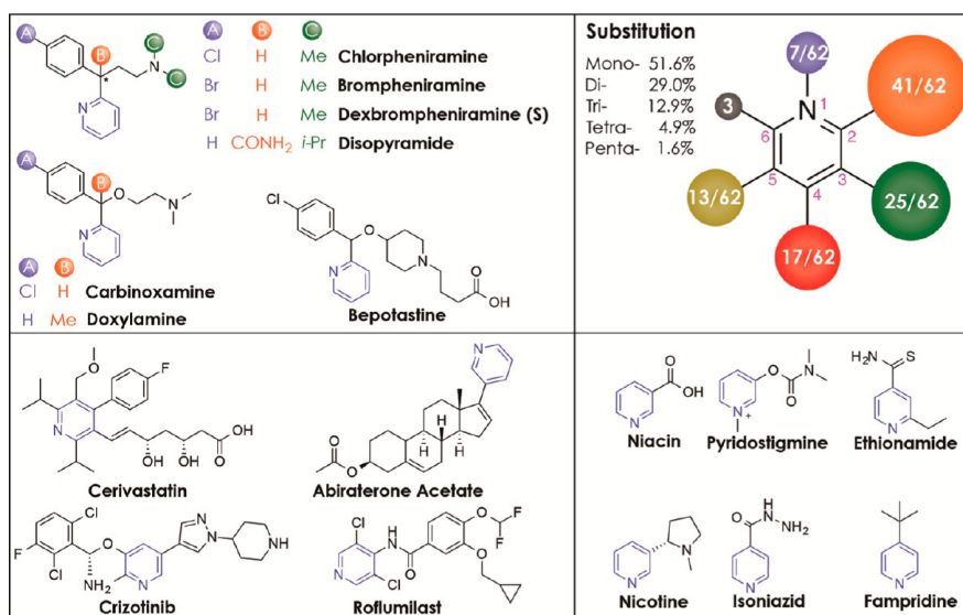
Figure 16. Pharmaceuticals containing pyridines.
