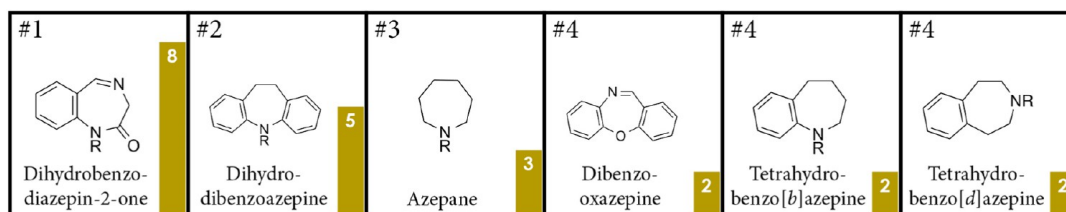
Figure 22. Top five most common seven-membered nitrogen heterocycles.
