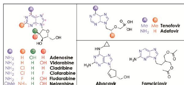
Figure 26. Pharmaceuticals containing purines.
