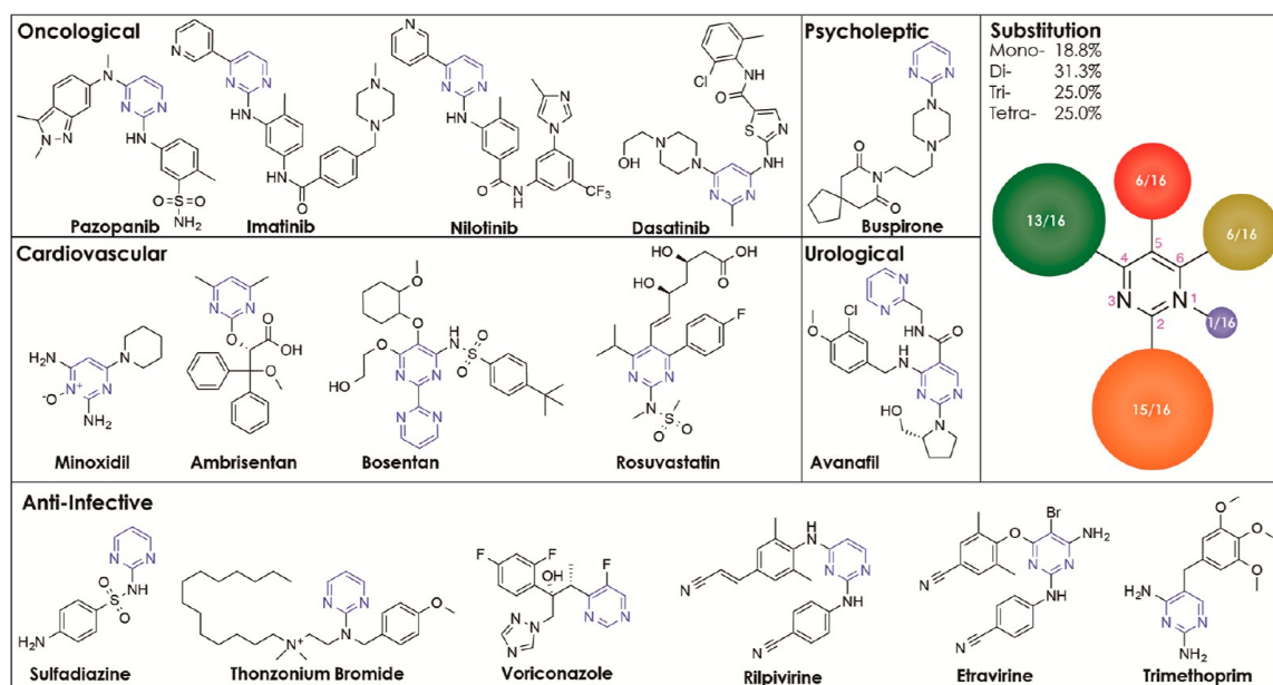
Figure 17. Pharmaceuticals containing pyrimidines.
