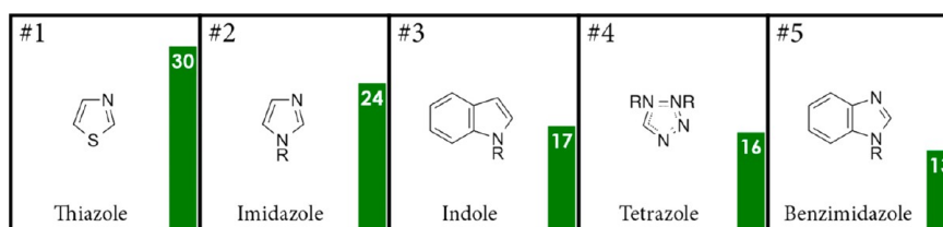
Figure 7. Top five most common five-membered aromatic nitrogen heterocycles.
