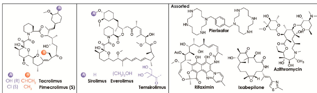
Figure 31. Examples of U.S. FDA approved nitrogen macrocycles.
