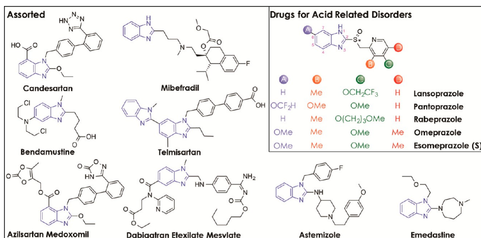
Figure 12. Pharmaceuticals containing benzimidazoles.
