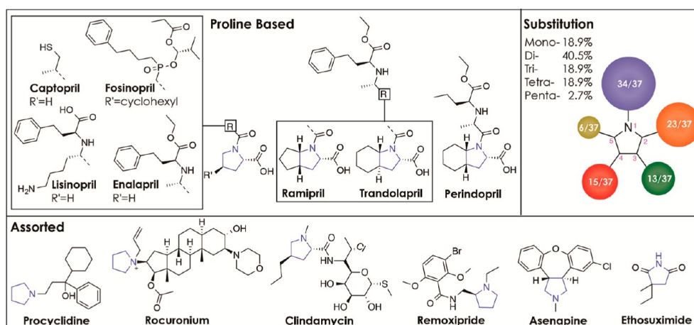
Figure 14. Pharmaceuticals containing pyrrolidines.
