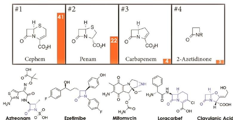
Figure 4. Top four most common four-membered nitrogen heterocycles.
