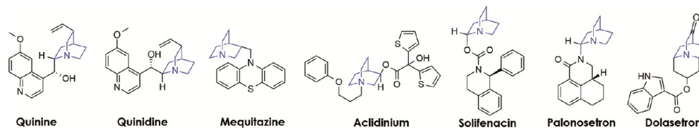
Figure 30. Pharmaceuticals containing quinuclidines.
