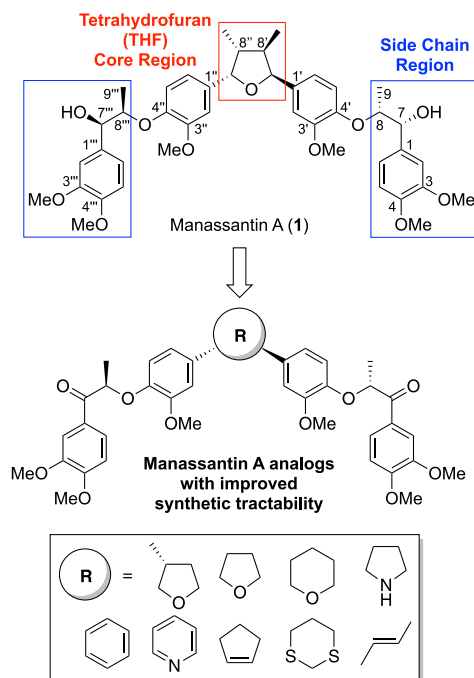
Figure 1. Structure and SAR plan of manassantin A.
