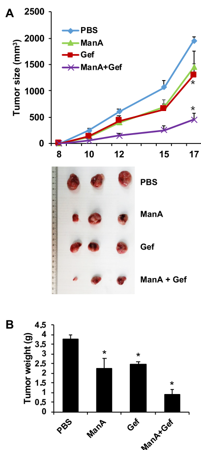
Figure 4. Manassantin A (ManA) cooperatively inhibits tumor growth in combination with an EGFR inhibitor, gefitinib (Gef). Lewis lung carcinoma cells ( 2 \times 10^5 ) were inoculated into both flanks of C57Bl/6 mice (Day 0). From two days after inoculation, mice ( n = 5 per group) were treated intraperitoneally with manassantin A (5 mg/kg body weight) and/or gefitinib (5 mg/kg body weight) three times a week for 17 days and then sacrificed. Tumor size (A) and tumor weight (B) were measured three times a week and on the final day, respectively. Tumor masses were photographed and shown in a box right the graph. * P < 0.05 versus vehicle control group.
