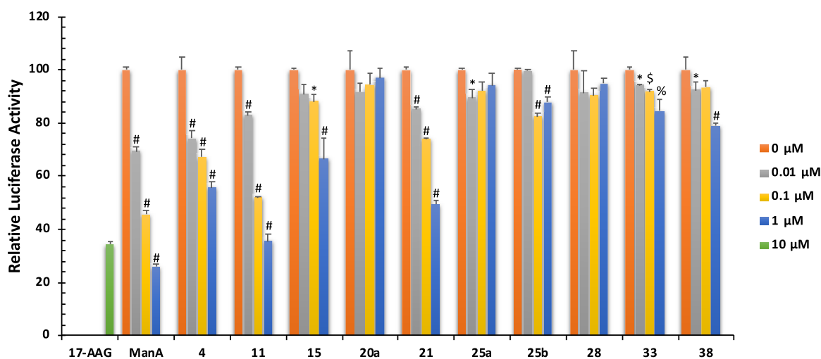
Figure 2. Activity of manassantin A (ManA) and analogues for HIF-1 inhibition. HEK-293T cells were transfected with pGL3-SHRE-VEGF-luciferase and pRL-SV40 plasmids, and treated with 0, 0.01, 0.1, and 1 \mu M of ManA (manassantin A) and analogues or 10 \mu M of 17-AAG (17-(allylamino)-17-demethoxygeldanamycin), as a positive control under hypoxia for 24 h. Relative luciferase activity was determined after normalized to the Renilla luciferase activity. Three independent experiments were performed. # P < 0.0001 versus vehicle control group, % P < 0.001 versus vehicle control group, $ P < 0.01 versus vehicle control group, and * P < 0.1 versus vehicle control group.
