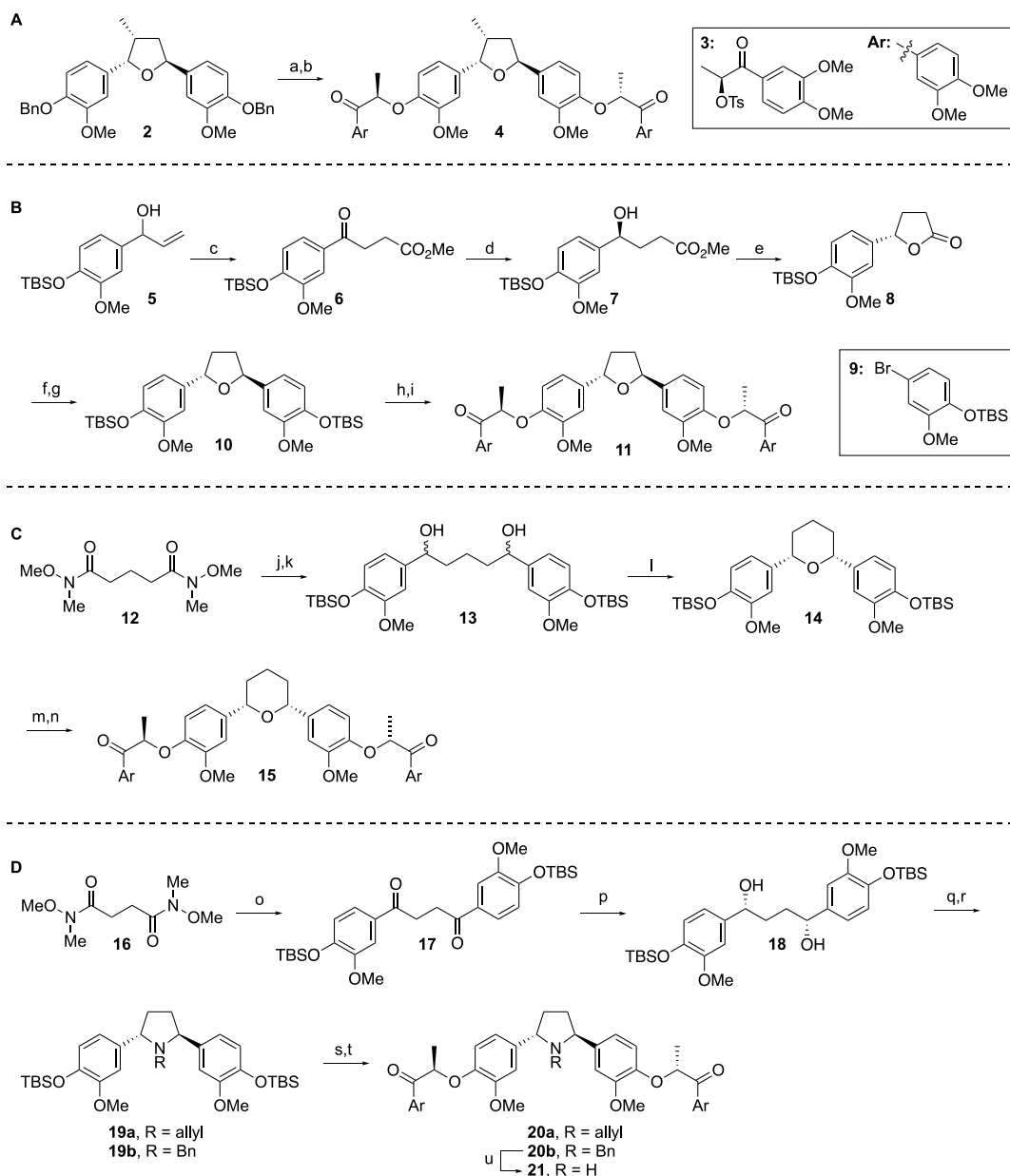
Scheme 1. Synthesis of the Analogues 4, 11, 15, 20a, and 21 a
