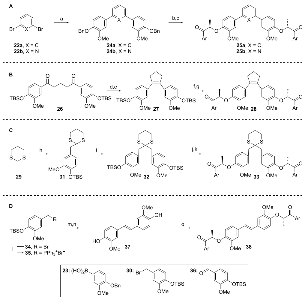
Scheme 2. Synthesis of the Analogues 25a, 25b, 28, 33, and 38 a
