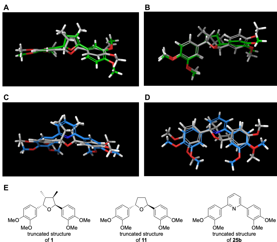
Figure 3. Overlays of optimized conformations of manassantin A (1) and analogues (11 and 25b). To avoid any unnecessary complications and/or exaggeration by the flexible side chains, truncated structures of 1, 11, and 25b were used instead of the full structures. Initial geometries were determined by conformational search based on MMFF and OPLS3. (A and B) Superimposition of an active manassantin A analog (gray: 1; green: 11). (C and D) Superimposition of an inactive manassantin A analog (gray: 1; sky blue: 25b). (E) Truncated structures 1, 11, and 25b.
