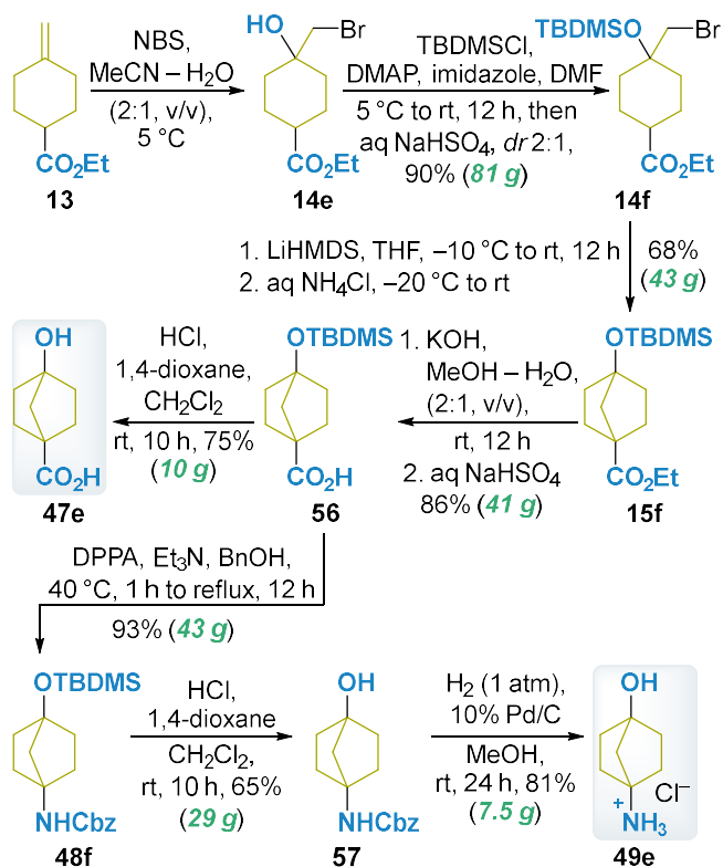
Scheme 8. Synthesis of building blocks 47e and 49e.
