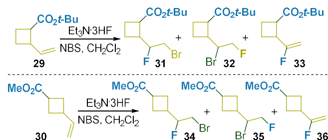
Scheme 3. Unsuccessful attempts on the fluorobromination of unsaturated esters 29 and 30 (the structures of the plausible products are proposed according to LC-MS and 1 H NMR spectra).
