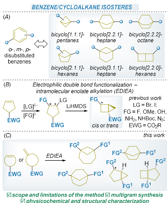
Scheme 1. (A) Some remarkable examples of the known bicyclic benzene/cycloalkane isosteres. (B) Electrophilic double bond desymmetrization – intramolecular enolate alkylation sequence for the synthesis of 1,3-disubstituted bicyclo[2.1.0]pentanes (housanes). (C) The main targets of this work.
