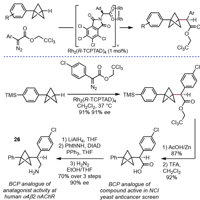
Scheme 19. Rhodium-Catalyzed Bridgehead C–H Diazocarbonyl Insertion (Davies et al. 43 )
