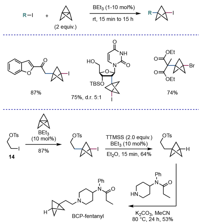
Scheme 7. Atom Transfer Radical Addition (ATRA) of Alkyl Halides Using Triethylborane as Initiator (Anderson et al. 25 )
