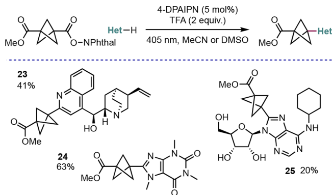
Scheme 18. Decarboxylative Minisci Coupling of Redox-Active BCP Esters (Mousseau et al. 42 )
