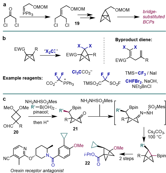
Scheme 15. Synthesis of Bridge-Substituted BCPs, including (a) a Classical Route to Bridge-Substituted [1.1.1]Propellanes, (b) Dihalocarbene Insertion in Bicyclo[1.1.0]butanes, and (c) a Barluenga-Type 1,2-Metallation Approach to Bridge-Substituted BCPs (Qin et al. 40 )
