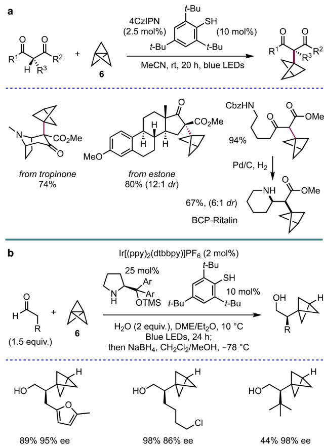
Scheme 9. (a) \alpha -Quaternary BCPs Synthesis via Addition of Electron-Deficient Radicals to 2 and (b) \alpha -Chiral BCPs Synthesis via Dual Organo/Photoredox Catalysis (Anderson et al. 27,28 )
