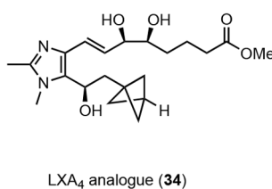
Figure 2. Examples of BCP substitution in bioactive molecules.
