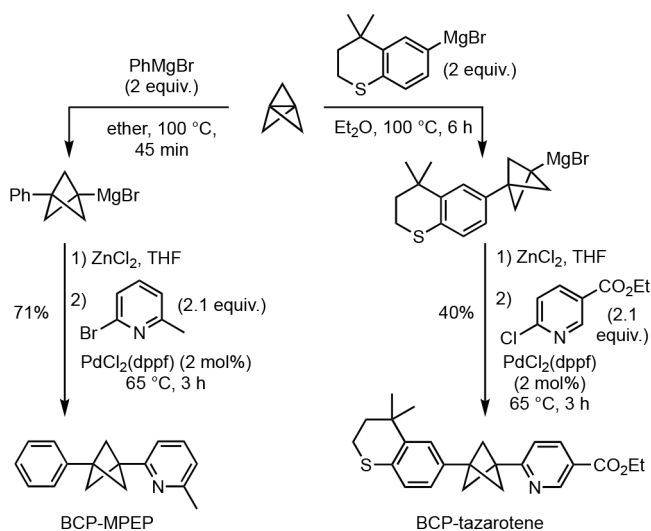
Scheme 16. Negishi Cross-Coupling of Bridgehead BCP Organozincs (Knochel et al. 16b )
