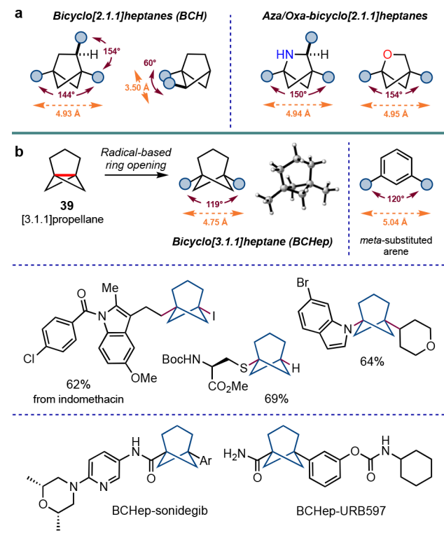
Scheme 23. (a) Related Bicyclic Scaffolds of Interest in Medicinal Chemistry Research and (b) Radical-Based Synthesis of Bicyclo[3.1.1]heptanes (BCHepts) (Anderson et al. 55 )
