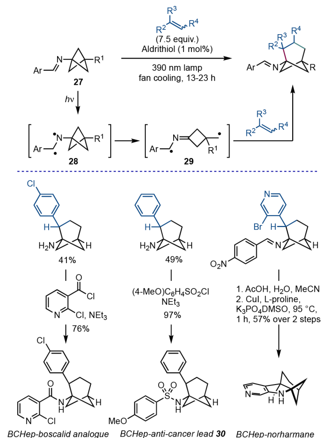
Scheme 20. Photochemical Alkene Insertion into BCP Imines (Stephenson et al. 44 )
