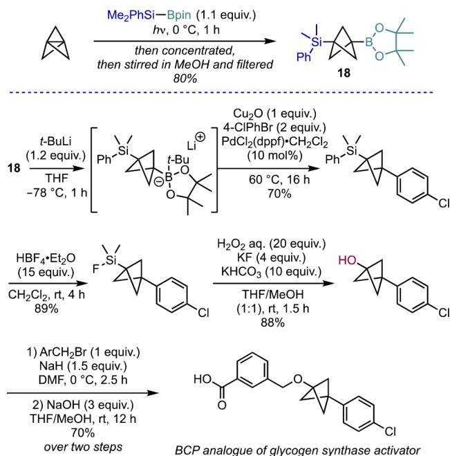
Scheme 14. Silylboration of [1.1.1]Propellane and Subsequent Functionalization (Uchiyama et al. 37 )
