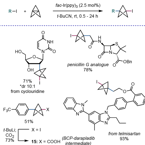
Scheme 8. ATRA Addition of Alkyl and (Hetero)aryl Halides under Photoredox Catalysis (Anderson et al. 26 )
