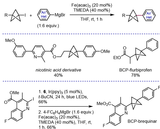
Scheme 17. Kumada Cross-Coupling of Bridgehead BCP Iodides (Anderson et al. 41 )
