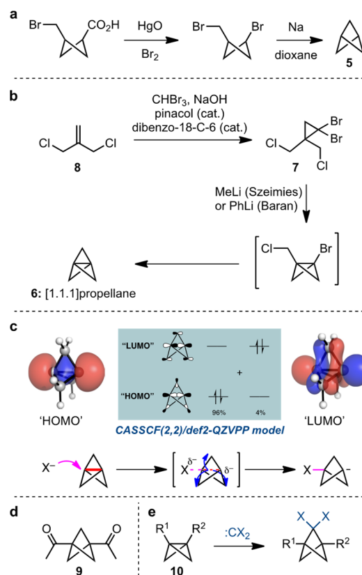
Scheme 1. Wiberg Synthesis of Bicyclo[1.1.1]pentane, 9 (b) the Optimal Synthesis of [1.1.1]Propellane, 11,13 (c) a Delocalized Ground-State Description of [1.1.1]Propellane Connects to Its Reactivity with Anions and Radicals, (d) Biacetyl BCP, and (e) Carbene Addition to Bicyclo[1.1.0]butanes
