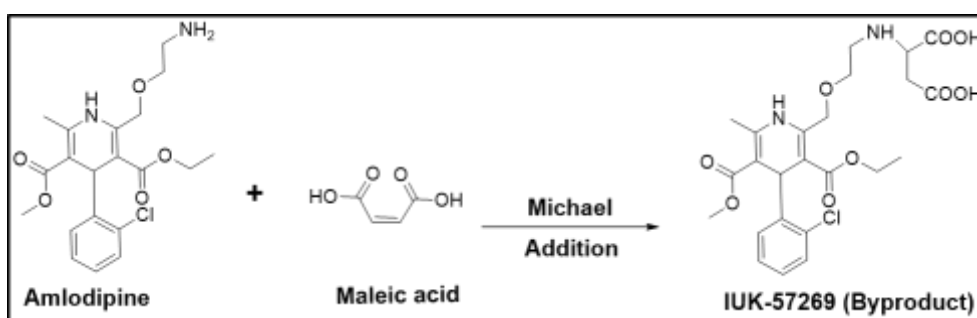
Figure 1. Degradation reaction of amlodipine in the presence of maleic acid.
