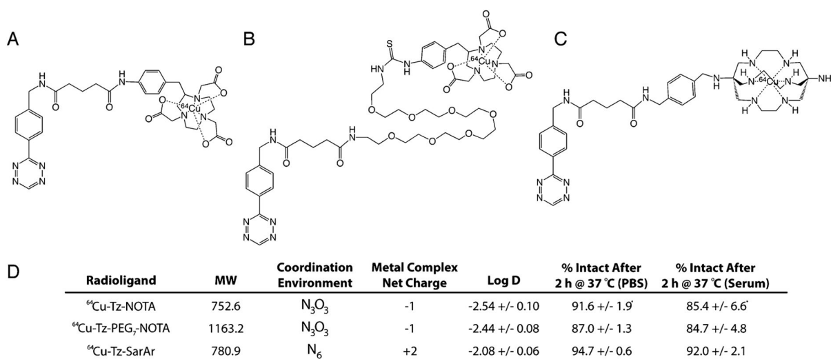
Figure 3. Structures of (A) ^{64}\text{Cu} -Tz-NOTA, (B) ^{64}\text{Cu} -Tz-PEG 7 -NOTA, (C) ^{64}\text{Cu} -Tz-SarAr, along with (D) some selected properties of the three tetrazine radioligands. Data originally reported in Zeglis, B. M. et al. Journal of Nuclear Medicine . 54 , 1389–1396 (2013). © 2013 by the Society of Nuclear Medicine and Molecular Imaging, Inc. 44
