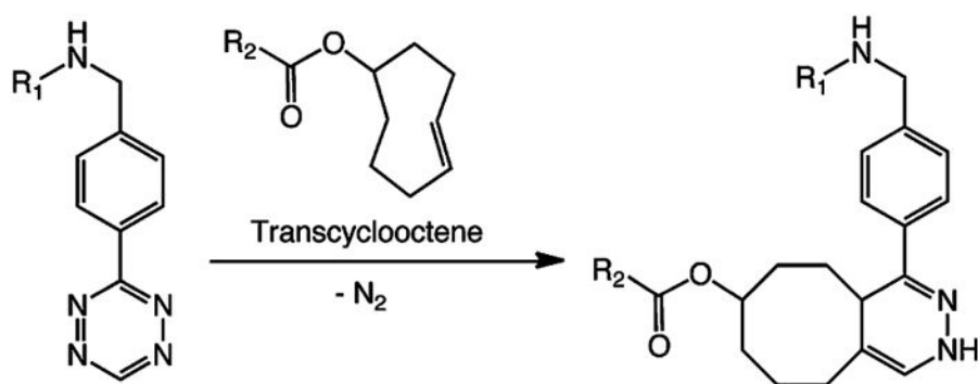
Figure 1. Inverse electron demand Diels–Alder cycloaddition.
