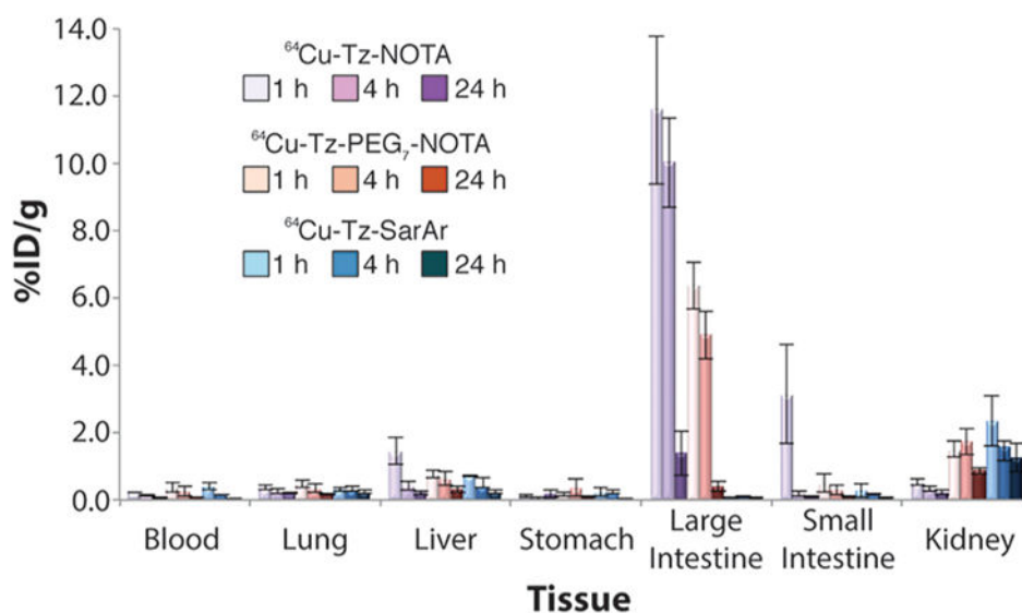
Figure 4. Biodistribution data (%ID/g \pm SD) of ^{64}\text{Cu} -Tz-NOTA, ^{64}\text{Cu} -Tz-PEG 7 -NOTA, and ^{64}\text{Cu} -Tz-SarAr in healthy athymic nude mice ( n = 4 for each time point). Mice were administered the radioligands (25–30 \mu\text{Ci} in 200 \mu\text{L} of 0.9% sterile saline) via intravenous tail vein injection and euthanized by \text{CO}_2(\text{g}) asphyxiation at 1, 4, and 24 h after injection.
