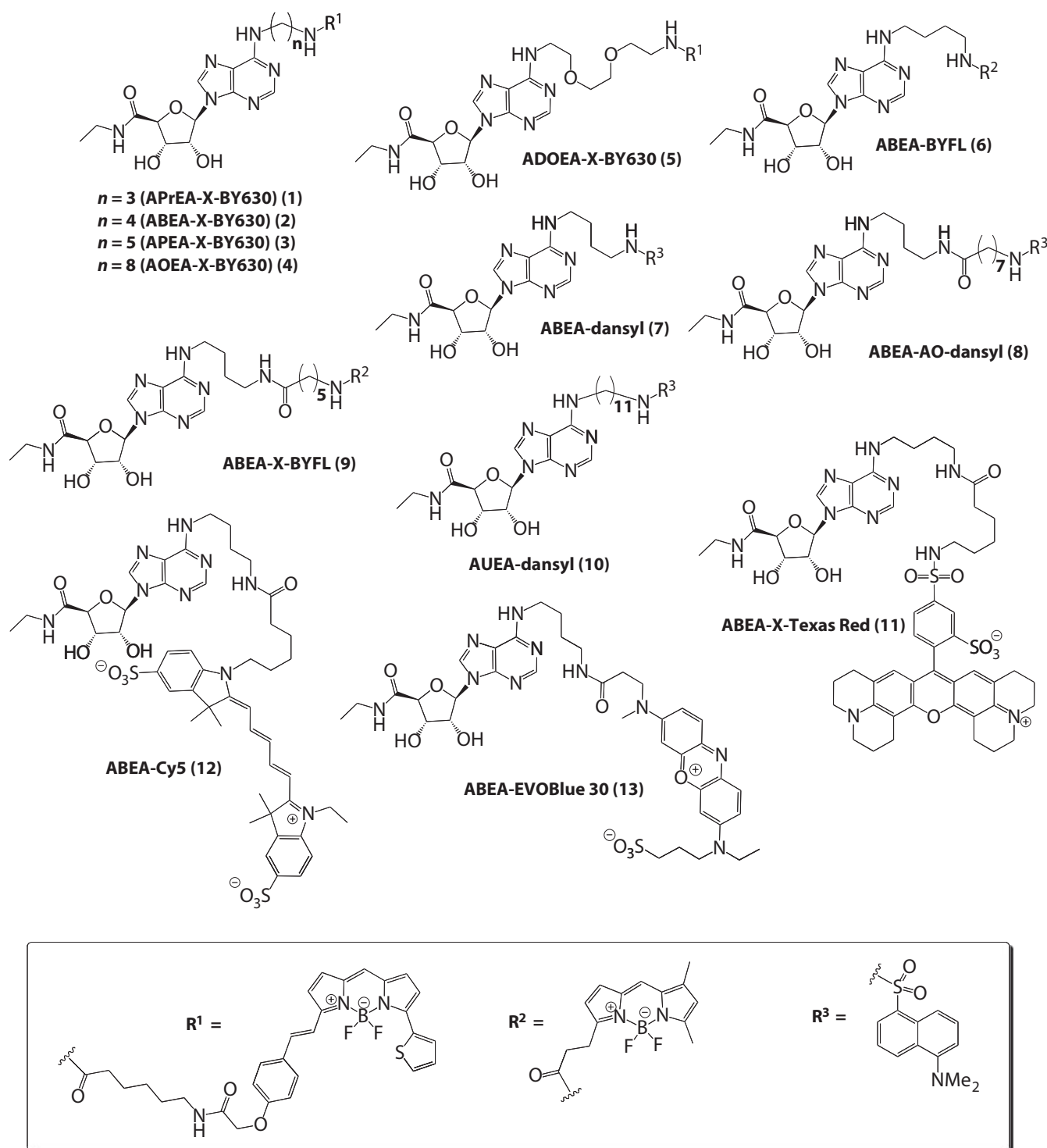
Figure 1 Chemical structures of fluorescent NECA derivatives. ABEA, N 6 -(4-aminobutyl)-5'-ethylamino-5'-oxo-5'-deoxyadenosine; ADOEA, N 6 -(8-amino-3,6-dioxaoctyl)-5'-ethylamino-5'-oxo-5'-deoxyadenosine; AO, 8-aminooctanoyl; AOEa, N 6 -(8-aminooctyl)-5'-ethylamino-5'-oxo-5'-deoxyadenosine; APEA, N 6 -(5-aminopentyl)-5'-ethylamino-5'-oxo-5'-deoxyadenosine; APrEA, N 6 -(3-aminopropyl)-5'-ethylamino-5'-oxo-5'-deoxyadenosine; AUEA, N 6 -(11-aminoundecyl)-5'-ethylamino-5'-oxo-5'-deoxyadenosine; X, 6-aminohexanoyl.
