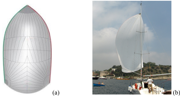
Fig. 5. (a) Spinnaker designed shape and its arrangement of panels; (b) flying shapes.
