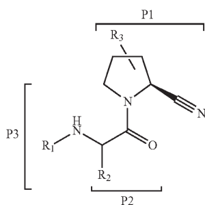
Generic structure of N-acyl-glycyl(2-cyano)pyrrolidines
