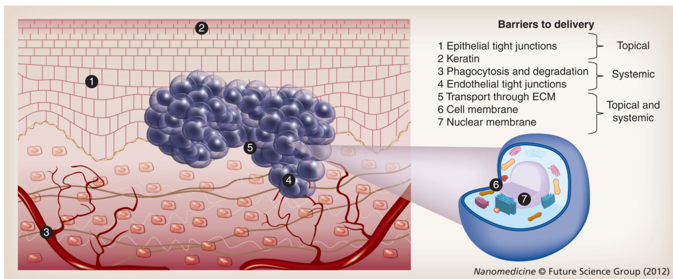
Figure 5. Barriers to contrast agent delivery
