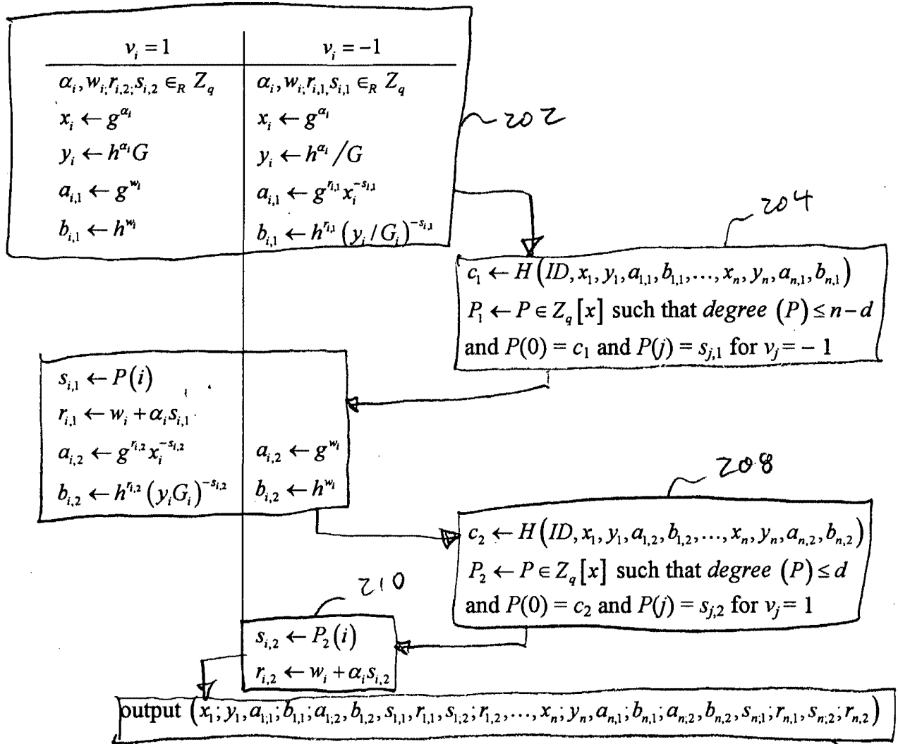
Figure 2: Ballot Encryption and Proof of Ballot Validity
