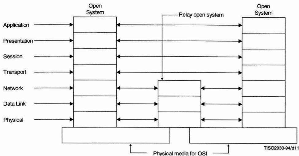
Figure 12 – Communication involving relay open systems
