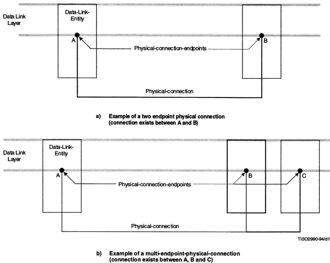
Figure 18 – Examples of physical connections
