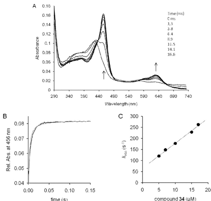
Figure 5. Reaction of MPO Compound I with compound 34 (pH 7.4 and 25 °C). (A) Spectral changes upon reaction of 2 \mu M MPO Compound I with 10 \mu M compound 34. First spectrum after mixing corresponds to Compound I subsequent spectra were recorded after 1.3, 3.8, 6.4, 8.9, 11.5, 14.1, and 16.6 ms. Arrows indicate spectral changes. (B) Typical time trace and fit of MPO Compound II formation followed at 456 nm. (C) Pseudo-first-order rate constants for MPO Compound I reduction plotted against compound 34 concentration.
