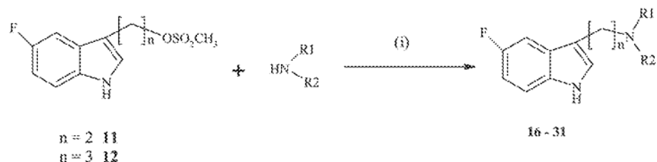
Scheme 4. Synthesis of Compounds 16–31 a
