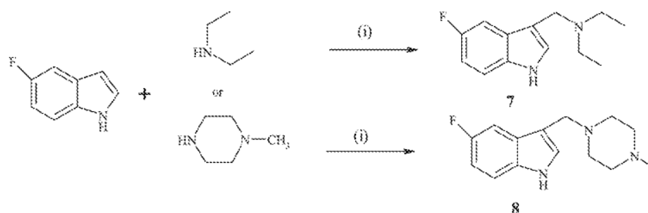
Scheme 2. Synthesis of Substituted 3-(Aminomethyl)indoles a
