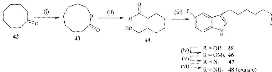
Scheme 7. Synthesis of Compound 48 a
