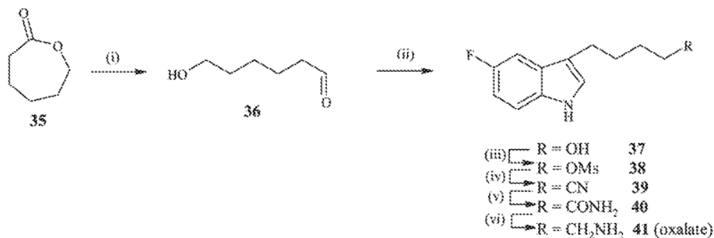
Scheme 6. Synthesis of Compound 41 a
