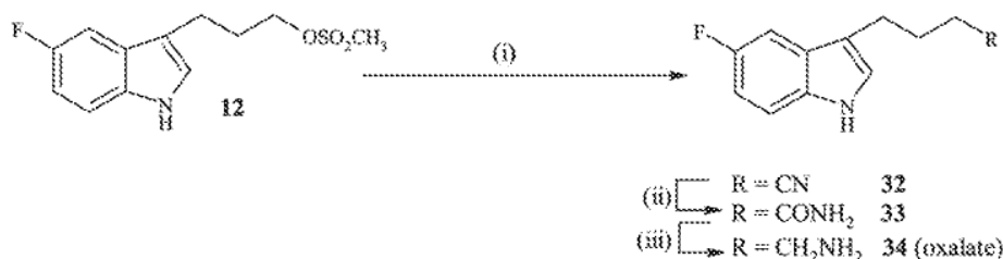
Scheme 5. Synthesis of Compound 34 a
