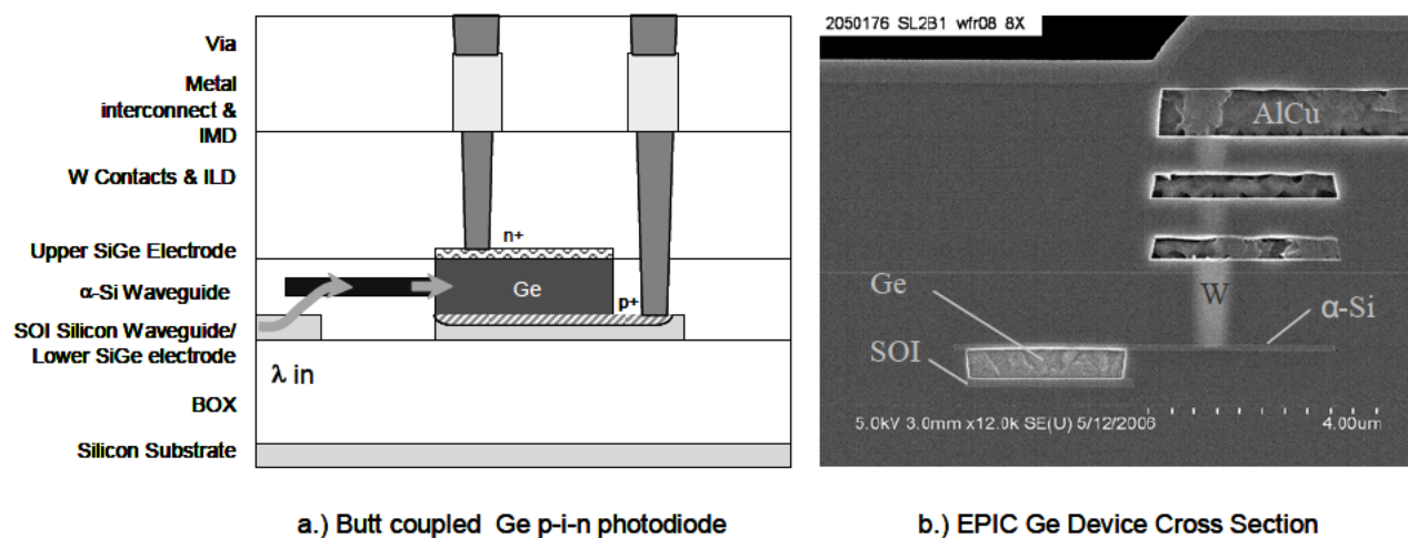
Figure 6. Waveguide integrated vertical Ge pin detector in CMOS process flow with butt coupled silicon waveguides using SOI silicon substrates.
