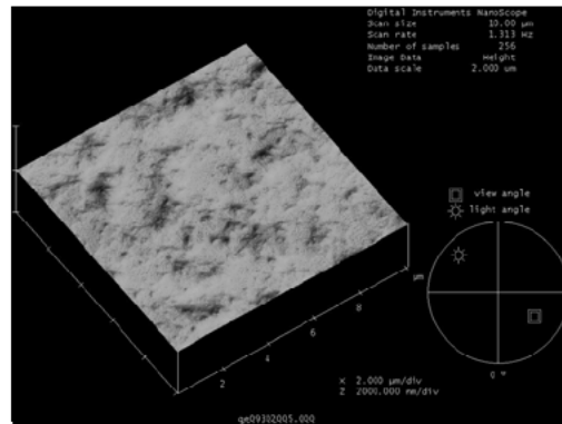
a.) AFM of as grown Ge Film on silicon
