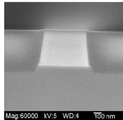
b.) RIE patterned Ge on silicon, oxide deposition fill & CMP
