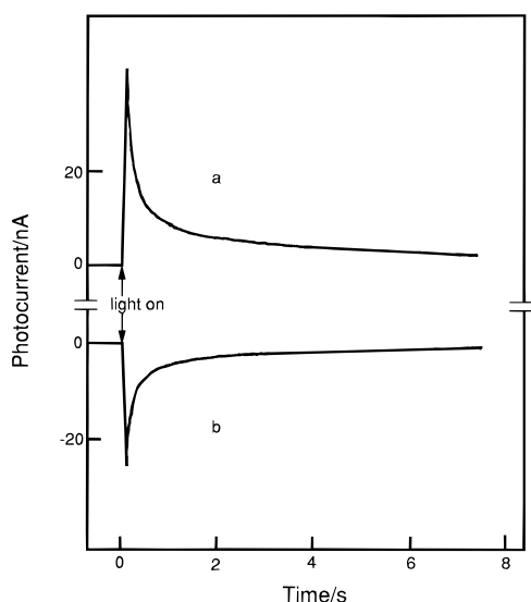
Figure 1. Short-circuit photocurrent of an ITO/ZnODEP/ITO cell as a function of time with a constant irradiation of 550 nm light after irradiation of the cell with a 550 nm light beam under a bias of (a) -2 or (b) +2 V for 5 s followed by a rest period of 10 s under short-circuit conditions in the dark.
