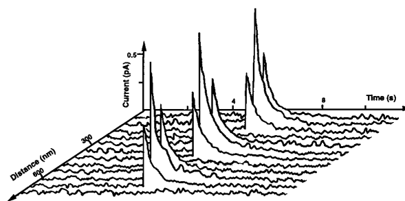
Figure 11. Discharge current as a function of time and distance. Charges were stored under a bias of 10 \text{ V} .
