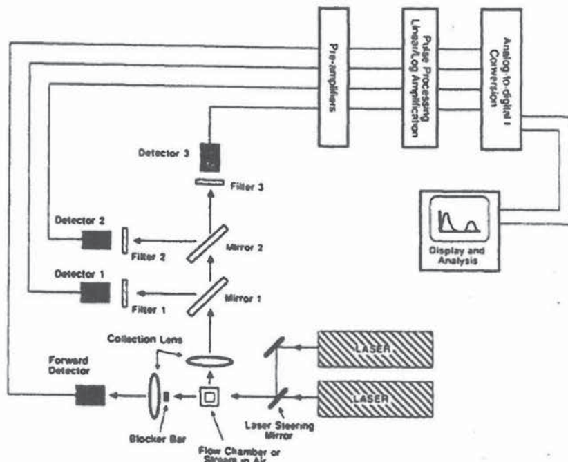
Figure 4 A generalized flow cytometer system.
