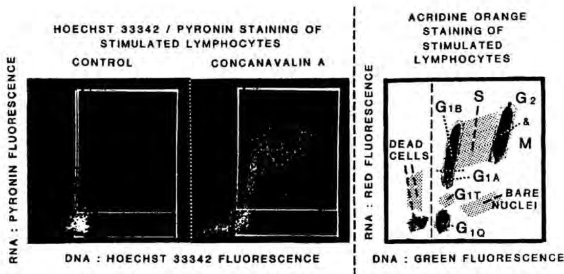
Figure 7-16. DNA and RNA content analysis of mitogen-stimulated lymphocytes. Left: typical results using the combination of Hoechst 33342 and pyronin Y described by the author 10 . Right: Typical results with acridine orange as described by Darzynkiewicz et al 262 , showing cell cycle compartments defined on the basis of DNA and RNA content.
