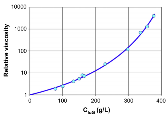
Fig. 4. Variations of the IgG relative viscosity as a function of IgG concentration. The solid line is the result of the Mooney fit.
