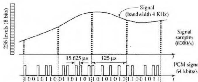
Figure 24.3-3 An example of PCM. A 4-kHz voice signal is sampled at a rate of 8 \times 10^3 samples per second. Each sample is quantized to 2^8 = 256 levels and represented by 8 bits, so that the signal is a sequence of bits transmitted at a rate of 64 kb/s.
