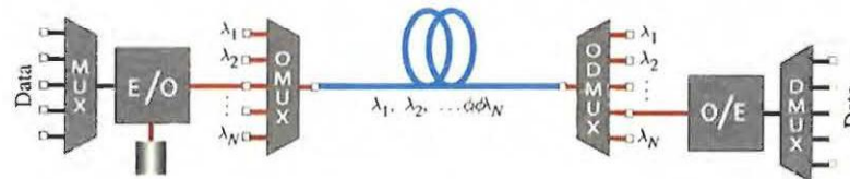
Figure 24.3-9 Wavelength division multiplexing (WDM).
