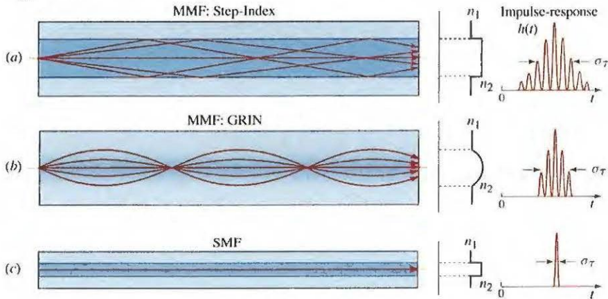
Figure 24.1-1 (a) Step-index multimode fibers (MMF): relatively large core diameter; uniform refractive indexes in the core and cladding; large pulse spreading due to modal dispersion. (b) Graded-index (GRIN) MMF: refractive index of the core is graded; there are fewer modes; pulse broadening due to modal dispersion is reduced. (c) Single-mode fibers (SMF): small core diameter; no modal dispersion; pulse broadening is due only to material and waveguide dispersion.
