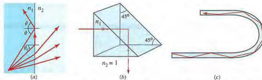
Figure 1.2-9 (a) Total internal reflection at a planar boundary. (b) The reflecting prism. If n_1 > \sqrt{2} and n_2 = 1 (air), then \theta_c < 45^\circ ; since \theta_1 = 45^\circ , the ray is totally reflected. (c) Rays are guided by total internal reflection from the internal surface of an optical fiber.
