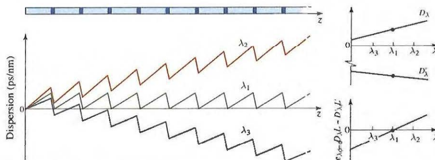
Figure 24.2-16 Perfect dispersion compensation at \lambda_1 , and imperfect dispersion compensation with net positive and negative dispersion at \lambda_2 and \lambda_3 , respectively. The error e_\lambda vanishes if the slopes of D_\lambda and D'_\lambda are equal.
