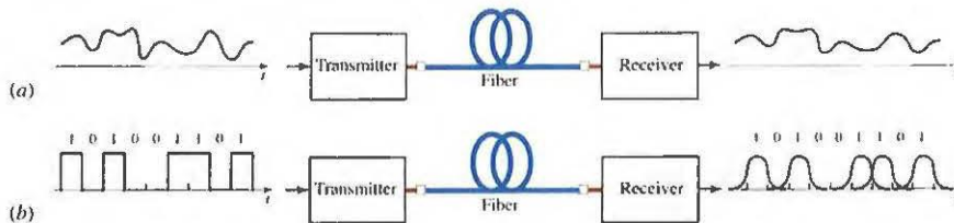
Figure 24.2-1 Optical fiber communication systems using intensity-modulation. (a) Analog system: the power of the light source is proportional to the signal, which is a continuous function of time representing, e.g., an audio or video waveform. (b) Digital ON-OFF keying: bits “1” and “0” are represented, respectively, by the presence and absence of an optical pulse.
