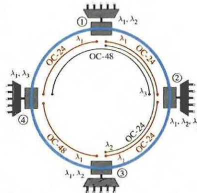
Figure 24.4-10 A schematic of a 4-node 3-channel WDM ring network.
