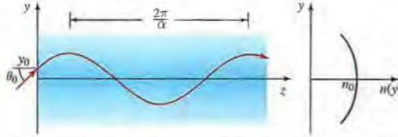
Figure 1.3-4 Trajectory of a ray in a GRIN slab of parabolic index profile (SELFOC).
