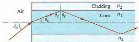
Figure 1.2-18 Acceptance angle of an optical fiber.
