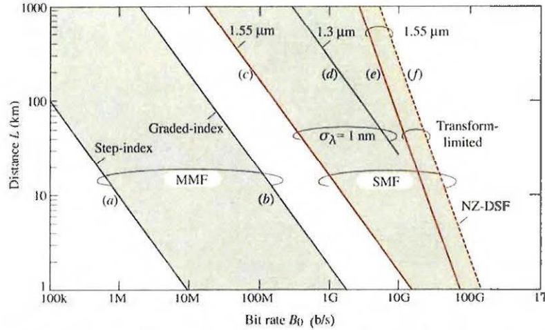
Figure 24.2-12 Dispersion-limited maximum fiber length L as a function of the bit rate B_0 for multimode fibers (MMF) and single-mode fibers (SMF). Six lines are shown (left to right): (a) MMF, step-index ( n_1 = 1.46 , \Delta = 0.01 ), LB_0 = 10 km-Mb/s; (b) MMF, graded-index with parabolic profile ( n_1 = 1.46 , \Delta = 0.01 ), LB_0 = 2 km-Gb/s; (c) SMF limited by material dispersion, operating at 1550 nm with D_\lambda = 17 ps/km-nm and \sigma_\lambda = 1 nm, B_0L \approx 15 km-Gb/s; (d) SMF limited by material dispersion, operating at 1300 nm with |D_\lambda| = 1 ps/km-nm and \sigma_\lambda = 1 nm, B_0L = 250 km-Gb/s; (e) SMF with transform limited pulses operating at 1550 nm with |D_\lambda| = 17 ps/km-nm; (f) same as (e) with non-zero dispersion-shifted fiber (NZ-DSF) with chromatic dispersion coefficient D_\lambda = 1 ps/km-nm.
