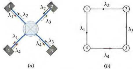
Figure 24.4-6 A WDM network in a star physical topology (a) is equivalent to the ring logical topology (b).
