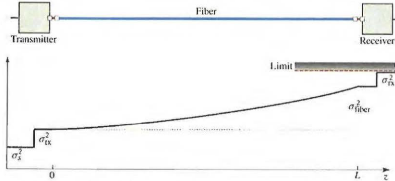
Figure 24.2-11 Budget for the pulse temporal width.
