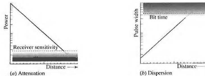
Figure 24.2-5 (a) Dependence of the optical power on the distance. (b) Dependence of the pulse width on the distance. The maximum length of the optical link is set by either (a) attenuation, when the received power drops below the receiver sensitivity, or (b) dispersion, when the pulse width exceeds the bit time.
