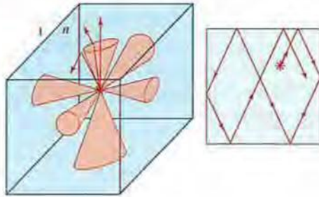
Figure 1.2-19 Trapping of light in a parallelepiped of high refractive index.
