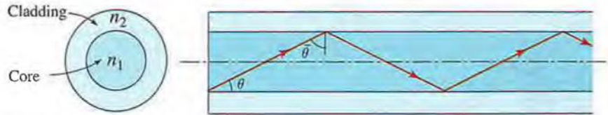
Figure 1.2-17 The optical fiber. Light rays are guided by multiple total internal reflections. Here \theta represents the angle measured from the axis of the optical fiber so that its complement \bar{\theta} = 90^\circ - \theta is the angle of incidence at the dielectric interface.
