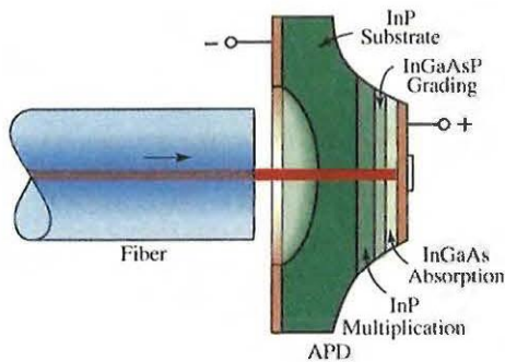
Figure 24.1-6 Structure of a separate-absorption-grading-multiplication (SAGM) APD.
