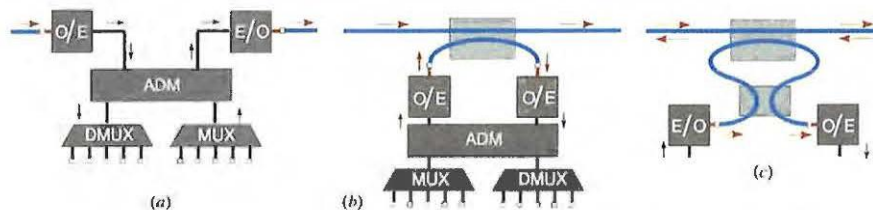
Figure 24.4-3 Interface between the node and the fiber network. (a) Opaque interface. The signal is converted from optical to electronic (O/E) and the ADM extracts data and adds new data, which is used to generate a new optical signal (E/O). (b) Optically coupled (transparent) interface using a directional coupler. (c) Optically coupled interface to a duplex fiber using two directional couplers.
