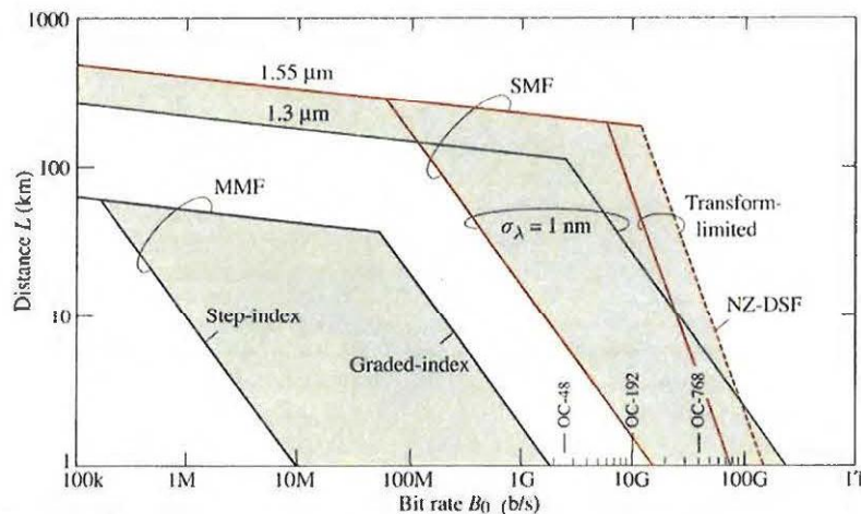
Figure 24.2-13 Maximum distance L versus bit rate B_o for six cases of fibers. This graph is obtained by superposing the graphs in Figs. 24.2-10 and 24.2-12. Each line represents the maximum distance L of the link at each rate B_o that satisfies both the attenuation and dispersion limits, i.e., guarantees the reception of the required power and pulse width at the receiver.
