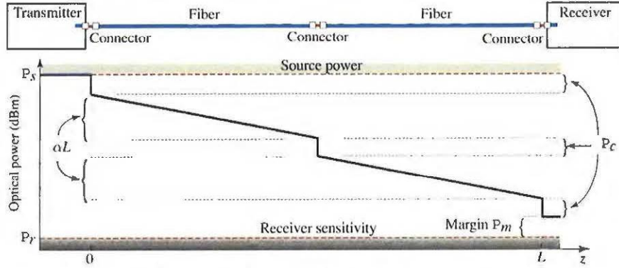
Figure 24.2-8 Power budget of an optical link.
