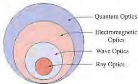
Figure 1.0-1 The theory of quantum optics provides an explanation of virtually all optical phenomena. The electromagnetic theory of light (electromagnetic optics) provides the most complete treatment of light within the confines of classical optics. Wave optics is a scalar approximation of electromagnetic optics. Ray optics is the limit of wave optics when the wavelength is very short.
