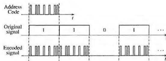
Figure 24.3-8 CDM encoding.
