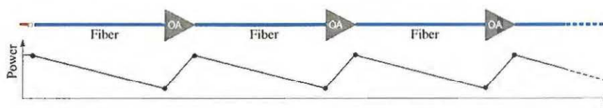
Figure 24.2-14 Compensation of attenuation by use of optical fiber amplifiers.
