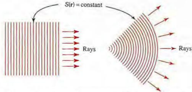
Figure 1.3-10 Rays and surfaces of constant S(\mathbf{r}) in a homogeneous medium.
