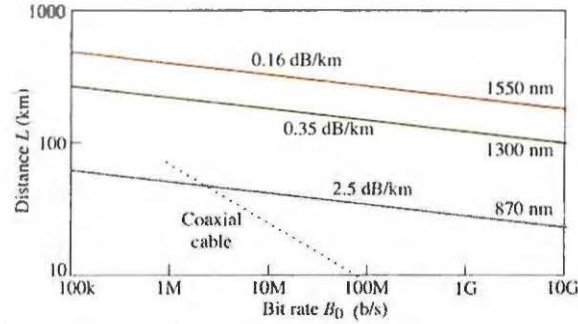
Figure 24.2-10 Maximum fiber length L as a function of bit rate B_0 under attenuation-limited conditions for a fused silica-glass fiber operating at wavelengths \lambda_o = 870, 1300 and 1550 nm assuming fiber attenuation coefficients \alpha = 2.5, 0.35 , and 0.16 dB/km, respectively; source power P_s = 1 mW ( P_s = 0 dBm); receiver sensitivity \bar{n}_o = 300 photons/bit for receivers operating at 870 and 1300 nm and \bar{n}_o = 1000 for the receiver operating at 1550 nm; and P_c = P_m = 0 . For comparison, the L - B_0 relation for a typical coaxial cable is also shown.
