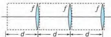
Figure 1.4-7 A periodic sequence of lenses.
