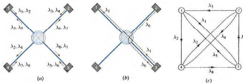
Figure 24.4-7 (a) A WDM multi-hop broadcast-and-select network. (b) A two-hop connection from node 1 to node 2 via node 3. (c) Logical topology of the network.
