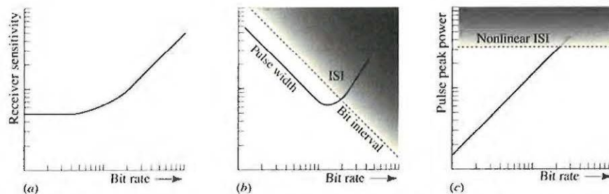
Figure 24.2-6 Effect of bit rate on (a) receiver sensitivity, (b) pulse width at the receiver, and (c) peak power. At higher bit rate, the communication system is more sensitive to attenuation, dispersion, and nonlinear effects.
