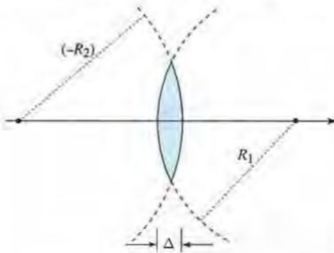
Figure 1.2-13 A biconvex spherical lens.
