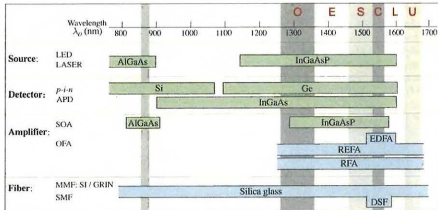
Figure 24.2-3 Types and materials of optical sources, detectors, amplifiers, and fibers used at various wavelengths. The first generations of optical links operated at wavelengths near 870 nm, 1310 nm, and 1550 nm.
