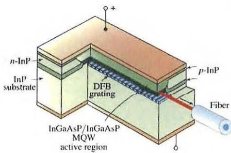
Figure 24.1-4 Buried-heterostructure multi-quantum-well distributed-feedback laser used for optical fiber communications. The dielectric film provides gain guiding while the alternating p and n -type layers allow current flow only in the vicinity of the active region. Lasers such as these offer ample gain at modest current levels, and provide output powers of 1 W or more in a single spatial mode. Typical values of the threshold current and differential responsivity are i_t < 10 \text{ mA} and \mathcal{R}_d \approx 0.4 \text{ W/A} , respectively.
