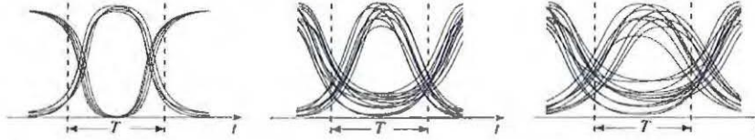
Figure 24.2-7 Closing of the eye diagram (left to right) as a result of noise and pulse broadening.
