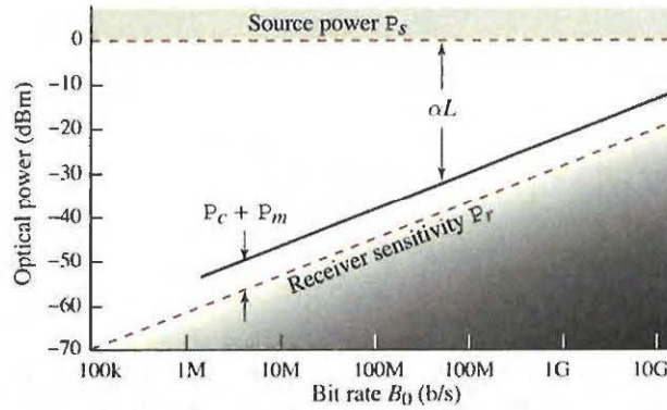
Figure 24.2-9 Power budget as a function of bit rate B_0 . As B_0 increases, the power P_r required at the receiver increases (so that the energy per bit remains constant), and the maximum length L decreases.
