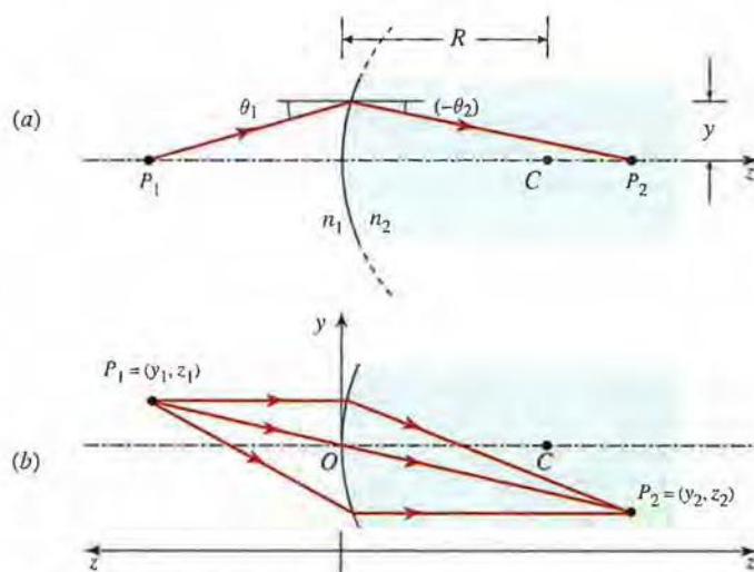
Figure 1.2-12 Refraction at a convex spherical boundary ( R > 0 ).
