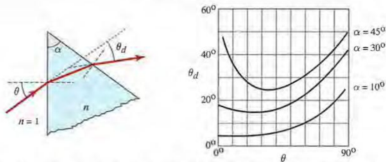
Figure 1.2-10 Ray deflection by a prism. The angle of deflection \theta_d is a function of the angle of incidence \theta for different apex angles \alpha when n = 1.5 . When both \alpha and \theta are small \theta_d \approx (n - 1)\alpha , which is approximately independent of \theta . When \alpha = 45^\circ or \theta = 0^\circ , total internal reflection occurs, as illustrated in Fig. 1.2-9(b).
