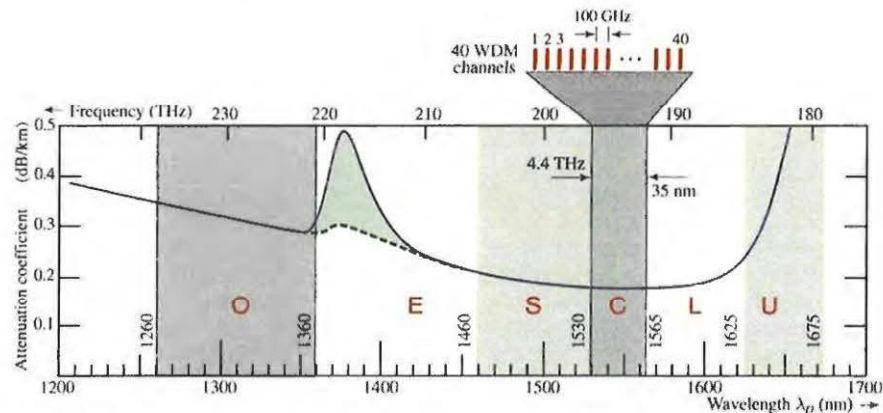
Figure 24.3-10 A 40-channel WDM system in the C spectral band, where fiber attenuation is minimal. The channel spacing is 100 GHz.
