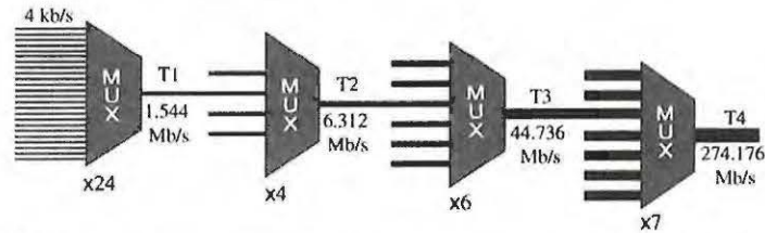
Figure 24.3-7 The T-system. A set of 24 4-kb/s signals are multiplexed by a TDM generating a T1 composite signal at 1.544 Mb/s. Four such signals are multiplexed to generate a T2 signal, and so on.
