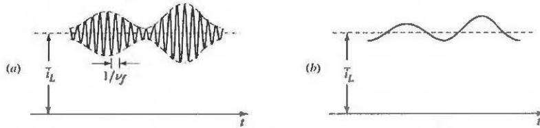
Figure 24.5-2 (a) Photocurrent generated by the heterodyne detector. The envelope and phase of the time-varying component carries complete information about the complex amplitude of the optical field representing the signal. (b) Photocurrent generated by the homodyne detector.
