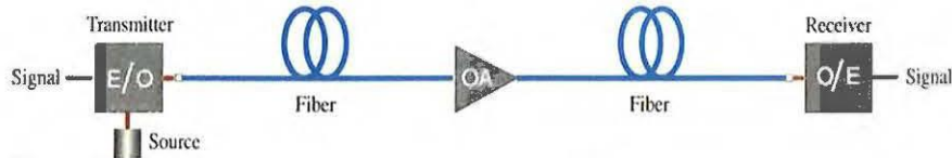
Figure 24.0-1 An optical fiber communication system. An electrical signal is converted into an optical signal (E/O) by modulating an optical source. The optical signal is transmitted through the fiber to the receiver. At the receiver, the optical signal is converted back into an electrical signal by use of a detector and demodulator (O/E). For long fibers, optical amplifiers (OA) may be used to boost the weakened optical signal. Alternatively, several optical links may be cascaded to form a longer link by use of an intermediate process of electrical amplification and signal regeneration between adjacent links. Such units are called regenerators or repeaters .
