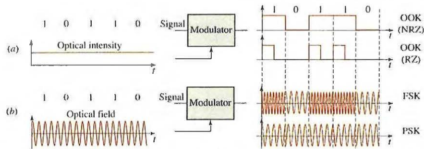
Figure 24.3-4 Examples of binary modulation of light: (a) ON-OFF keying intensity modulation (OOK/IM); (b) frequency shift keying (FSK) and phase shift keying (PSK) field modulation.
