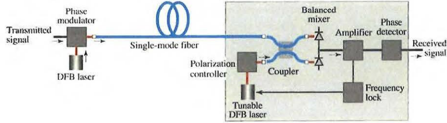
Figure 24.5-3 Coherent optical fiber communication system.
