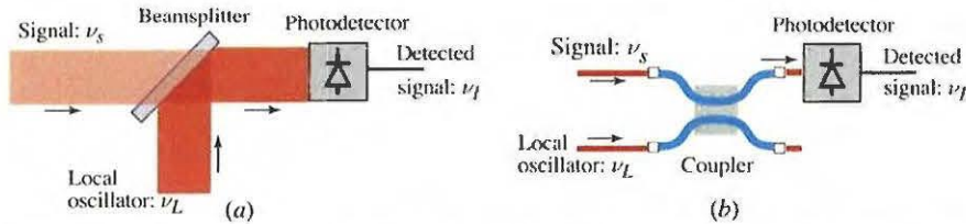
Figure 24.5-1 Optical heterodyne detection. A signal wave of frequency \nu_s is mixed with a local oscillator wave of frequency \nu_L using (a) a beamsplitter, and (b) an optical coupler. The photocurrent varies at the frequency difference \nu_I = \nu_s - \nu_L .
