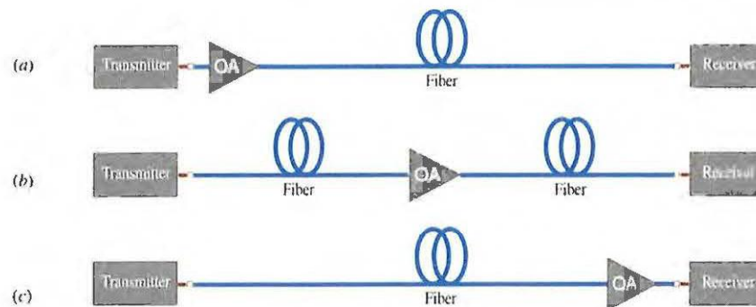
Figure 24.1-5 Optical fiber amplifiers are used in three configurations in an optical fiber communication system: (a) postamplifiers; (b) line amplifiers; and (c) preamplifiers.
