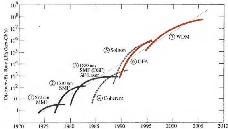
Figure 24.2-4 The history of optical fiber communication systems comprises continuous improvement of the bit rate distance product LB_0 .
