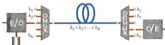
Figure 24.2-2 Wavelength-division multiplexing (WDM)
