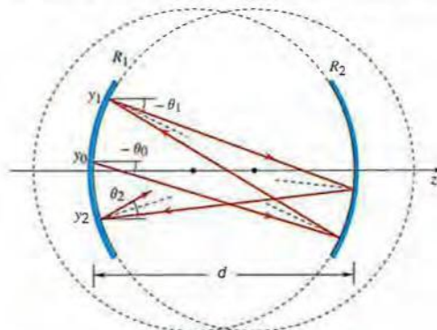
Figure 1.4-10 The optical resonator as a periodic optical system.
