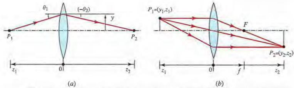
Figure 1.2-14 (a) Ray bending by a thin lens. (b) Image formation by a thin lens.
