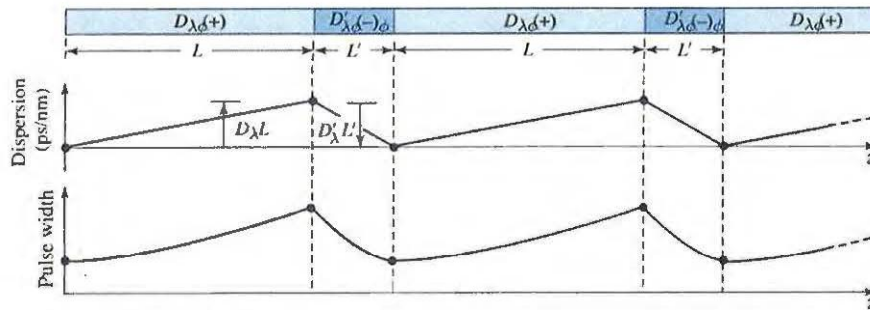
Figure 24.2-15 Dispersion compensation by use of fiber segments of opposite dispersion.
