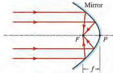
Figure 1.2-2 Focusing of light by a paraboloidal mirror.
