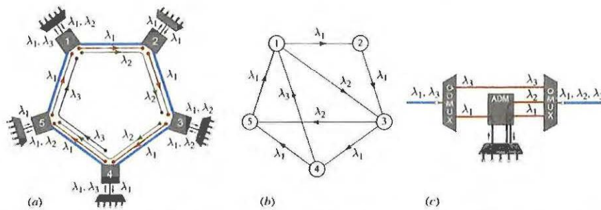
Figure 24.4-8 (a) A 5-node 3-channel wavelength-routed ring network. (b) Its logical topology. (c) An optical-add-drop multiplexer (OADM) used at node 5.
