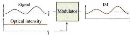
Figure 24.3-2 Intensity modulation.
