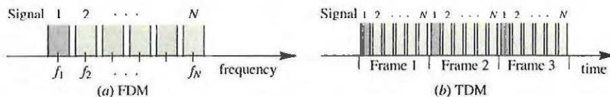
Figure 24.3-6 (a) In frequency-division multiplexing (FDM), a spectral band centered about a distinct frequency is allocated to each signal. (b) In time-division multiplexing, a sequence of time slots is allocated to each signal. The time slots of different signals are interleaved.
