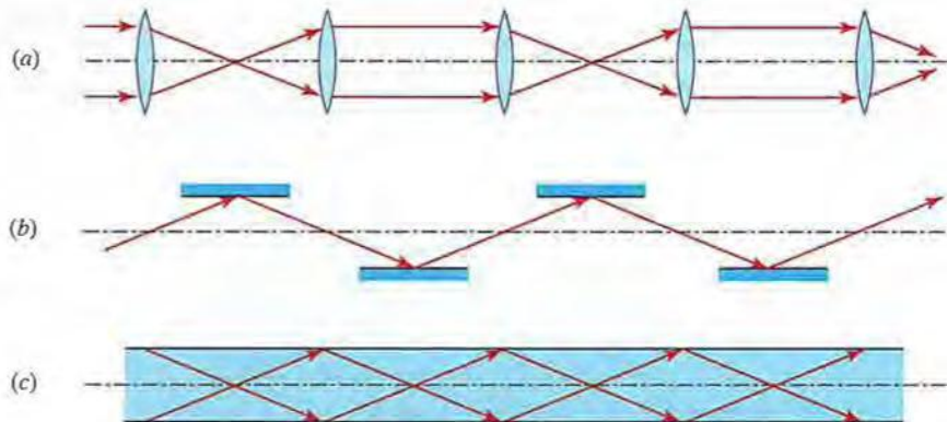
Figure 1.2-16 Guiding light: (a) lenses; (b) mirrors; (c) total internal reflection.
