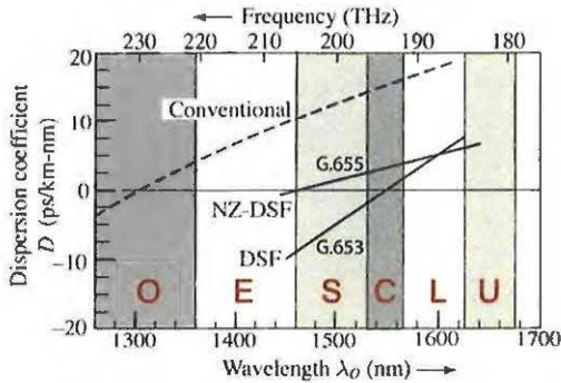
Figure 24.1-3 Wavelength dependence of the chromatic dispersion coefficient D of a conventional fiber and examples of a dispersion-shifted fiber (DSF) and non-zero-dispersion shifted fiber (NZ-DSF). The designations G.653 and G.655 are specifications of the ITU (International Telecommunications Union).
