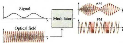
Figure 24.3-1 Amplitude and frequency modulation of the optical field.
