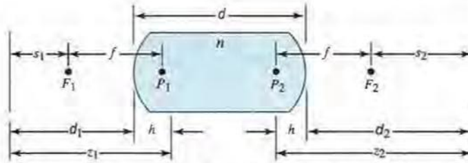
Figure 1.4-4 Imaging with a thick lens. P_1 and P_2 are the principal points and F_1 and F_2 are the focal points.
