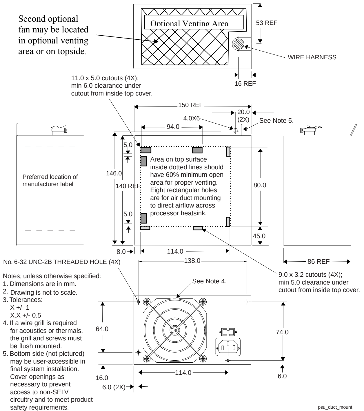
Figure 10. Power Supply Dimensions for Chassis That Require Top Venting
