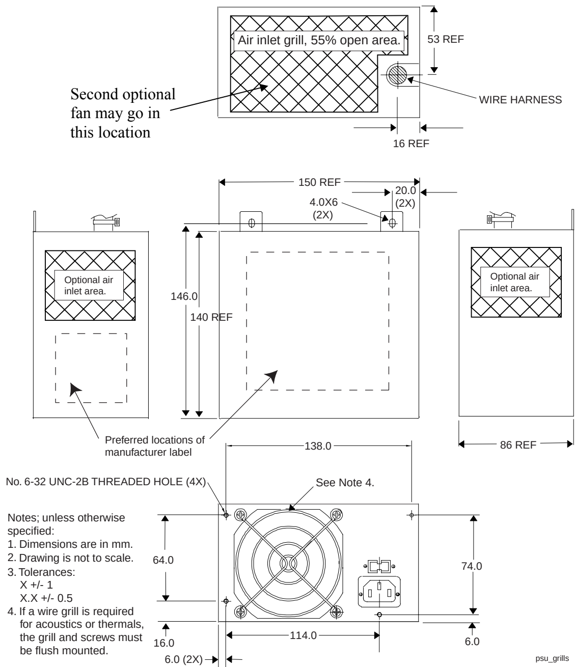
Figure 9. Power Supply Dimensions for Chassis That Does Not Require Top Venting
