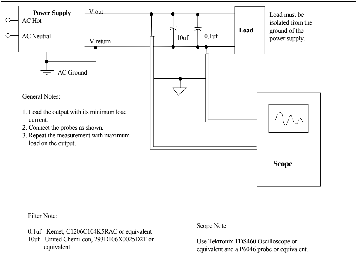
Figure 6. Differential Noise Test Setup
