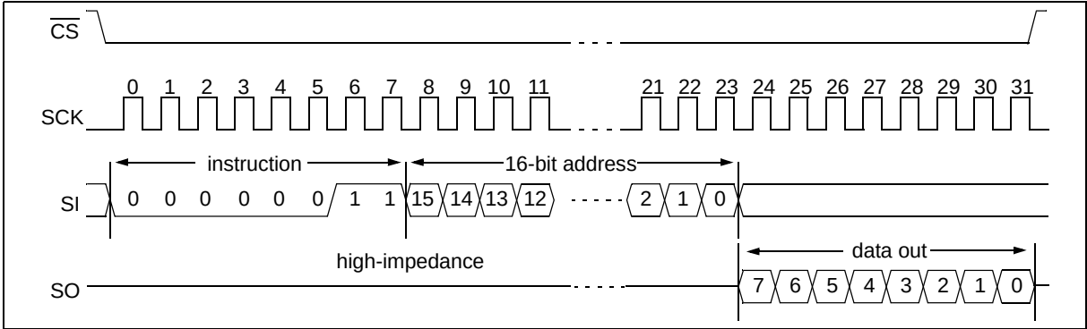
FIGURE 2-1: READ SEQUENCE
