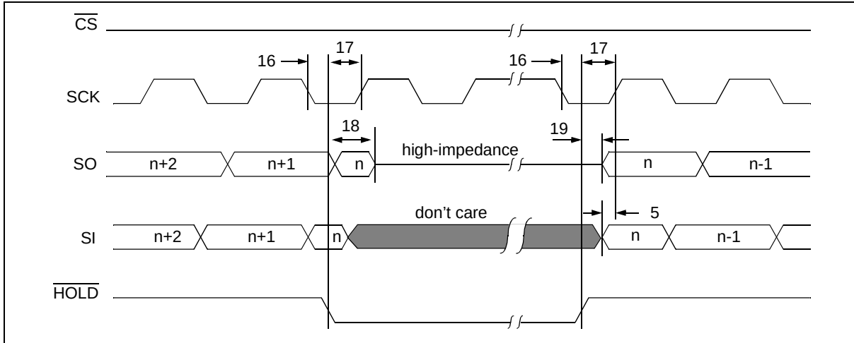
FIGURE 1-1: HOLD TIMING
