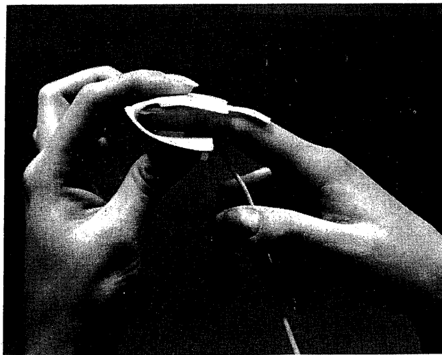
FIGURE 52.6 Disposable finger probe of a noninvasive pulse oximeter.
