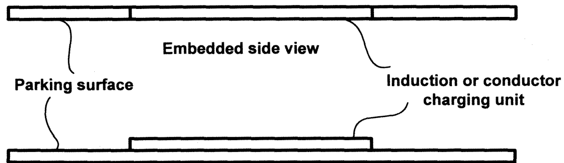
Overlay conversion kit option side view
