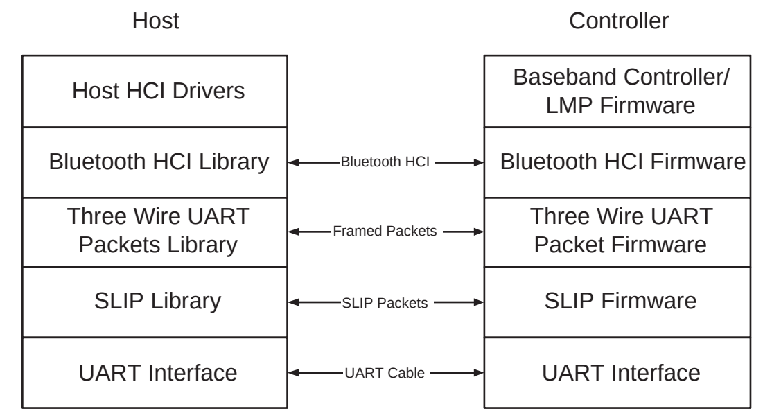
Figure 2.1: The Relationship Between the Host and the Controller
