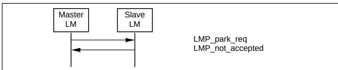
Sequence 80: Slave rejects to enter into park state
