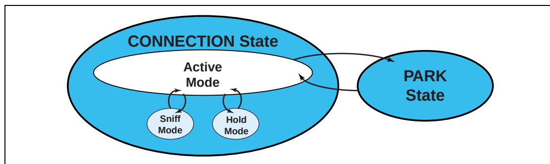
Figure 8.5: Connection state.
