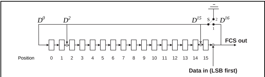
Figure 3.4: The LFSR circuit generating the FCS.
