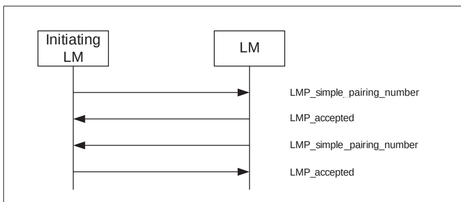
Sequence 59: Authentication OOB: Only one device is OOB-r capable
