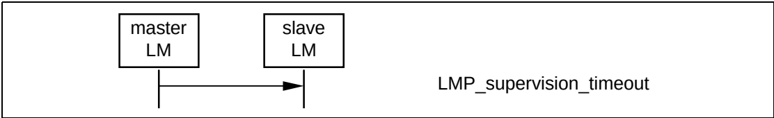
Sequence 10: Setting the link supervision timeout.
