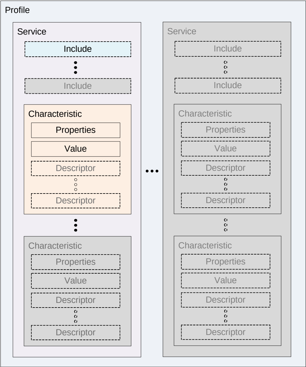
Figure 2.5: GATT Profile hierarchy
