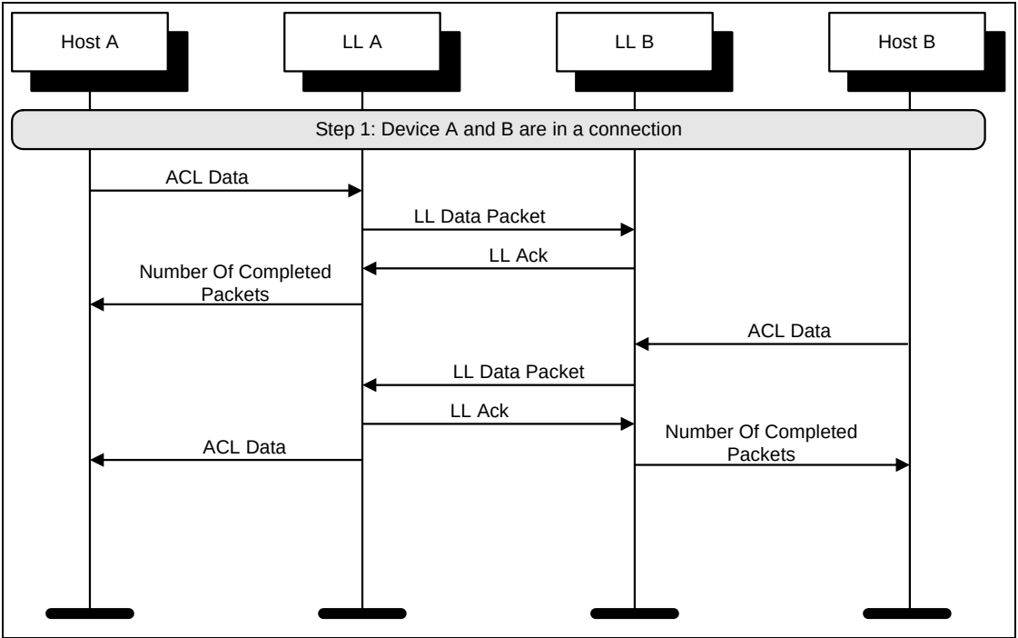
Figure 6.1: Sending Data
