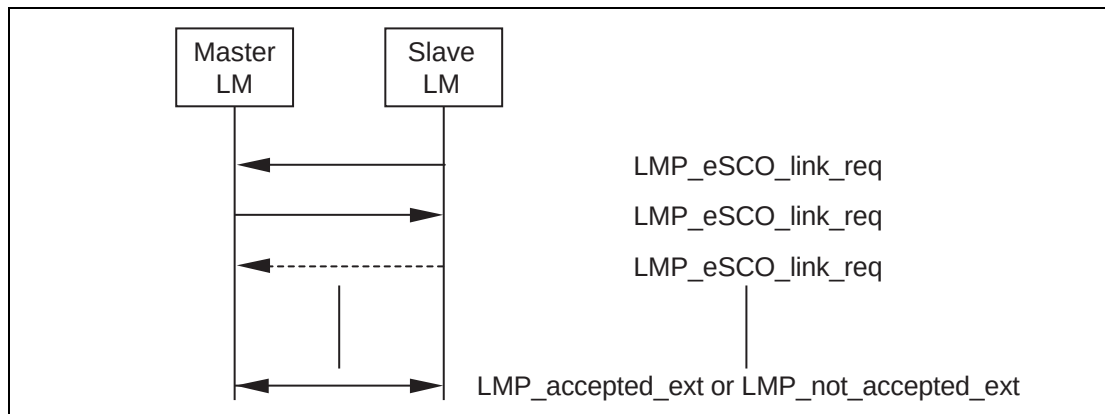
Sequence 96: Slave requests an eSCO link.
