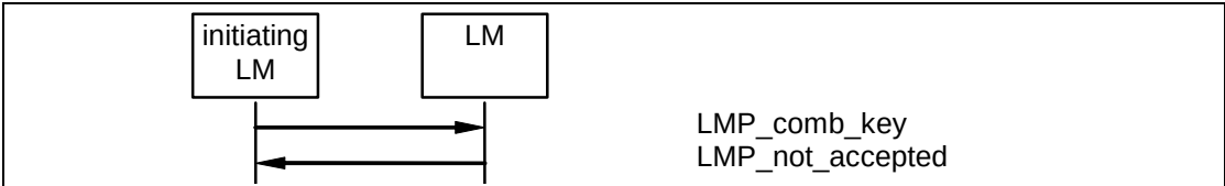
Sequence 32: Change of the link key not possible since the other device uses a unit key.
