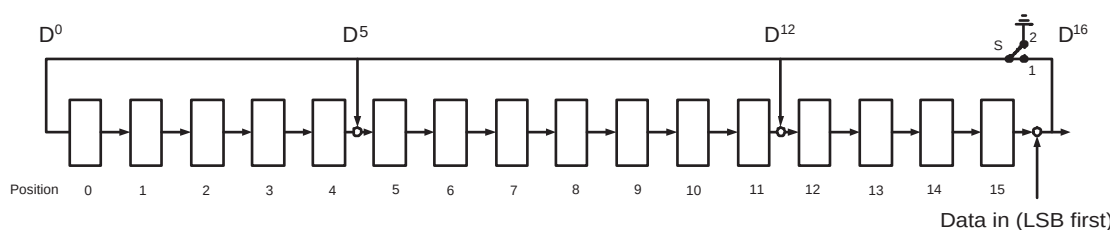
Figure 5.1: The LFSR Circuit Generating the CRC
