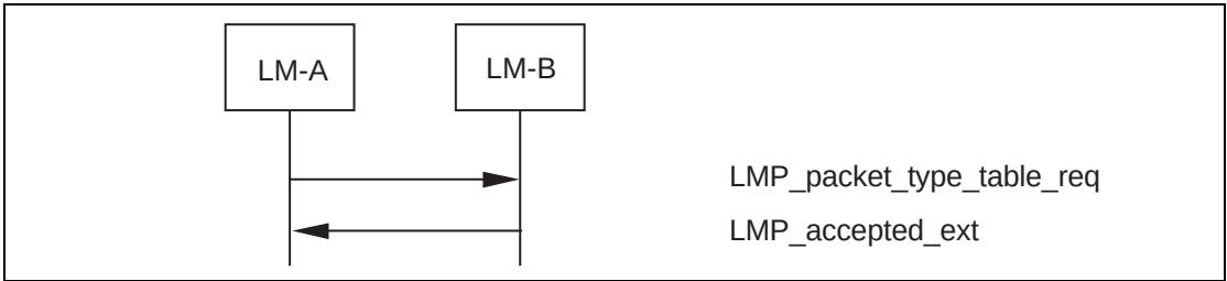
Sequence 22: Packet type table change is accepted.
