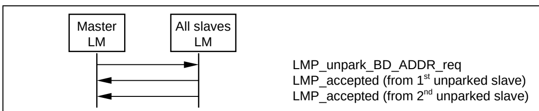
Sequence 86: Master unparks slaves addressed with their BD_ADDR
