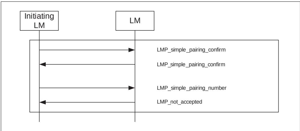
Sequence 54: Authentication Passkey Entry: Commitment check failure on the Responder side
