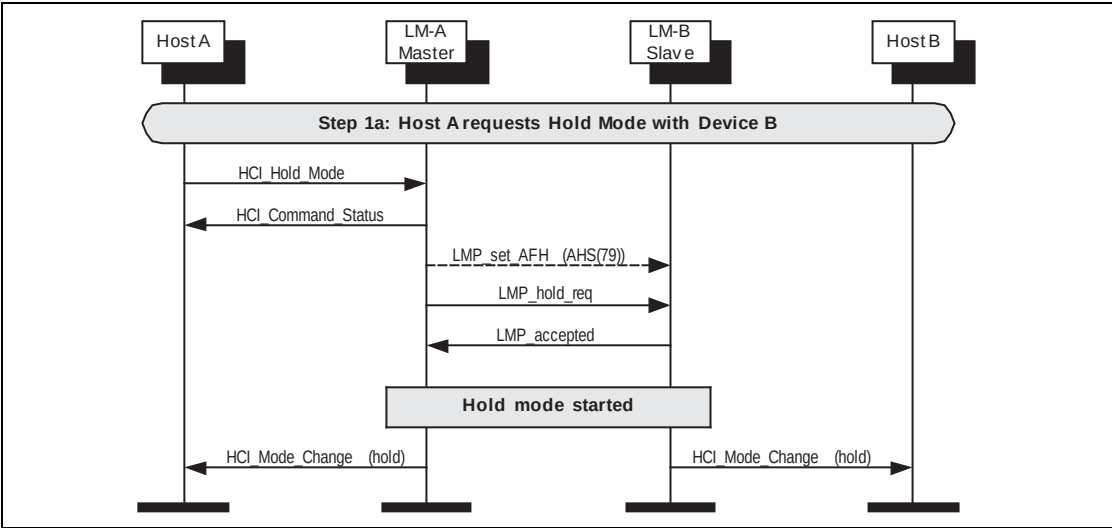
Figure 6.3: Hold request.
