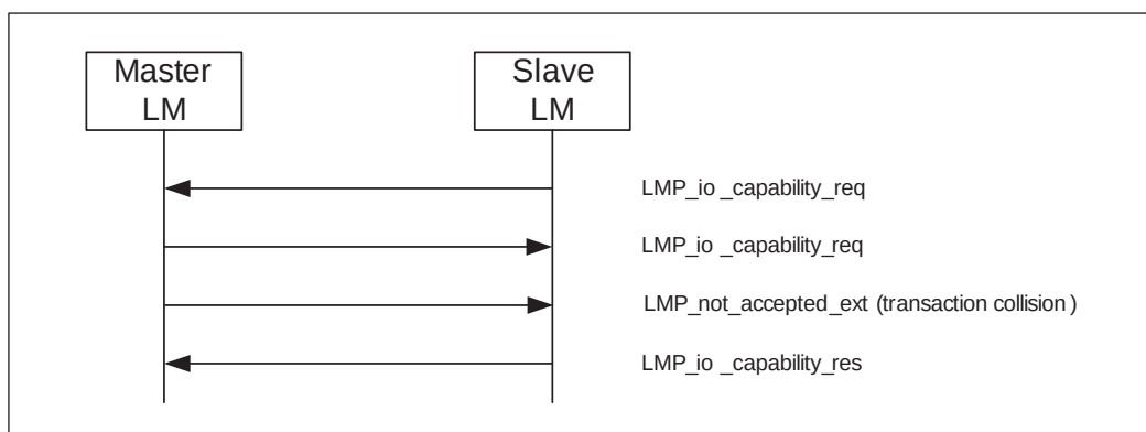
Sequence 47: IO Capability exchange with transaction Collision (slave transmitting LMP_io_capability_req first) and resolution
