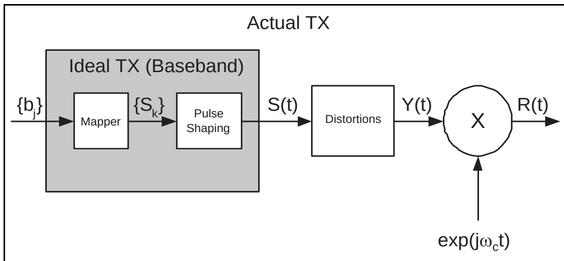
Figure 7.1: TX model.
