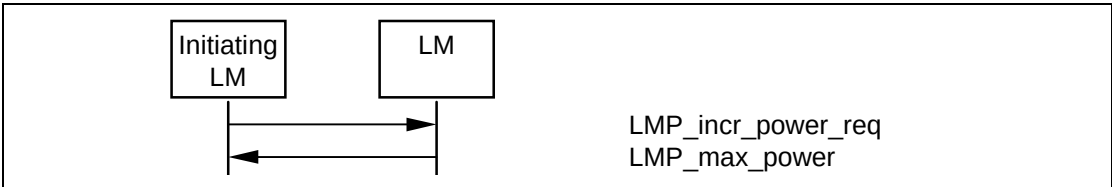
Sequence 3: The TX power cannot be increased.
