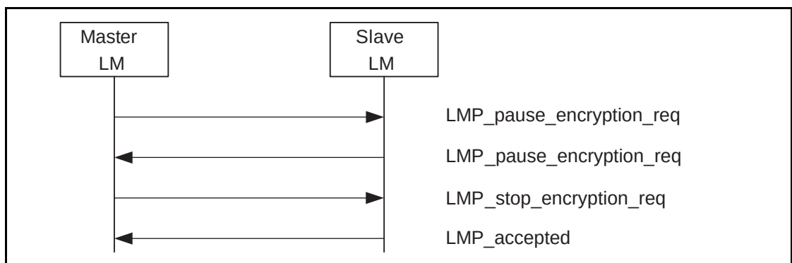
Sequence 40: Master-initiated pausing of encryption
