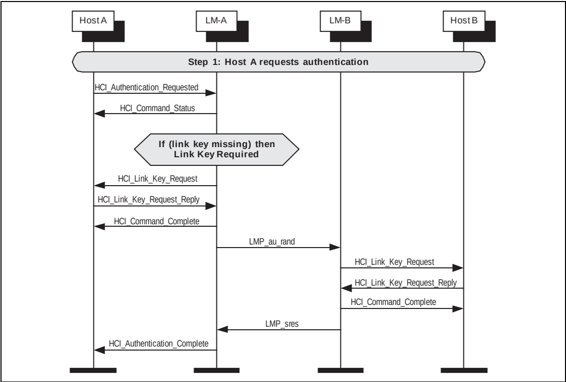
Figure 4.1: Authentication requested.
