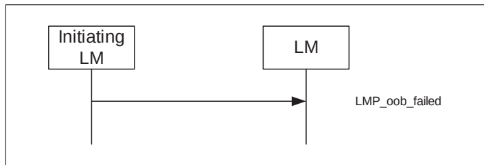
Sequence 62: Authentication stage 1 OOB: OOB information not available on the Initiator side
