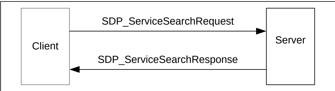
Figure 4.4: ServiceSearch Transaction
