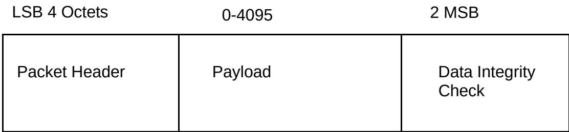
Figure 4.1: Packet Format
