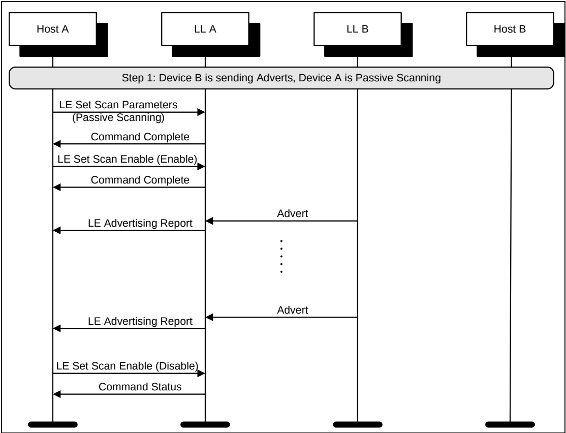
Figure 4.1: Passive Scanning
