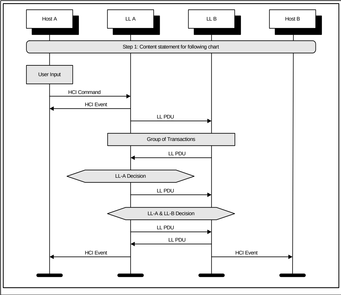
Figure 1.1: Example MSC
