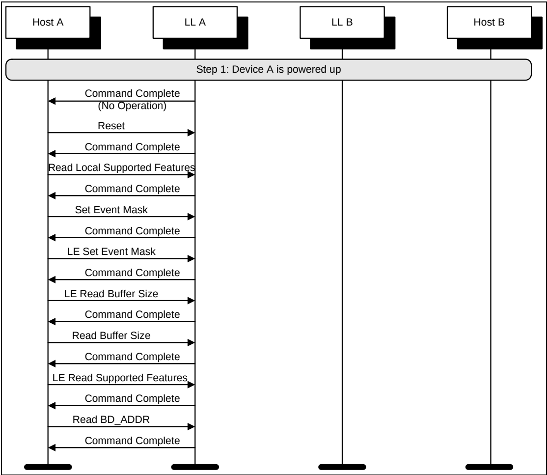
Figure 2.1: Initial Setup
