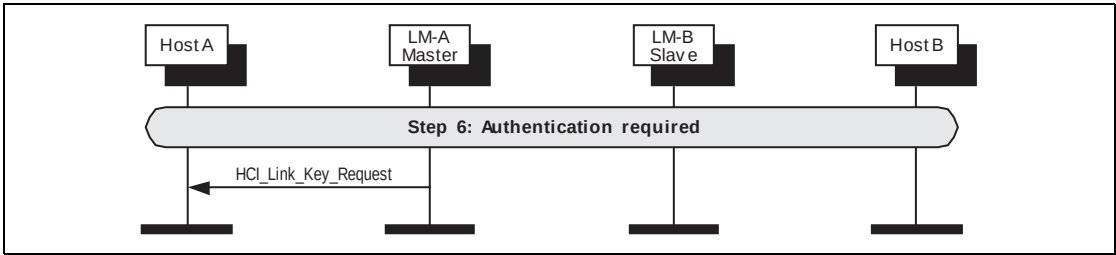
Figure 3.9: Authentication initiated.
