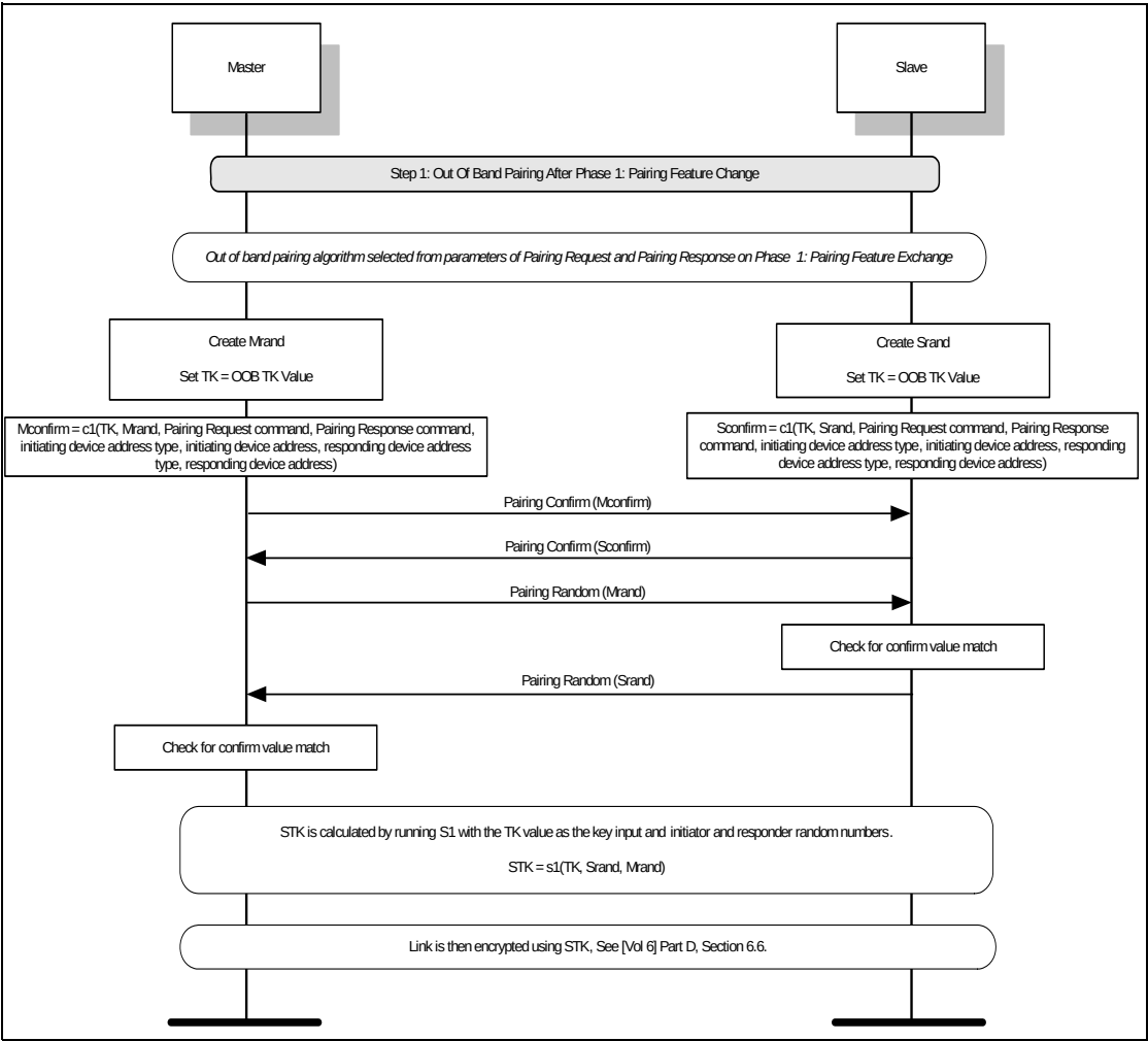
Figure 5.7: OOB Pairing Method
