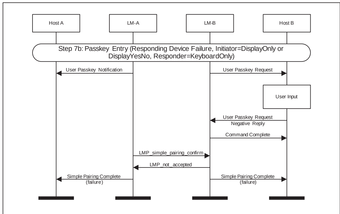
Figure 4.14: Passkey Entry Failure on Responding Side
