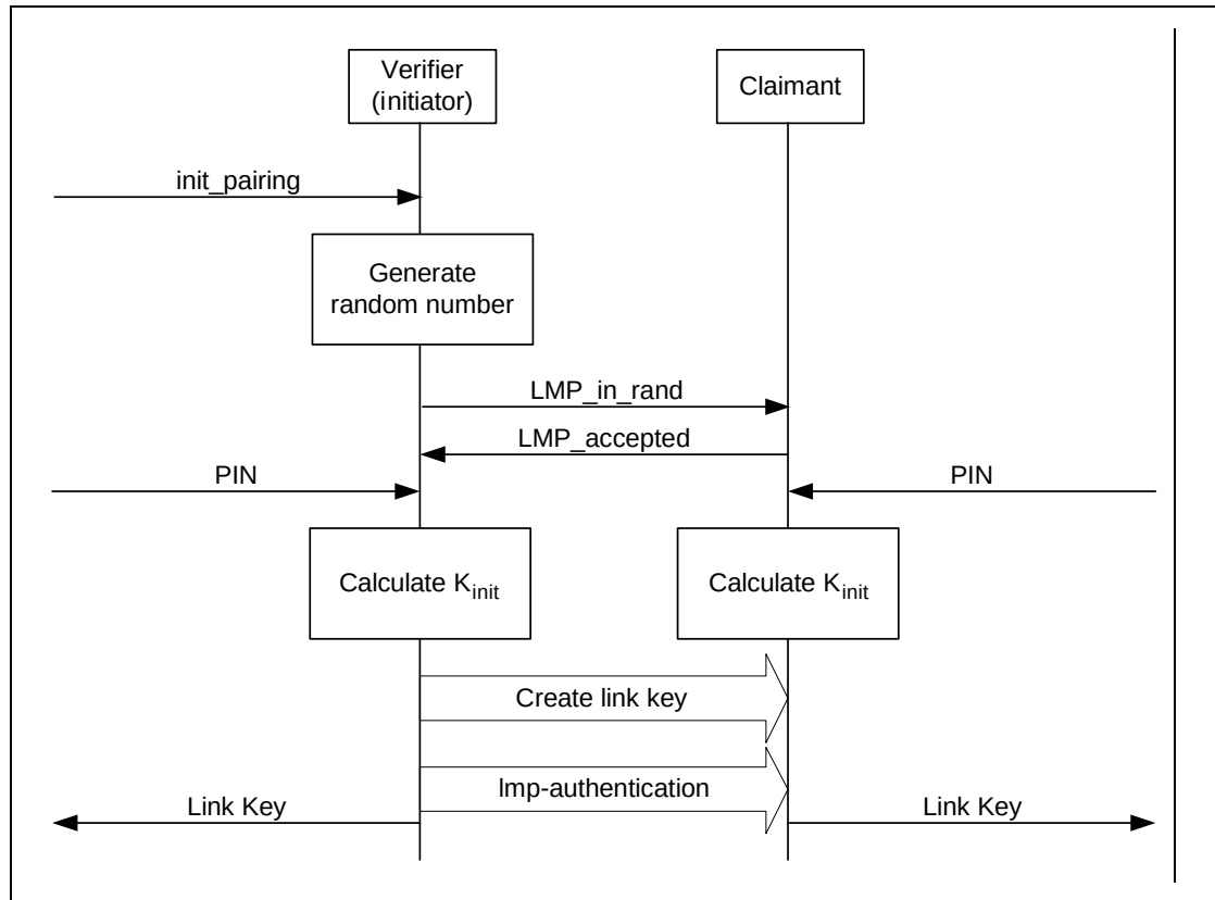
Figure 17.2: LMP-pairing as defined in [2].
