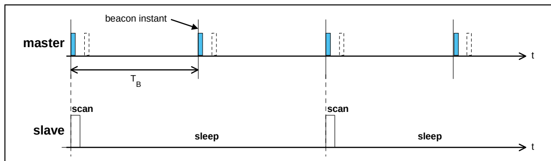
Figure 8.18: Extended sleep interval of parked slaves.
