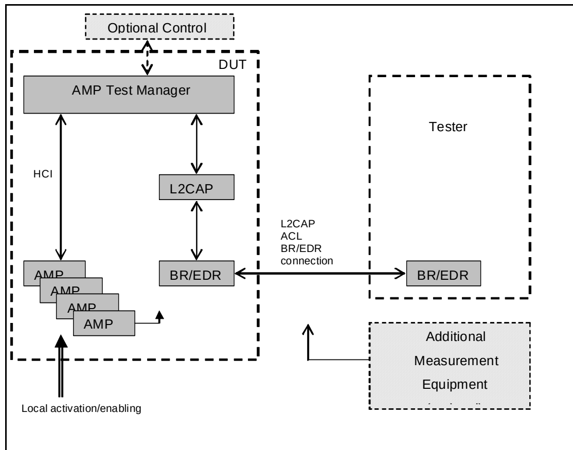
Figure 1.10: Test Architecture
