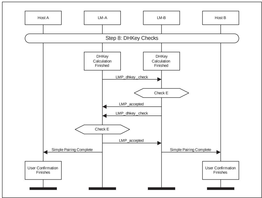
Figure 4.18: DHKey Checks
