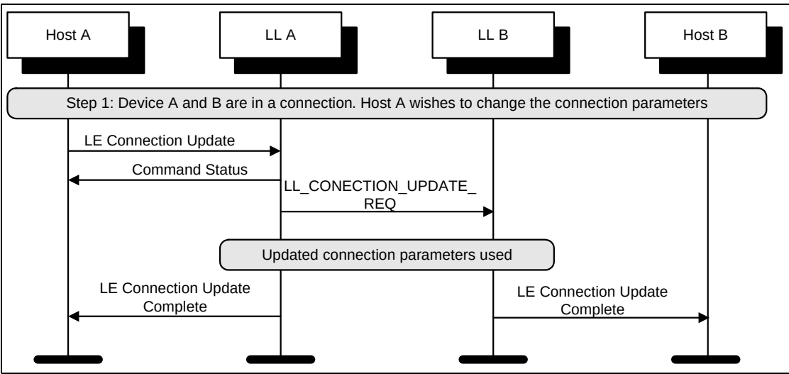
Figure 6.2: Connection Update
