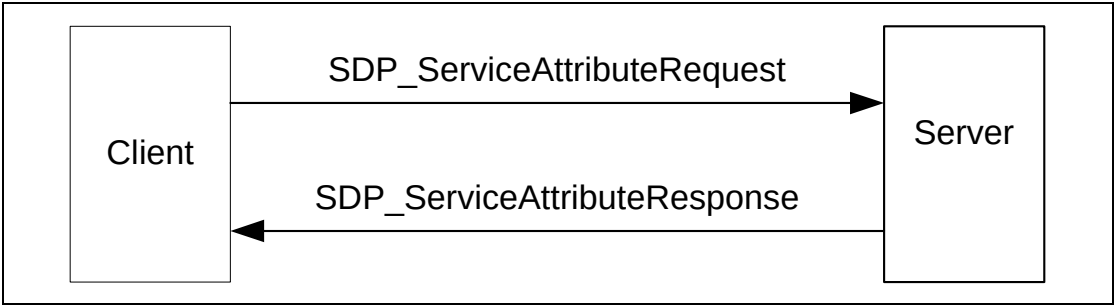
Figure 4.5: ServiceAttribute Transaction
