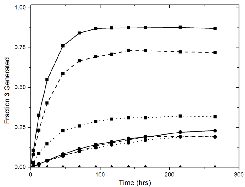
Figure 4. Fraction of 3 generated from (■) 1a (●) 1b (▲) 1c (at the baseline) in the presence of (—) 10mM, (---) 1.0mM, and (···) 0.1mM GSH.
