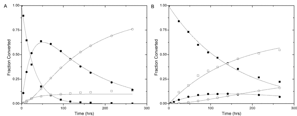
Figure 3. Relative HPLC measured concentrations for 1a (panel A) and 1b (panel B) over time, with constructed curves using derived rate constants and equations 5–8 for (■) 1 (a or b) (□) 1 RO (●) 3 and (○) 3 RO .
