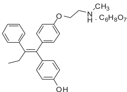
Figure 1 Chemical structure of endoxifen.
