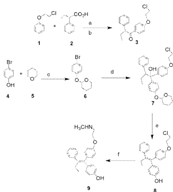
Scheme 1. Reagents and conditions: (a) method; (i) 2 , \text{SOCl}_2 , EDC; 3 , \text{AlCl}_3 , EDC; (b) method; (ii) TFAA, rt; (c) concd \text{H}_2\text{SO}_4 , rt; (d) (i) 6 , Mg, THF; reflux→rt; (ii) add 3 in THF, reflux; (e) concd HCl, MeOH, reflux; (f) methylamine, 2-propanol, reflux.
