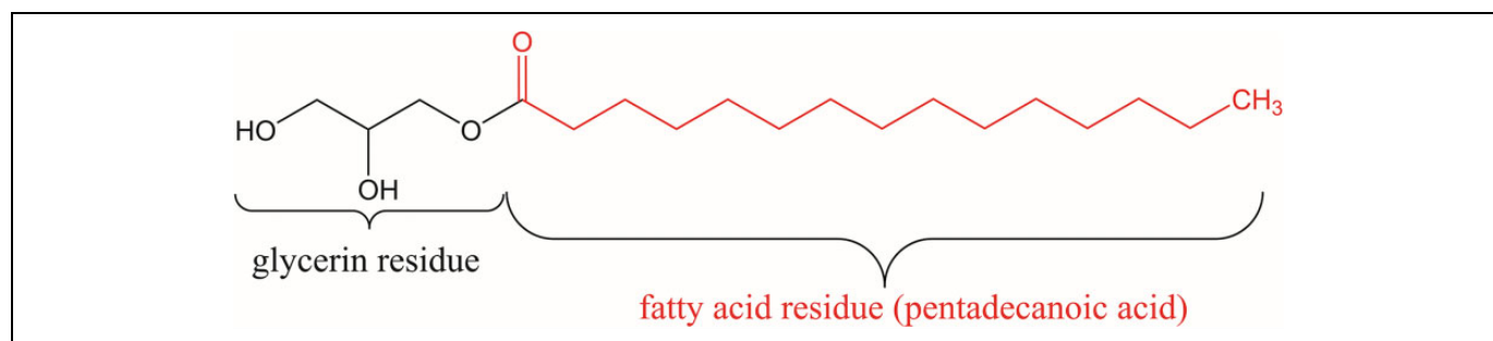
Figure 1. Glyceryl Pentadecanoate, a monoglyceride monoester.
