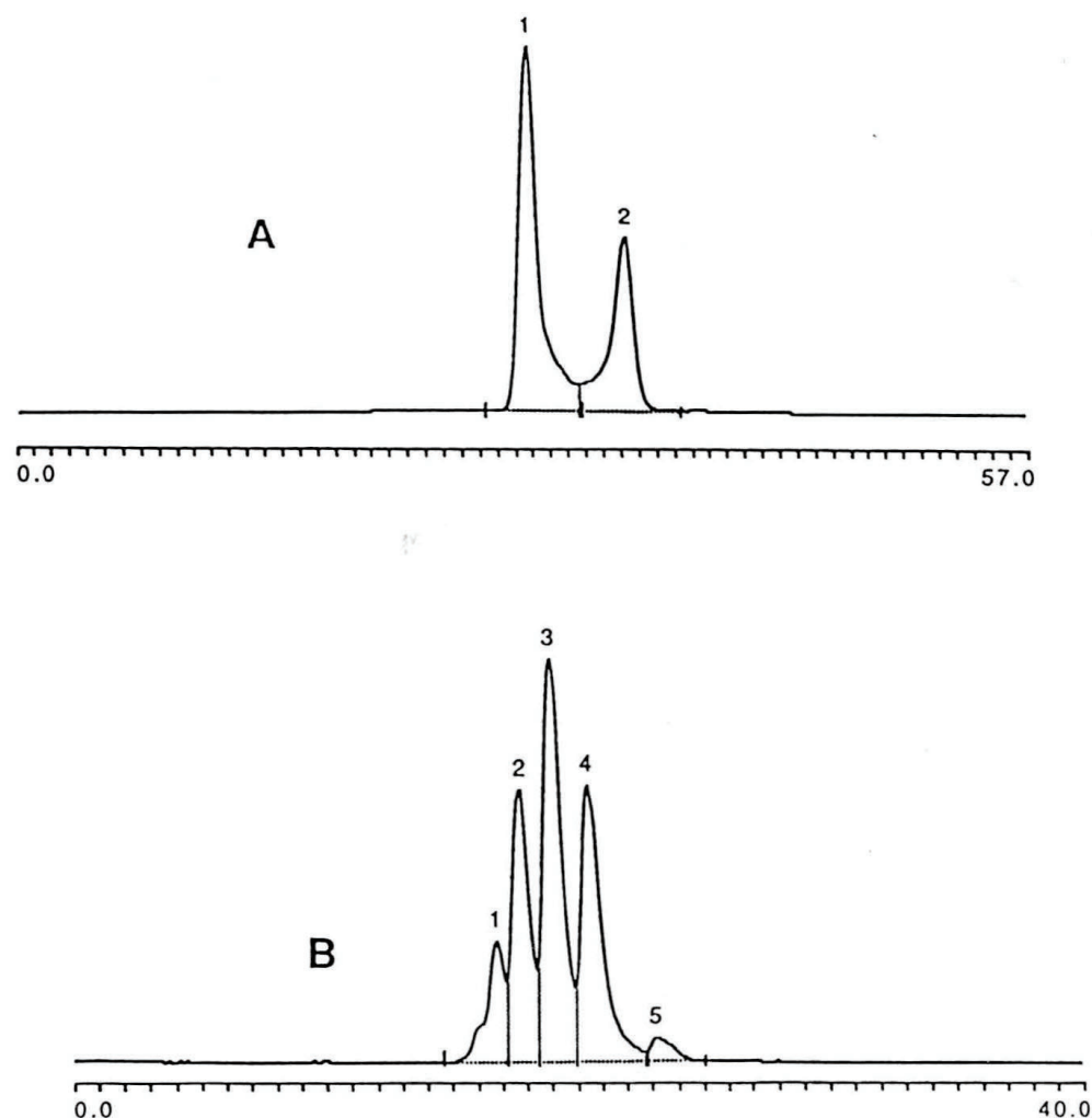
Figure 4. (A) PolyCAT A cation-exchange HPLC chromatographic separation of a 5 mg/ml sample of 4-4-20/212 scFv showing monomer (peak 1) and dimer (peak 2). Retention times of peaks 1 and 2 are 28.9 and 34.4 min, respectively. (B) HPLC size-exclusion chromatograph analysed on a TSK G3000SW column showing a highly aggregated CC49/212 scFv. The monomer (peak 4), dimer (peak 3), and trimer (peak 2) fractions elute at 20.4, 18.9, and 17.7 min, respectively.
