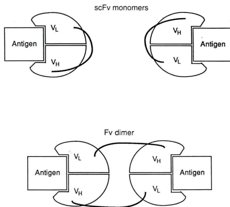
Figure 1. Schematic depiction of V_L/V_H rearrangement model. Top: Two single-chain Fv proteins bound to antigens. Linker peptides shown in bold print. Bottom: An scFv dimer with interchain V_L-V_H interfaces formed by V_L and V_H domains from two scFv monomer polypeptides.
