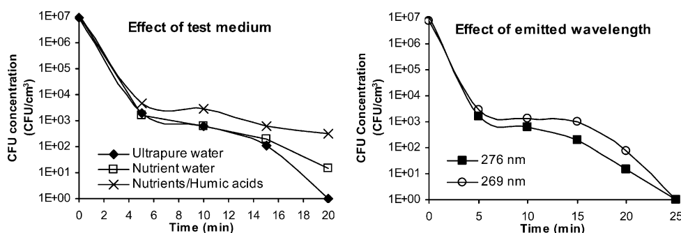
Fig. 1 Effect of test medium and emitted wavelength to E. coli destruction
